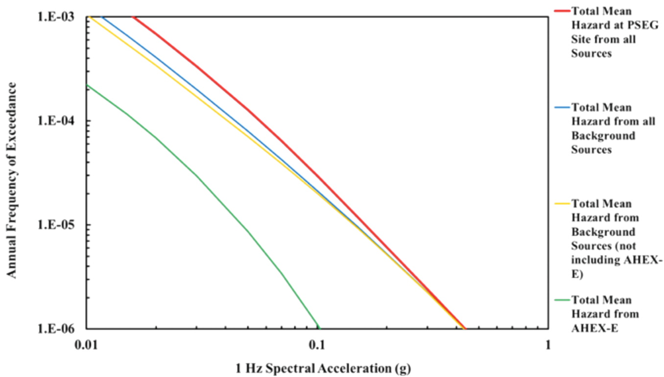
Contribution to 1 Hz Rock Total Mean Hazard at PSEG Site
