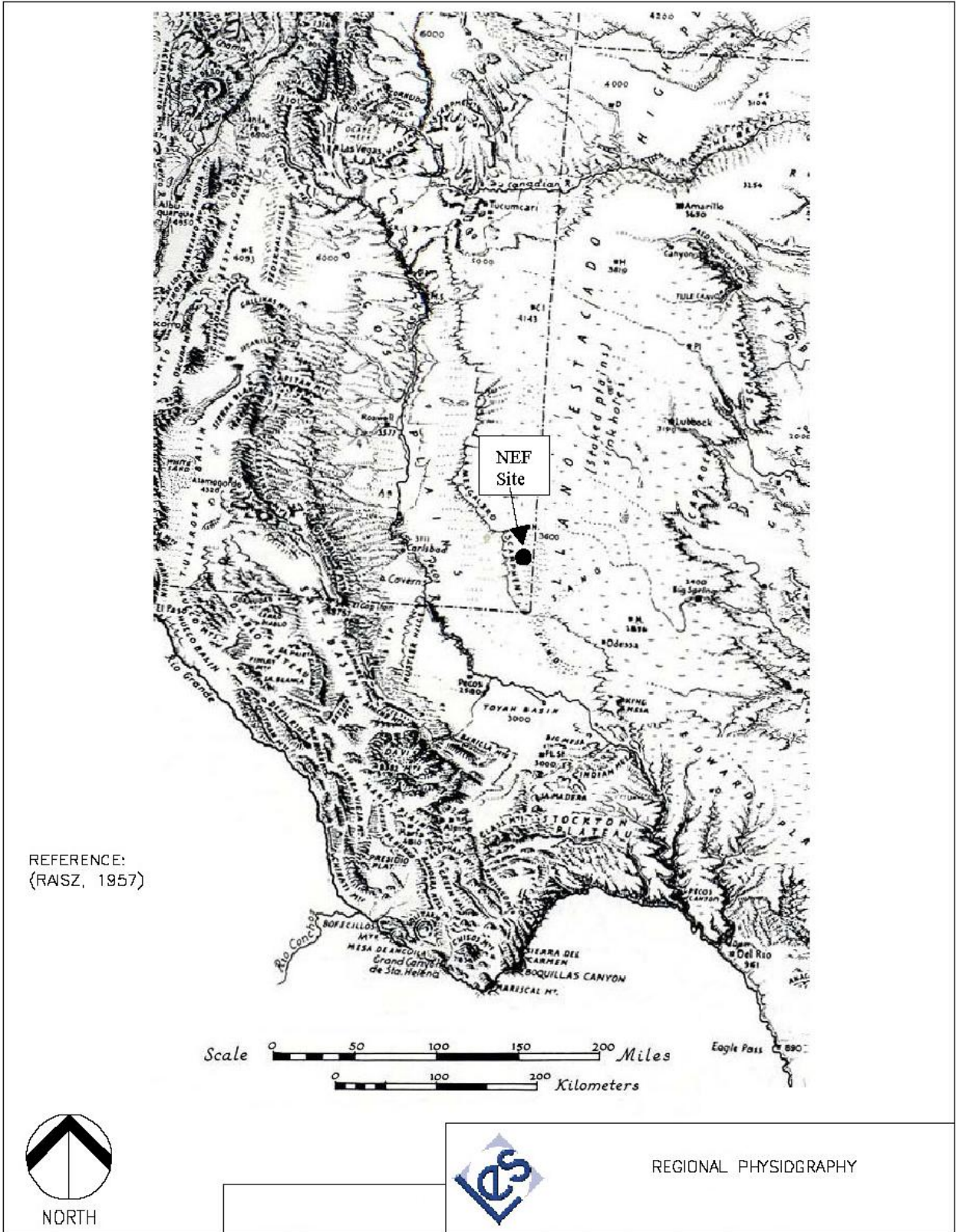
Figure 3.3-1 Regional Physiography
