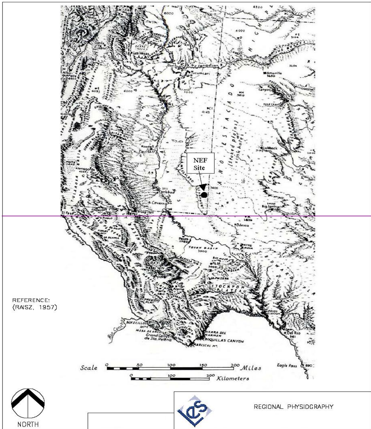
Figure 3.3-1—Regional Physiography
