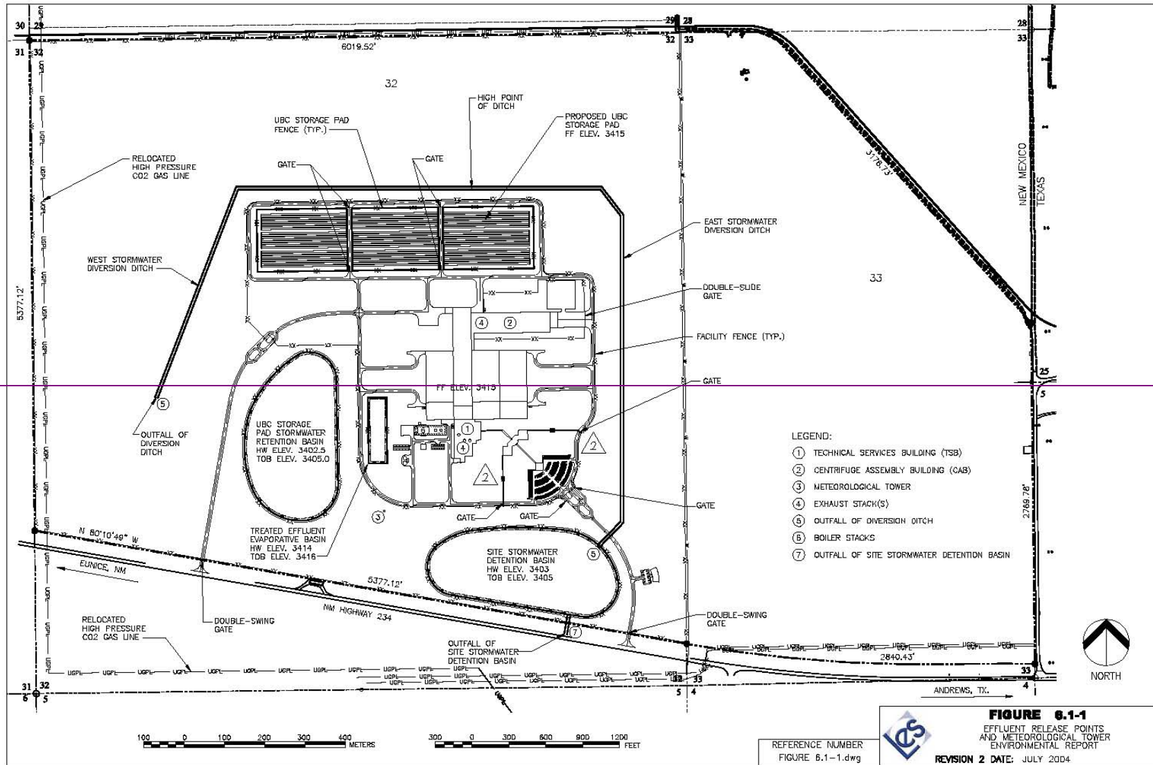
Figure 6.1-1 — Effluent Release Points and Meteorological Tower
