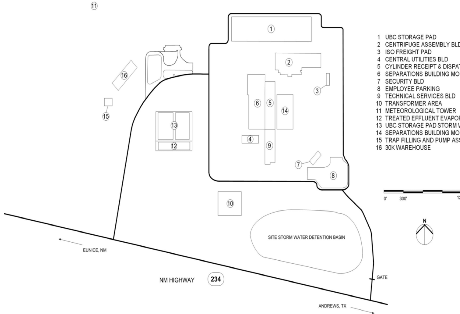
Figure 2.1-4_ NEF Buildings
