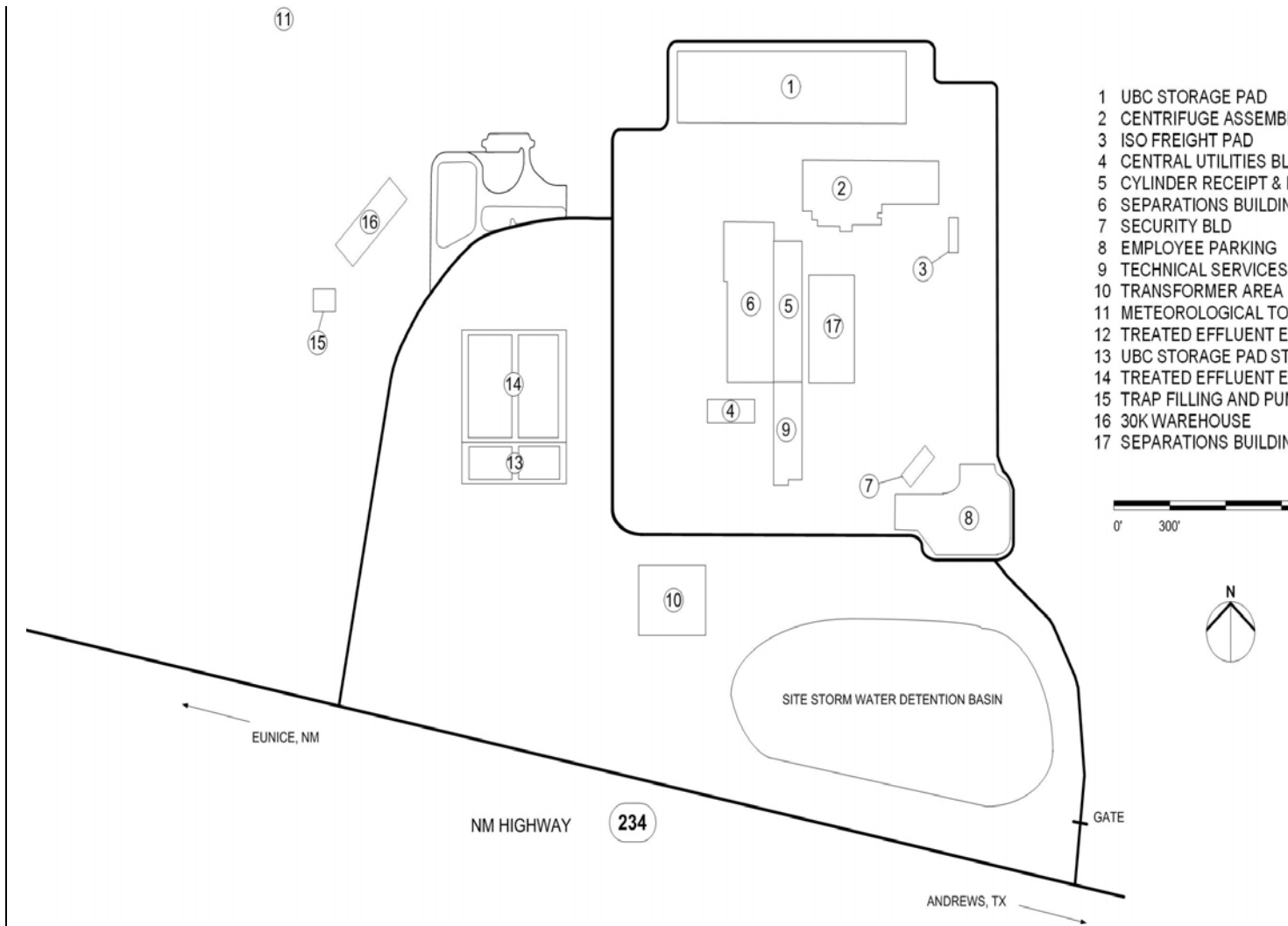
Figure 1.2-4 NEF Buildings
