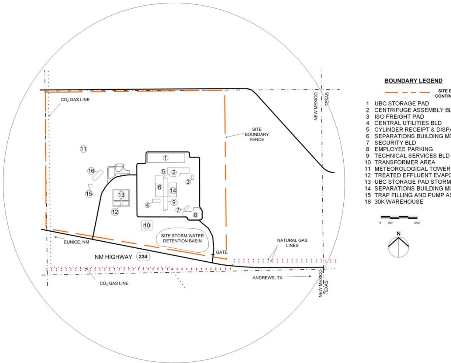
Figure 2.1-2 _Site Area and Facility Layout Map 1.6-Kilometer (1-Mile Radius)
