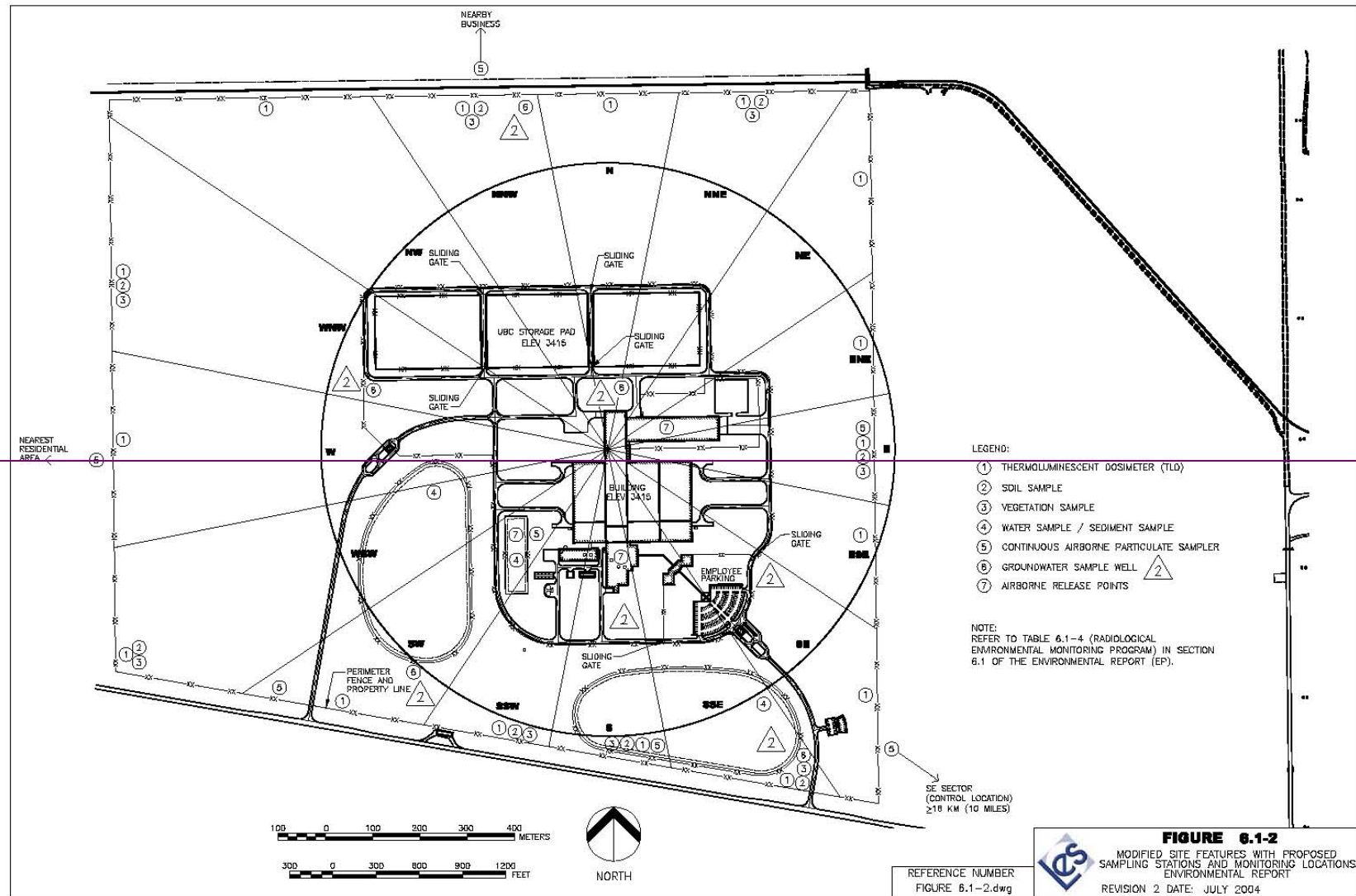
Figure 6.1-2—Modified Site Features With Proposed Sampling Stations and Monitoring Locations
