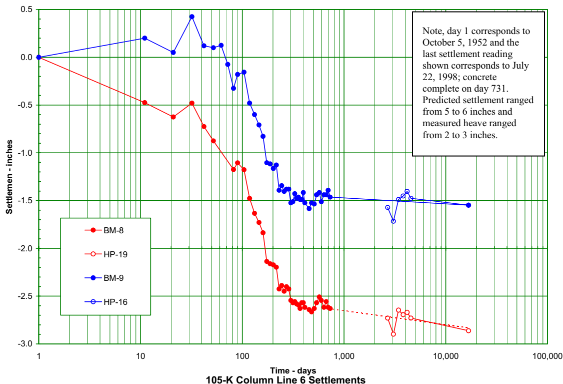
Figure 2; K-Area Settlement
