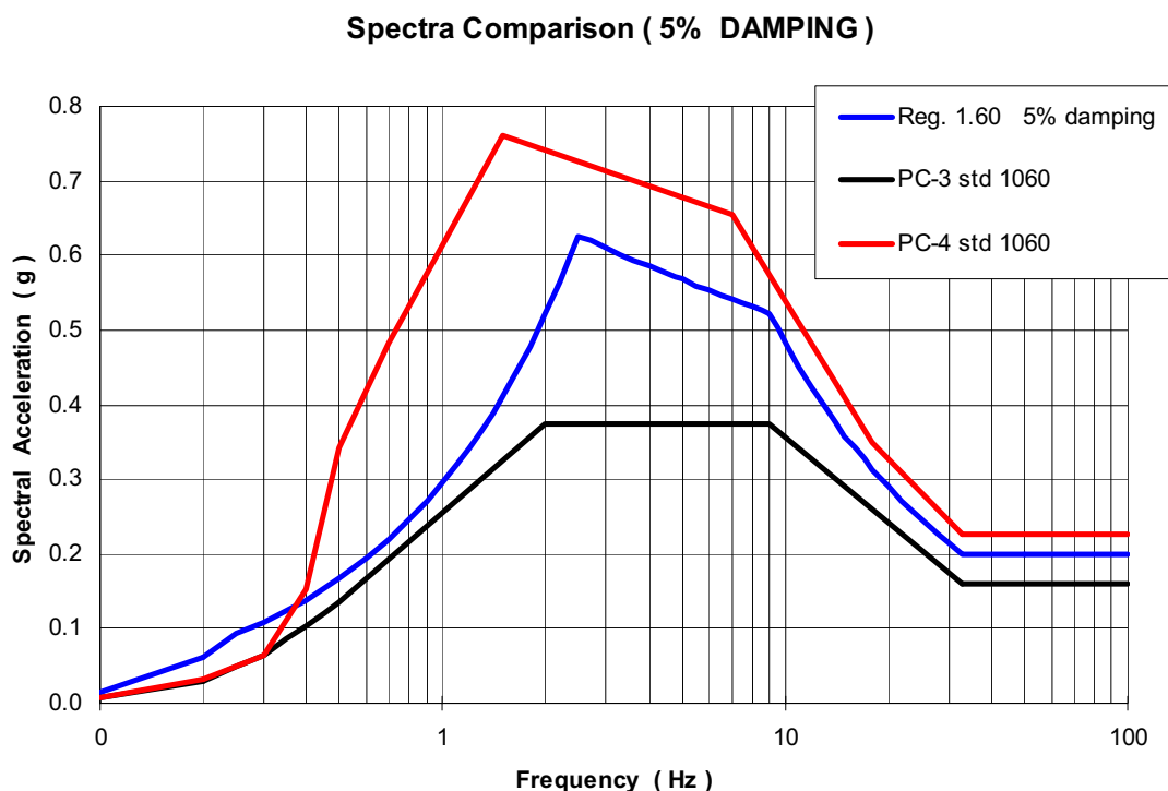
Figure 3; Response Spectra
