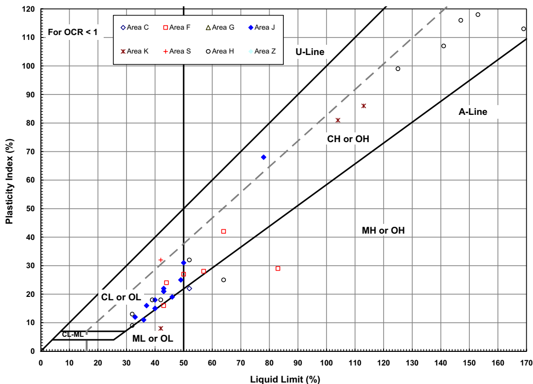
Figure 6; Comparison of Atterberg Limits
