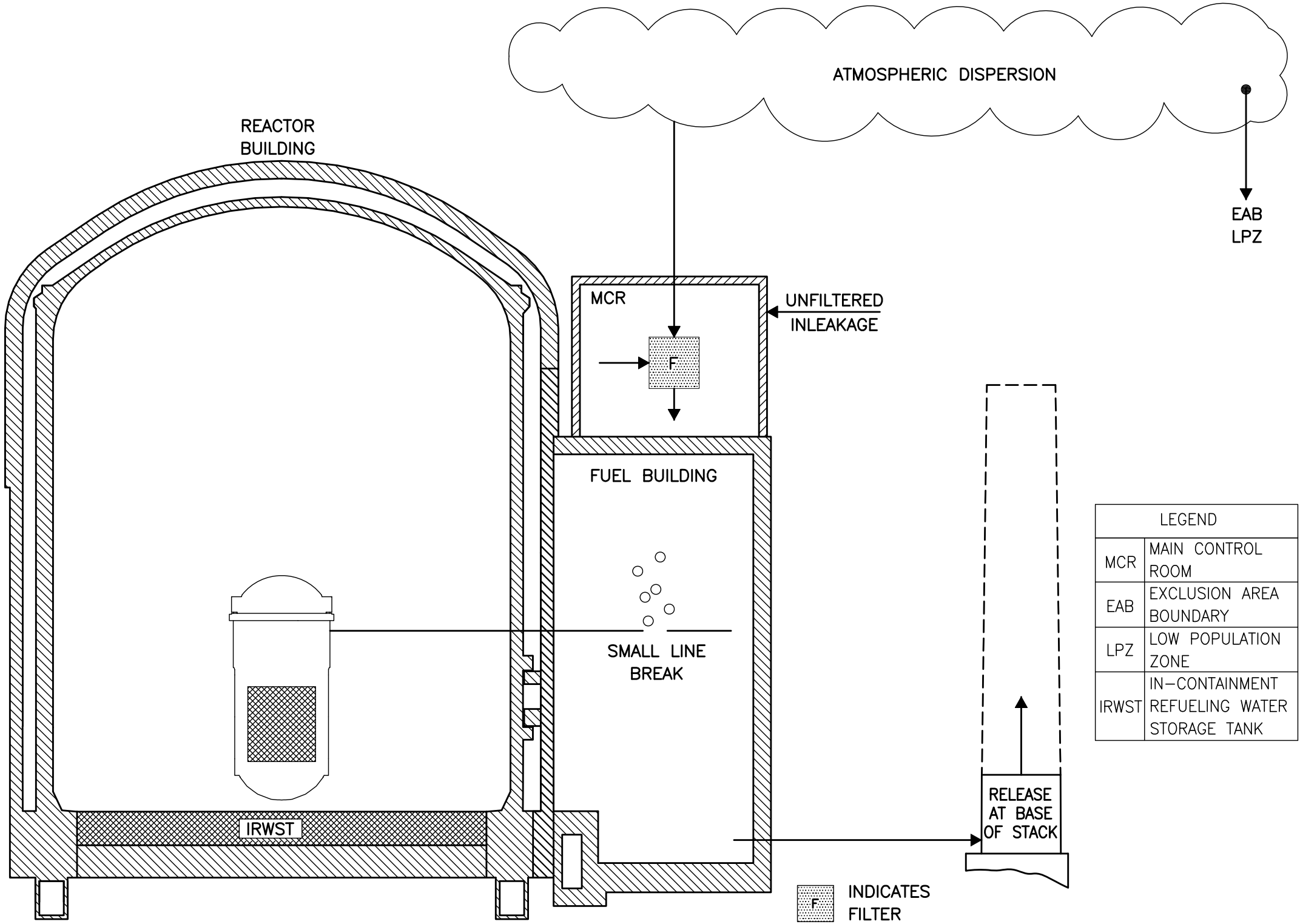
Figure 15.0-5—Small Line Break Accident Scenario
