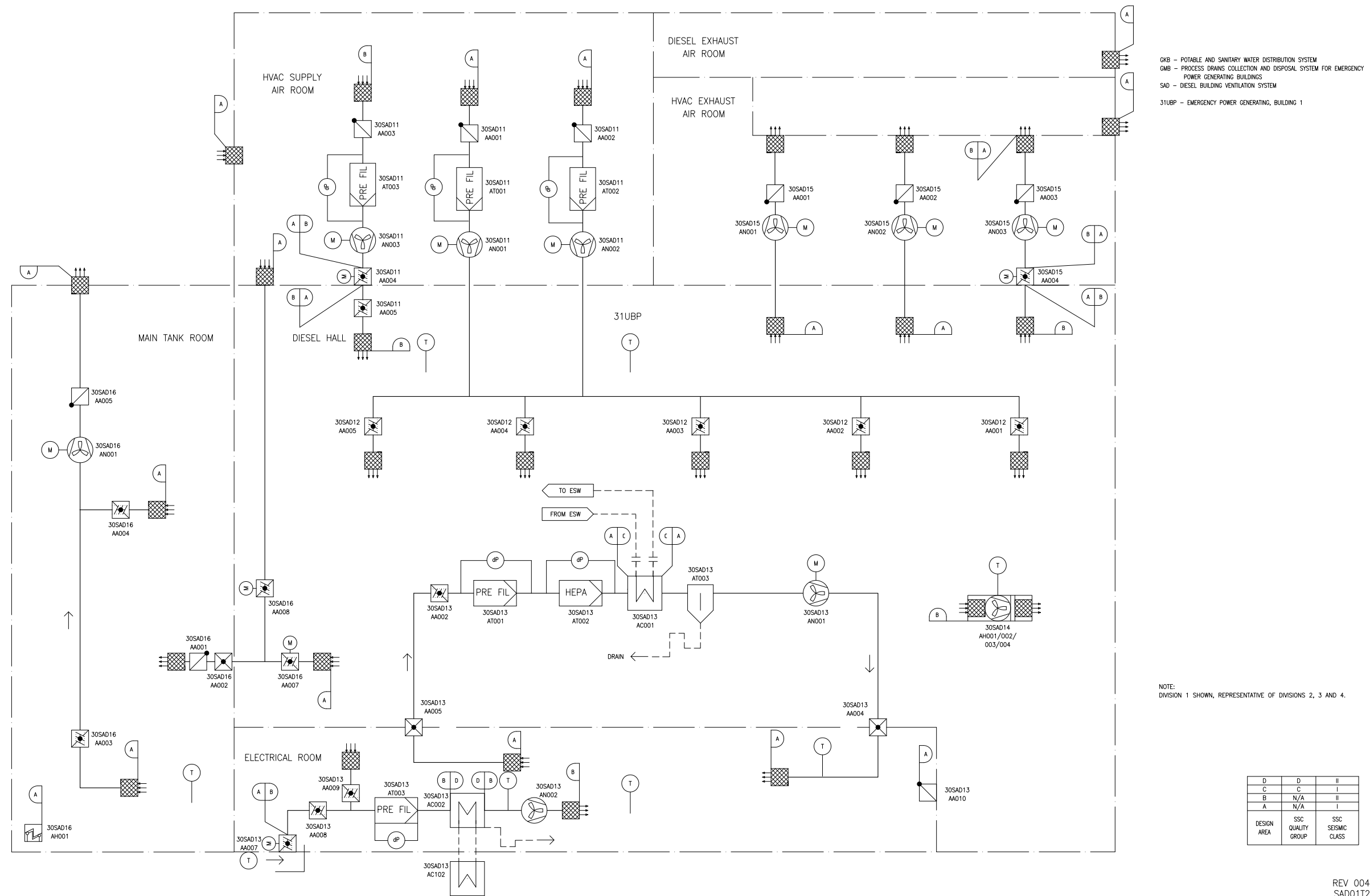
Figure 9.4.9-1—Emergency Power Generating Building Ventilation System
