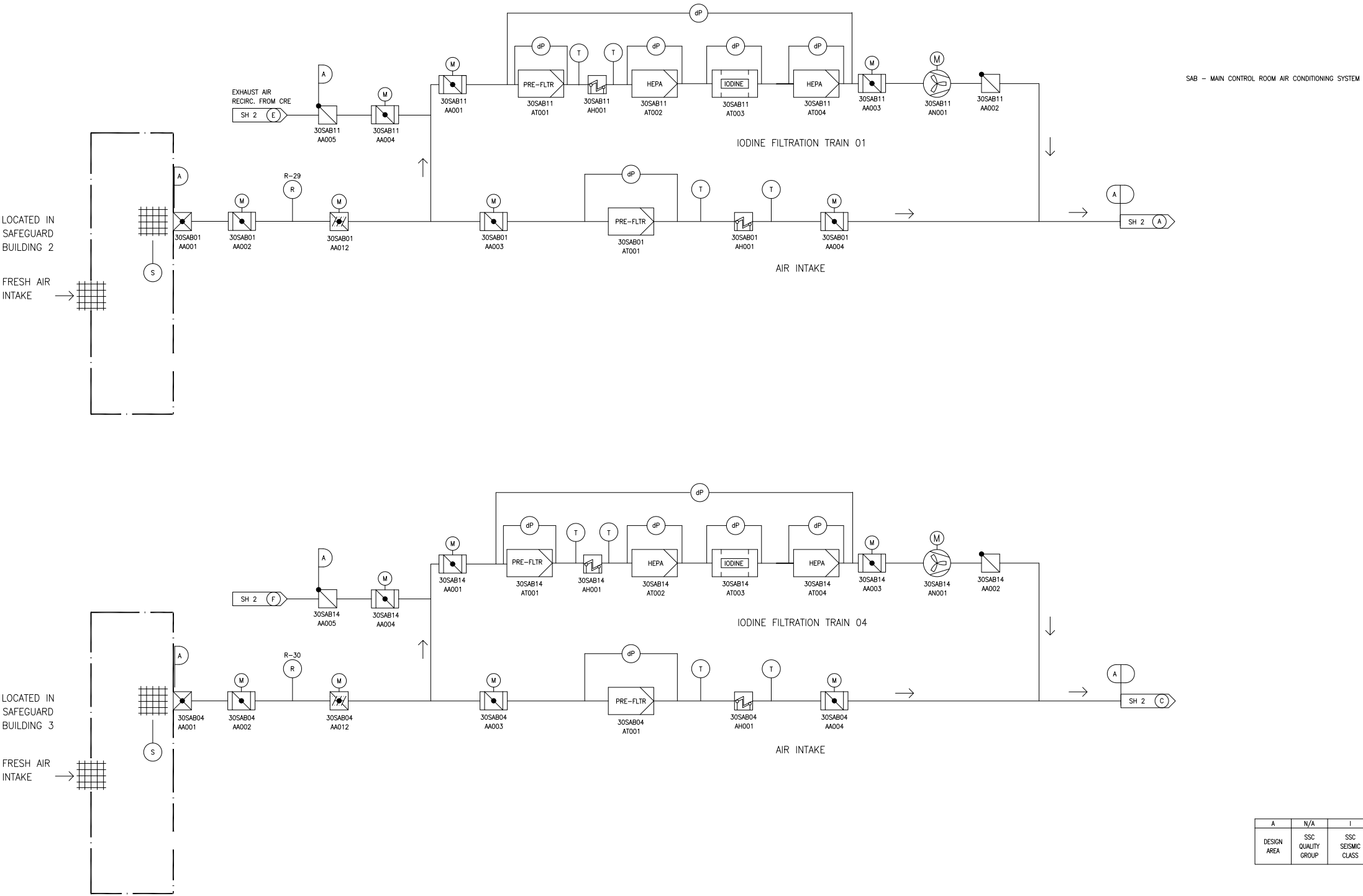
Figure 9.4.1-1—Control Room Air Intake and CREF (Iodine Filtration) Train Subsystem
