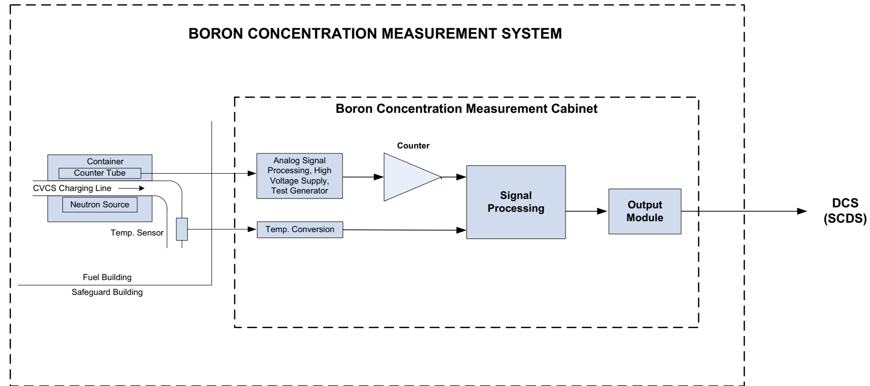
Figure 7.1-16—Boron Concentration Measurement System Arrangement
