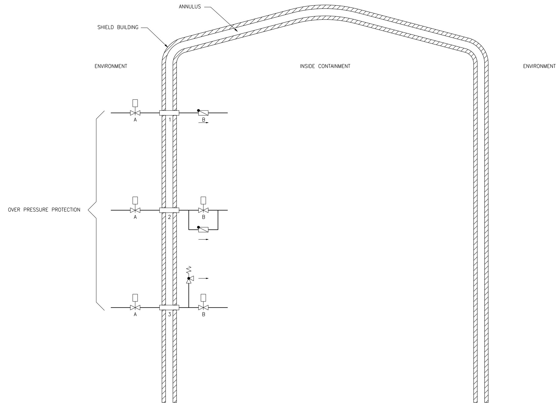
Figure 6.2.4-2—Containment Isolation Valve Arrangements for Overpressure Protection
