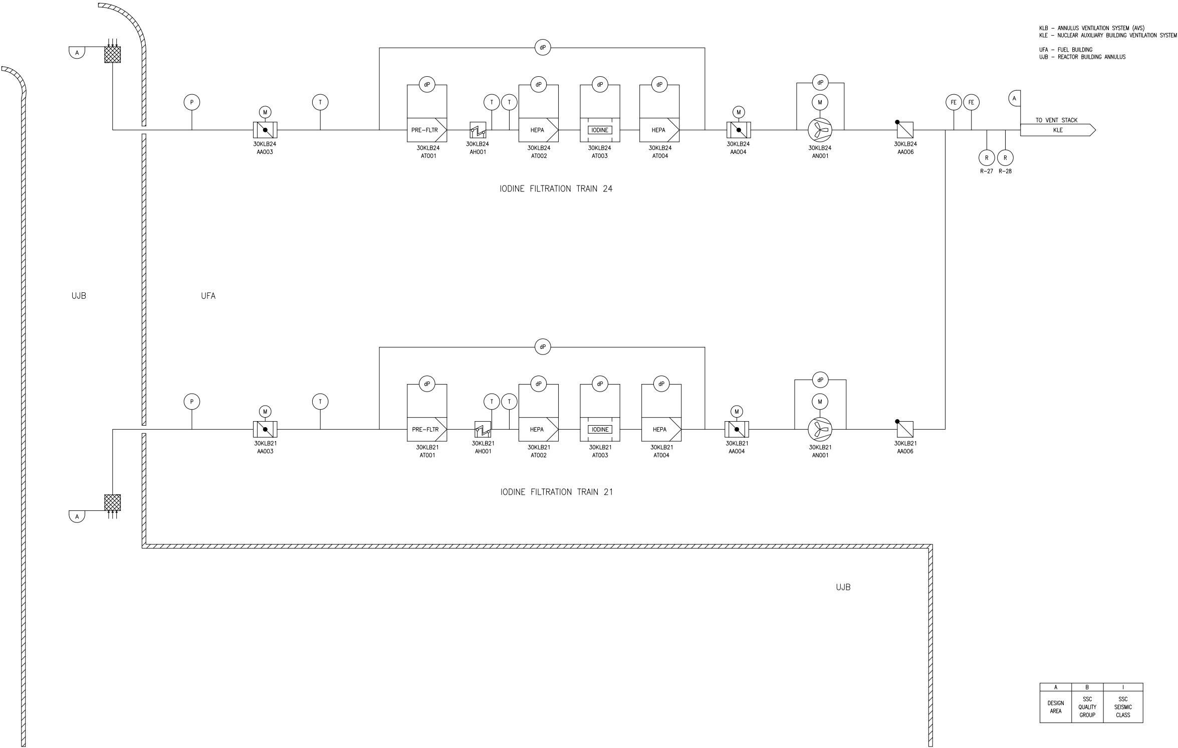
Figure 6.2.3-2—AVS Accident Trains
