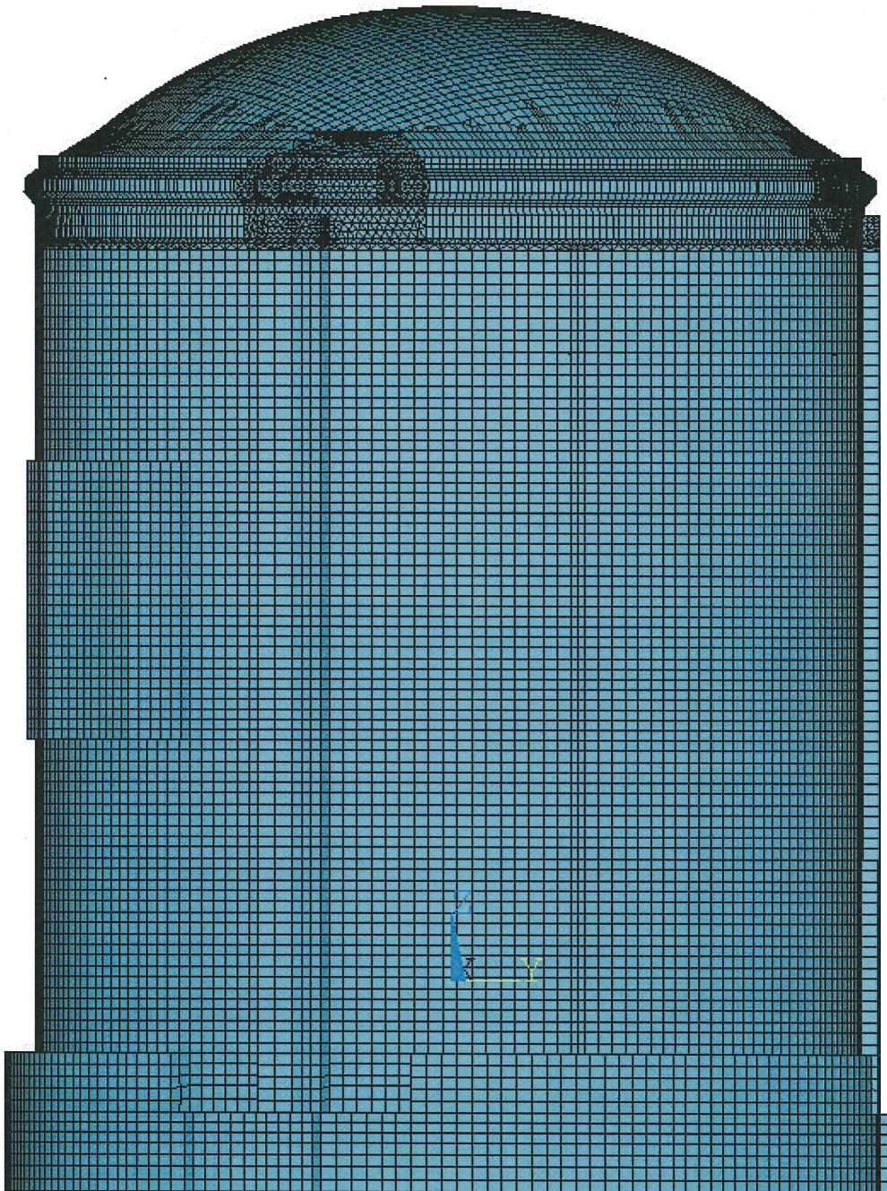
Figure 3E.1-15—Elevation View of the Entire RCB
