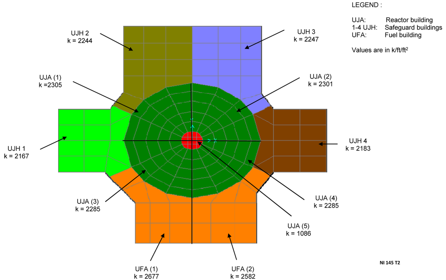
Figure 3.8-145—Foundation Modulus for High Frequency Soil Cases
