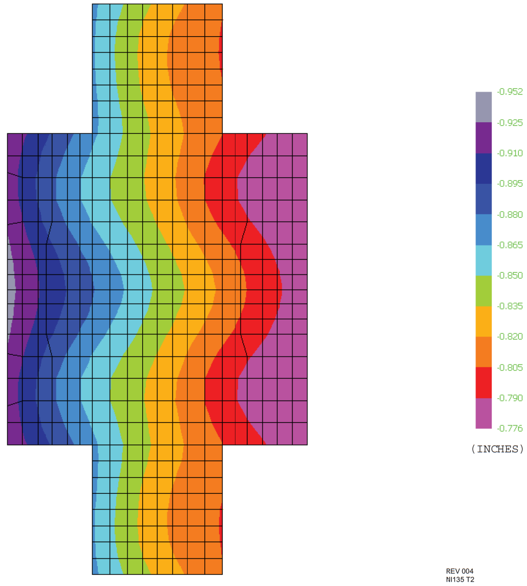
Figure 3.8-135—Total Differential Settlement, EPGB
