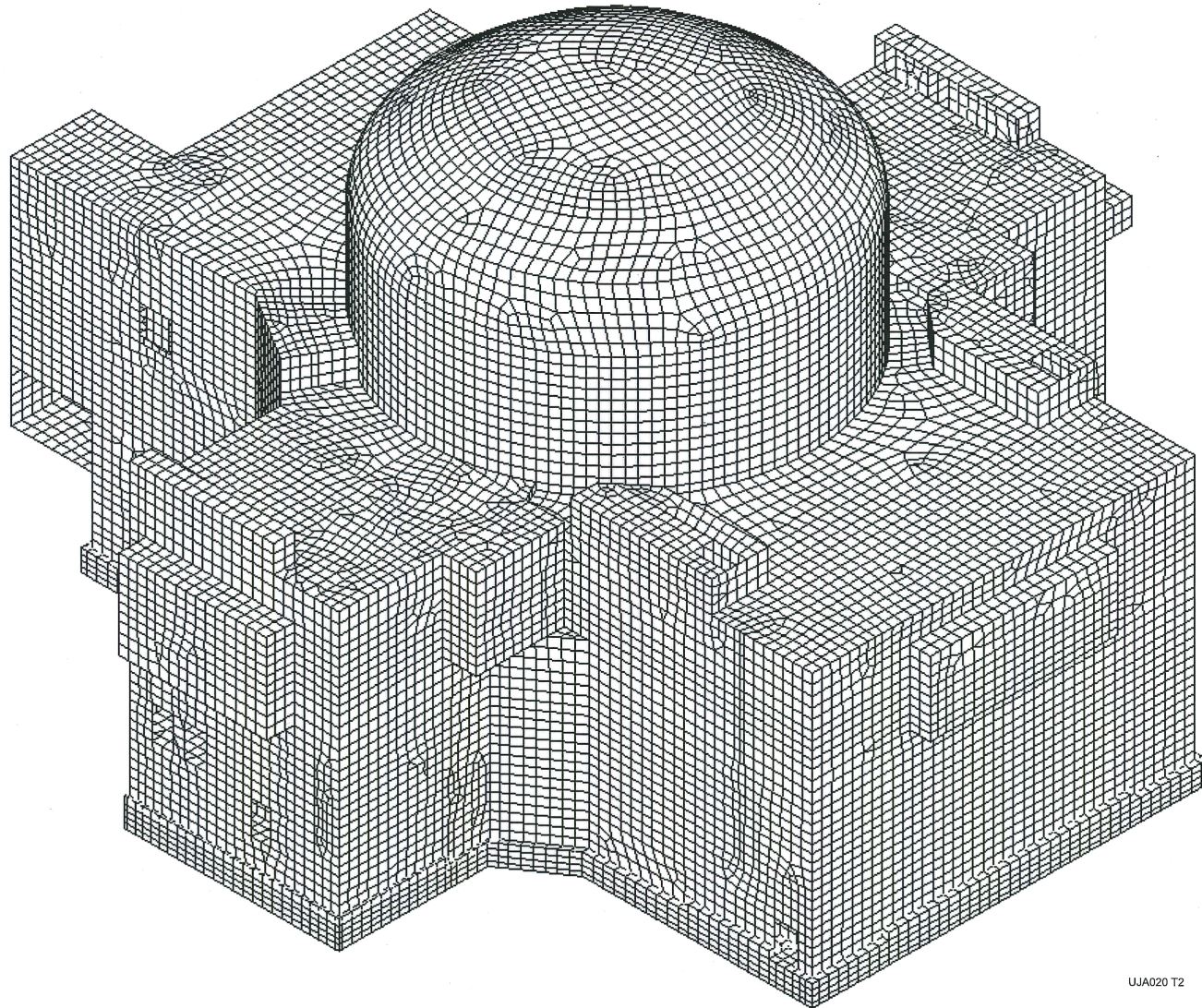
Figure 3.8-86—ANSYS Finite Element Model of Nuclear Island Common Basemat Structure - Outside View
