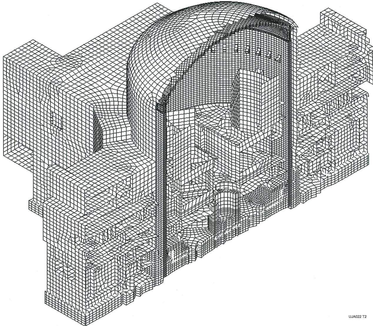
Figure 3.8-88—ANSYS Finite Element Model of Nuclear Island Common Basemat Structure - Section Through Safeguard Buildings 4 and 1
