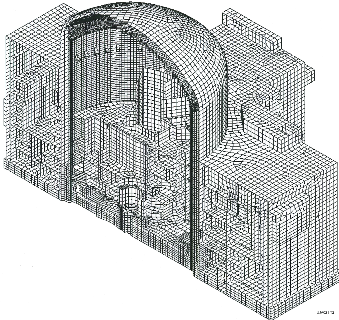
Figure 3.8-87—ANSYS Finite Element Model of Nuclear Island Common Basemat Structure - Section Through Fuel Building and Safeguard Building 2/3 Island
