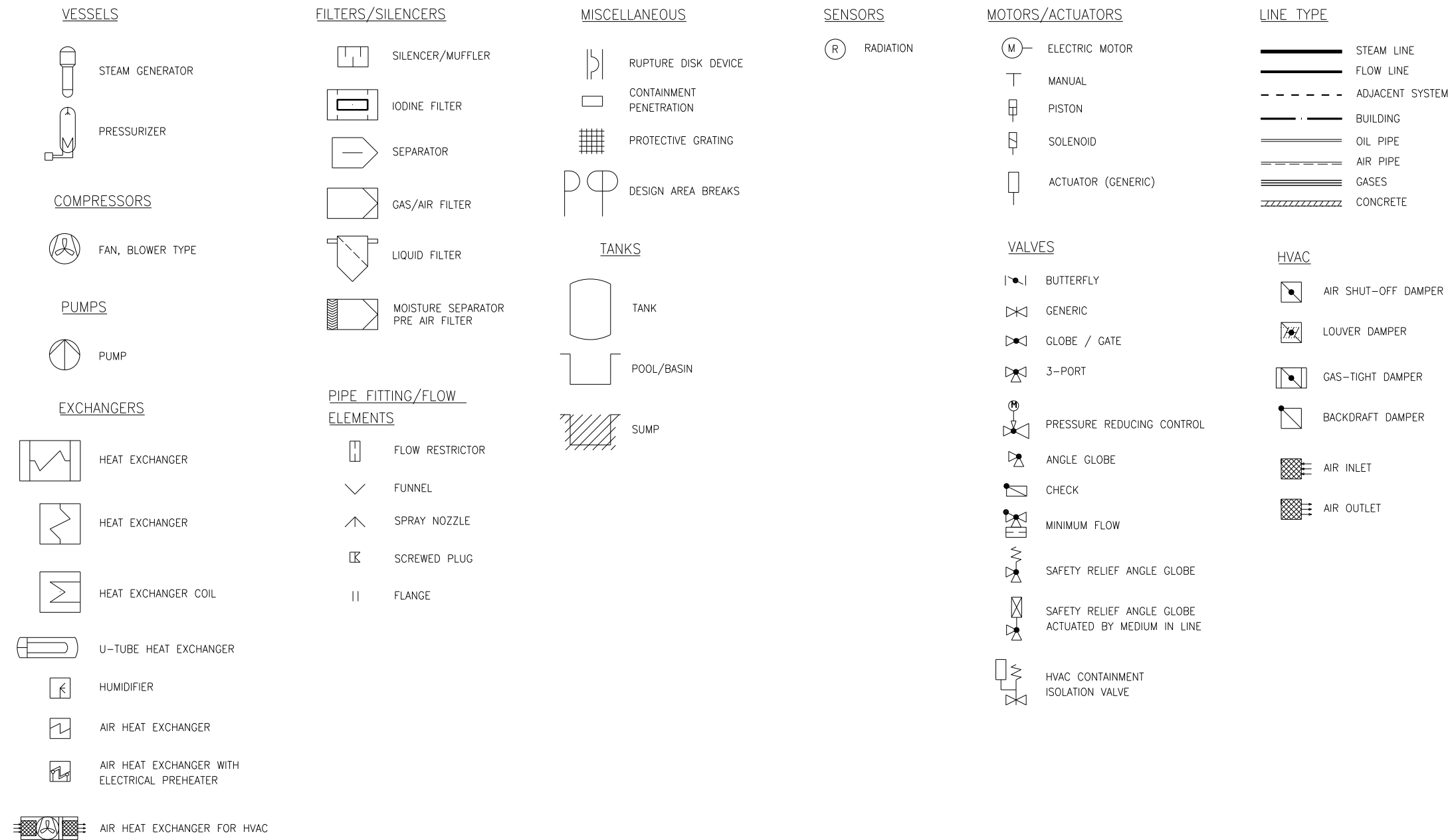
Figure 1.3-1—Functional Arrangement Symbol Legend
