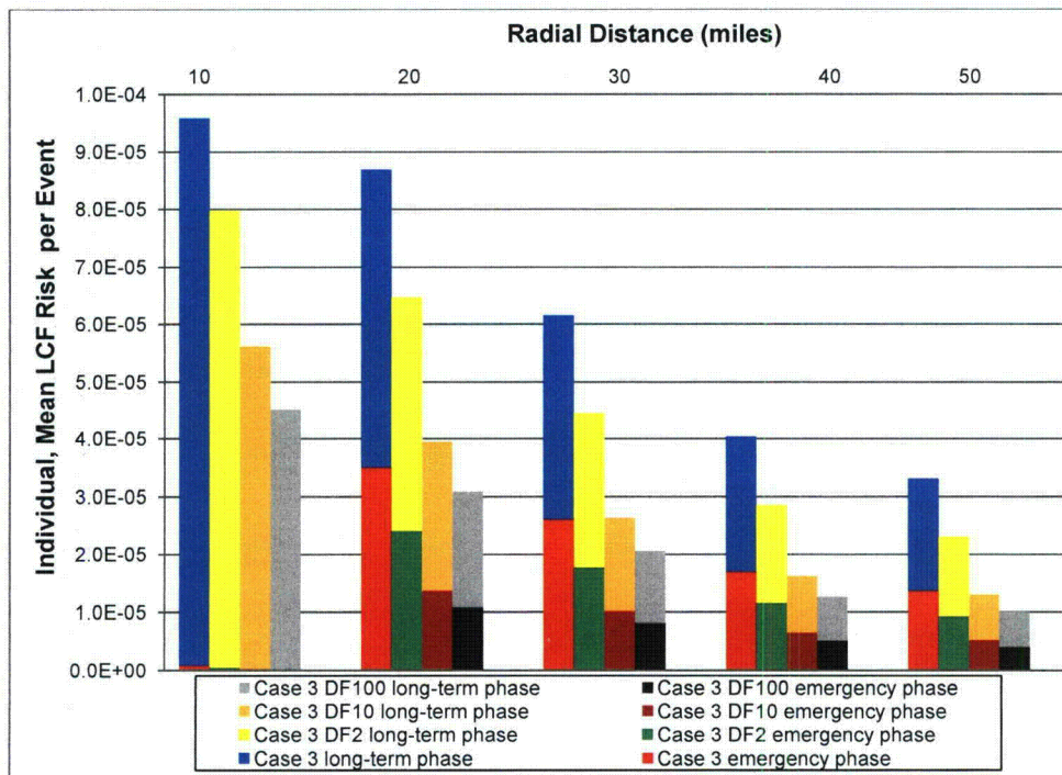
Figure 3 Case 3 individual, mean LCF risk per event for residents within a circular area at specified radial distances with specified decontamination factors
