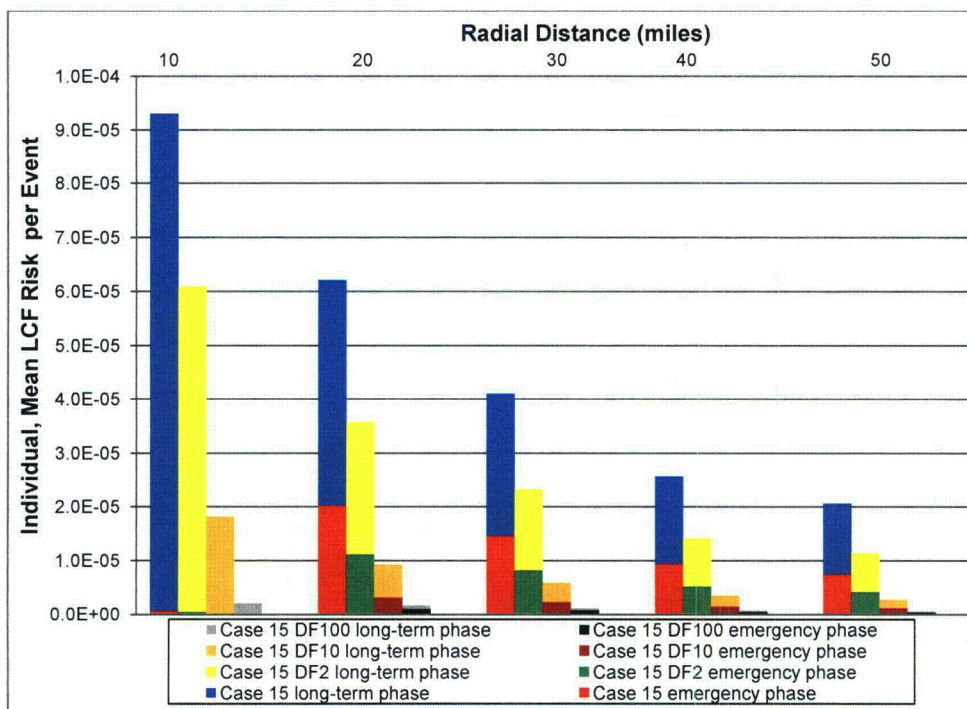
Figure 16 Case 15 individual, mean LCF risk per event for residents within a circular area at specified radial distances with specified decontamination factors
