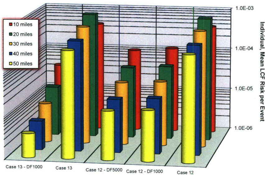
Figure 9 Individual, mean LCF risk per event for residents within a circular area at specified radial distances for the Drywell Venting Cases
