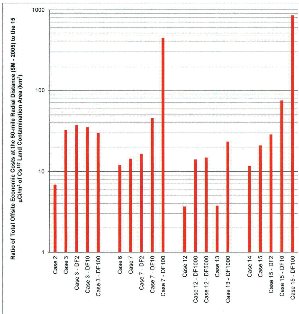
Figure 20 Ratio of mean, total offsite economic costs per event within a circular area of 50-mile radius to the land contamination area exceeding 15 \mu\text{Ci}/\text{m}^2 of Cs-137 for all the cases considered
