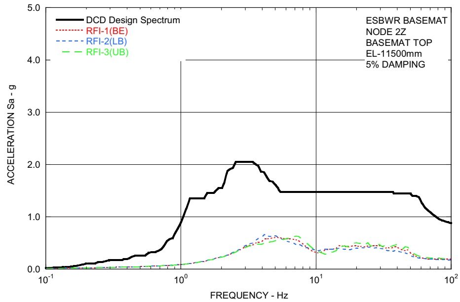
Figure 3.7.2-209f Comparison of Floor Response Spectra - RB/FB Basemat in Z-Direction [EF3 SUP 3.7-4]
