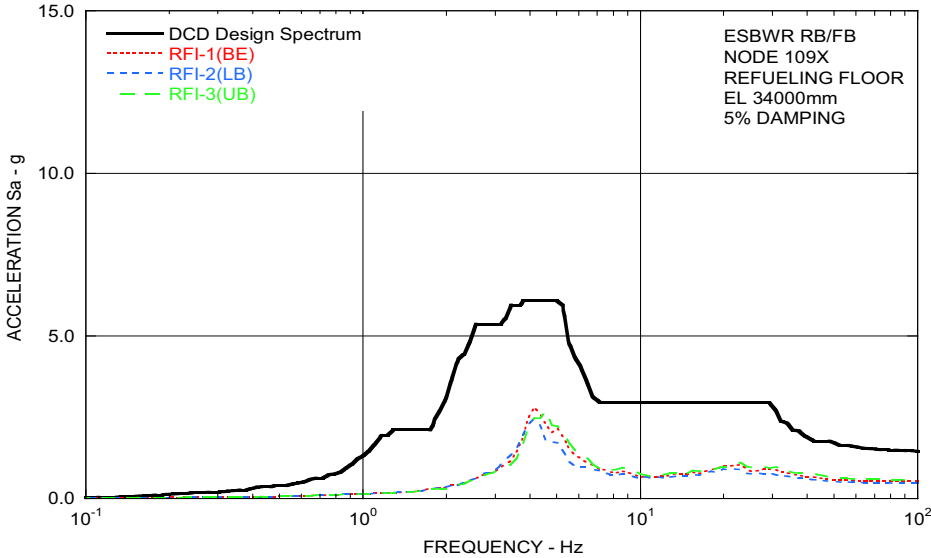
Figure 3.7.2-207a Comparison of Floor Response Spectra - RB/FB Refueling Floor in X-Direction [EF3 SUP 3.7-4]
