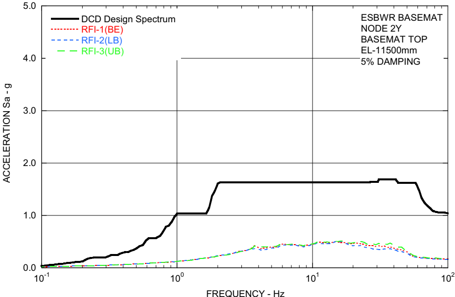
Figure 3.7.2-208f Comparison of Floor Response Spectra - RB/FB Basemat in Y-Direction [EF3 SUP 3.7-4]
