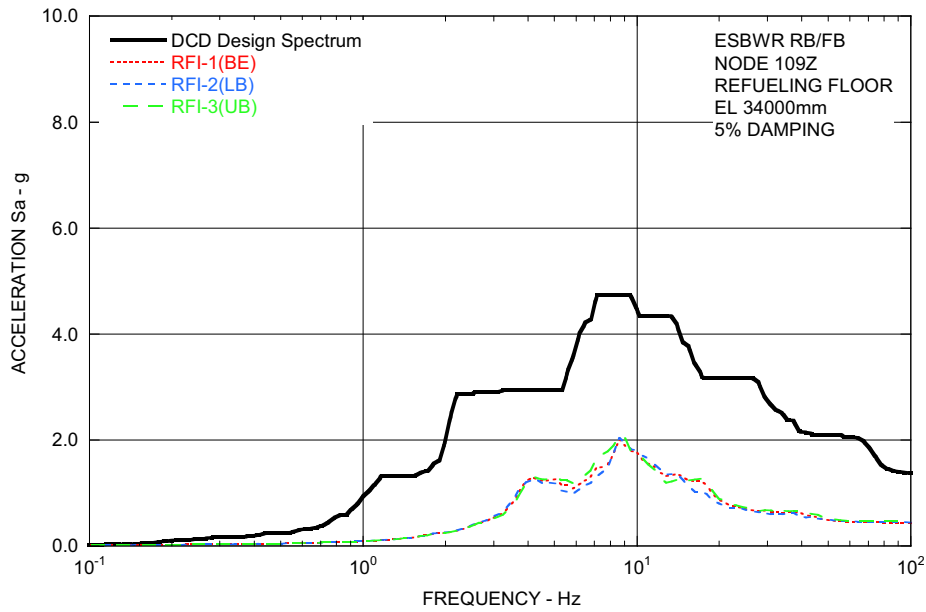
Figure 3.7.2-209a Comparison of Floor Response Spectra - RB/FB Refueling Floor in Z-Direction [EF3 SUP 3.7-4]
