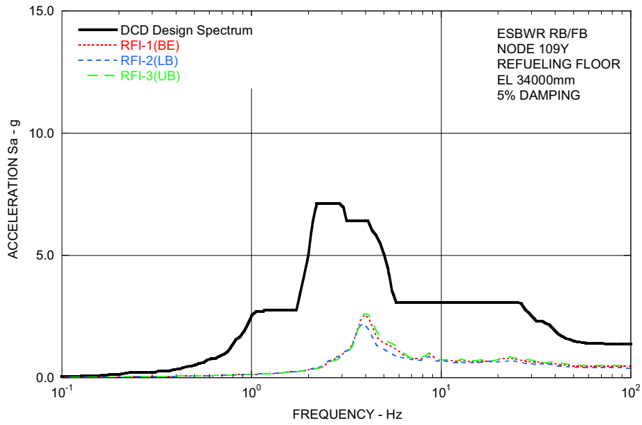
Figure 3.7.2-208a Comparison of Floor Response Spectra - RB/FB Refueling Floor in Y-Direction [EF3 SUP 3.7-4]
