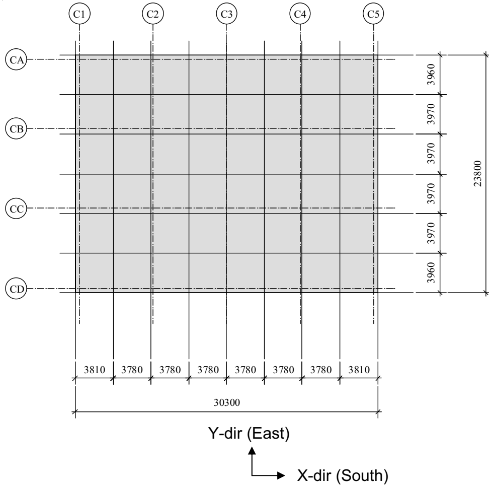
Figure 3.7.2-204 SASSI2000 Plate Elements for CB Basemat [EF3 SUP 3.7-4]
