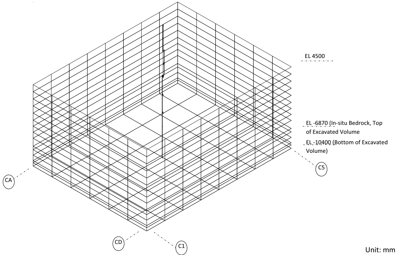
Figure 3.7.2-206 Overview of CB SASSI2000 SSI Model
