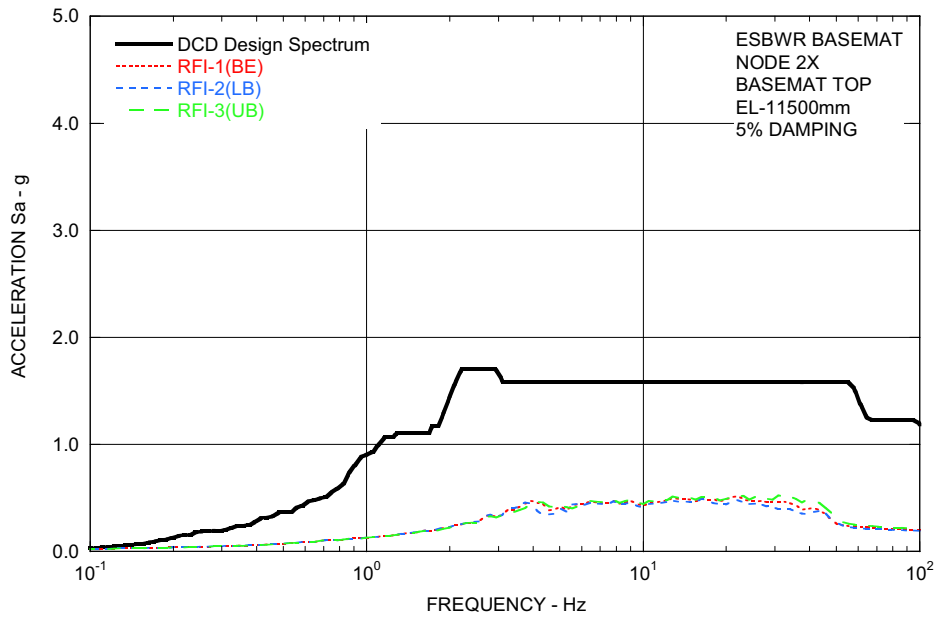
Figure 3.7.2-207f Comparison of Floor Response Spectra - RB/FB Basemat in X-Direction [EF3 SUP 3.7-4]
