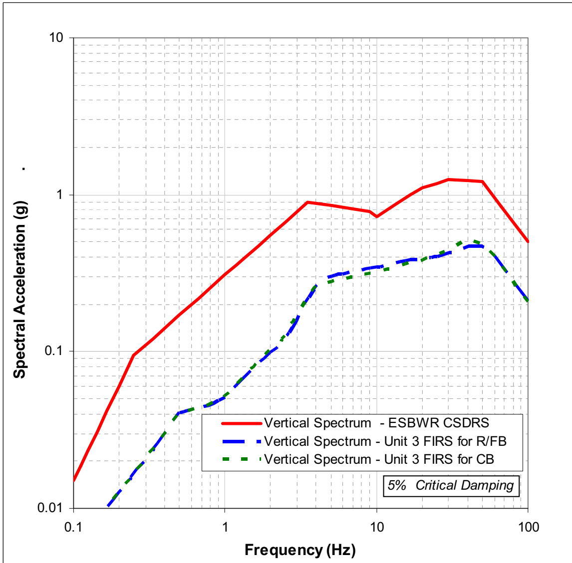
Figure 2.0-202 Comparison of Vertical CSDRS with the Unit 3 FIRS for the RB/FB and CB [EF3 COL 2.0-1-A]
