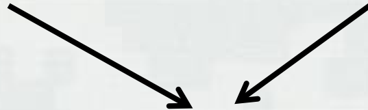
Frequentist
