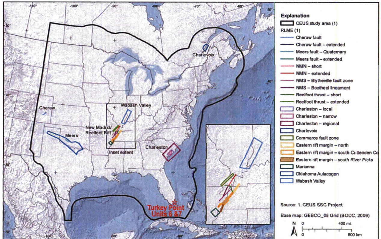
Figure 2.5.2-282 RLME Sources in the CEUS SSC Model
