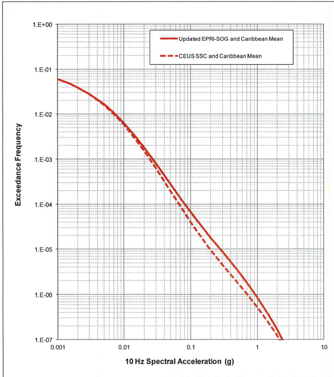
Figure 8: CEUS Hard Rock Hazard Results for 10 Hz Spectral Acceleration
