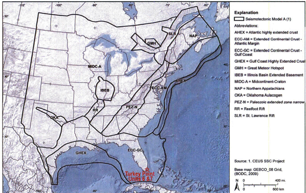
Figure 1: Seismotectonic Source Zones
