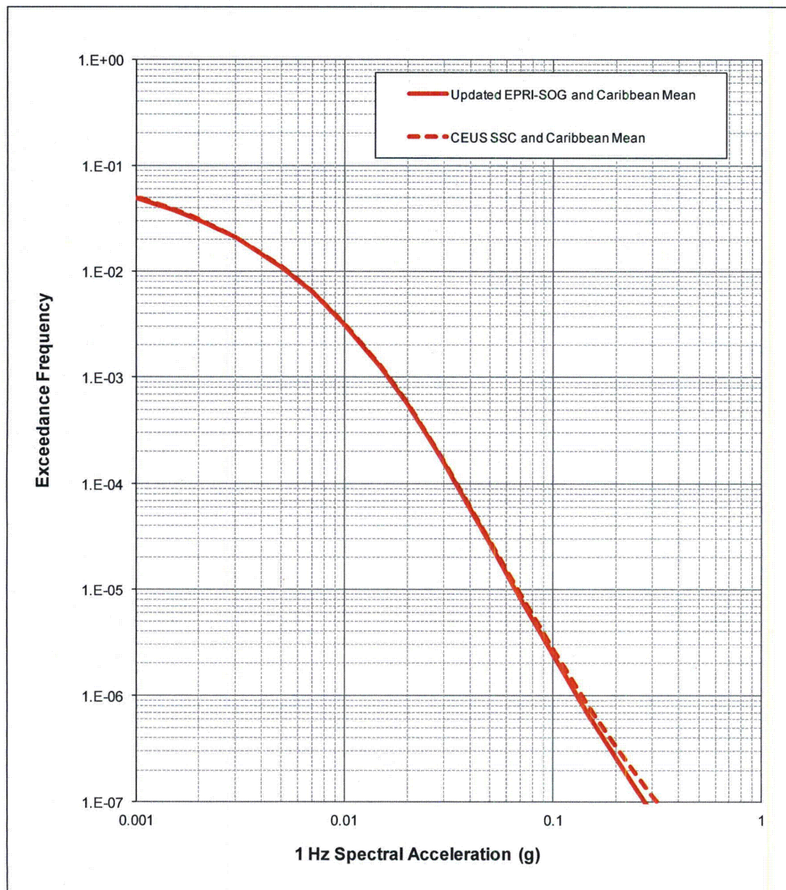
Figure 5: CEUS Hard Rock Hazard Results for 1 Hz Spectral Acceleration
