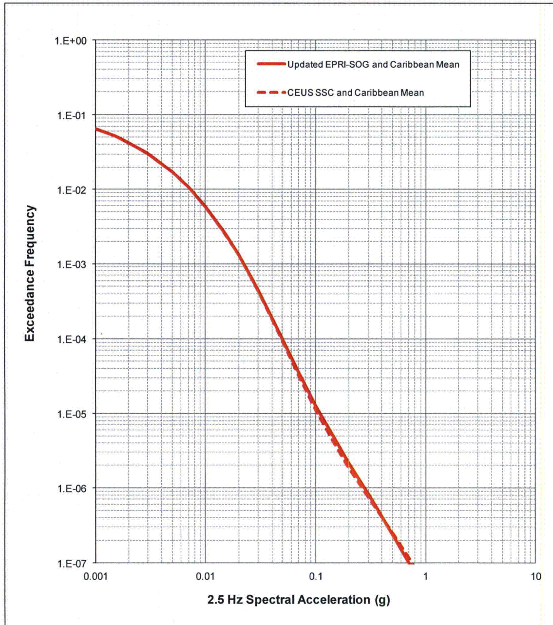
Figure 6: CEUS Hard Rock Hazard Results for 2.5 Hz Spectral Acceleration
