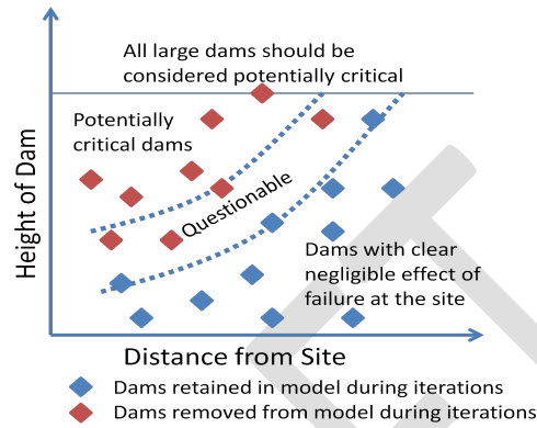
Figure 4 – Example Illustration of Dam Failure Evaluation Screening Approach (Method 4)
