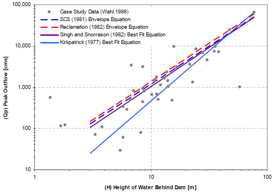
Figure 8 - Peak Outflow as a Function of Height of Water behind Dam (Pierce 2010)
