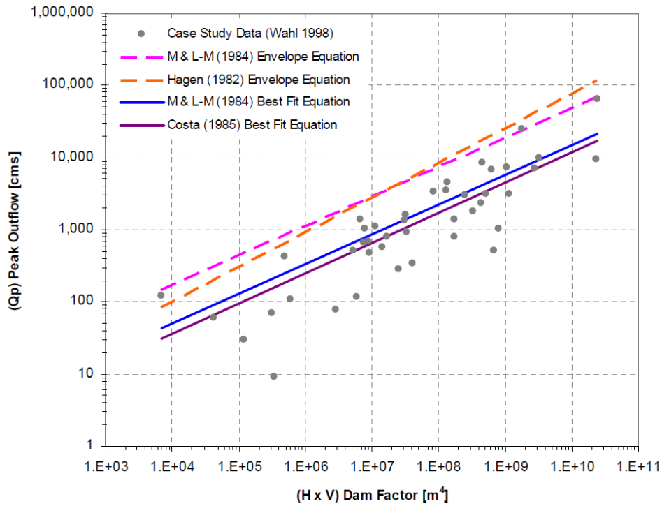
Figure 9 - Peak Outflow as a Function of Dam Factor (Pierce 2010)
