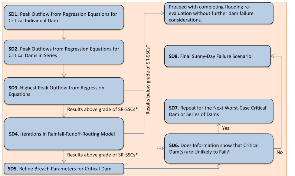
Figure 7 - Approach to Sunny-Day Failure Evaluation
