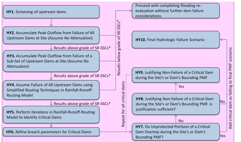
Figure 5 - Approach to Hydrologic Failure Evaluation
