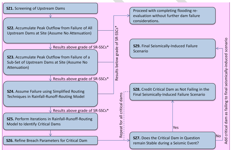
Figure 6 - Approach to Seismically-Induced Failure Evaluation
