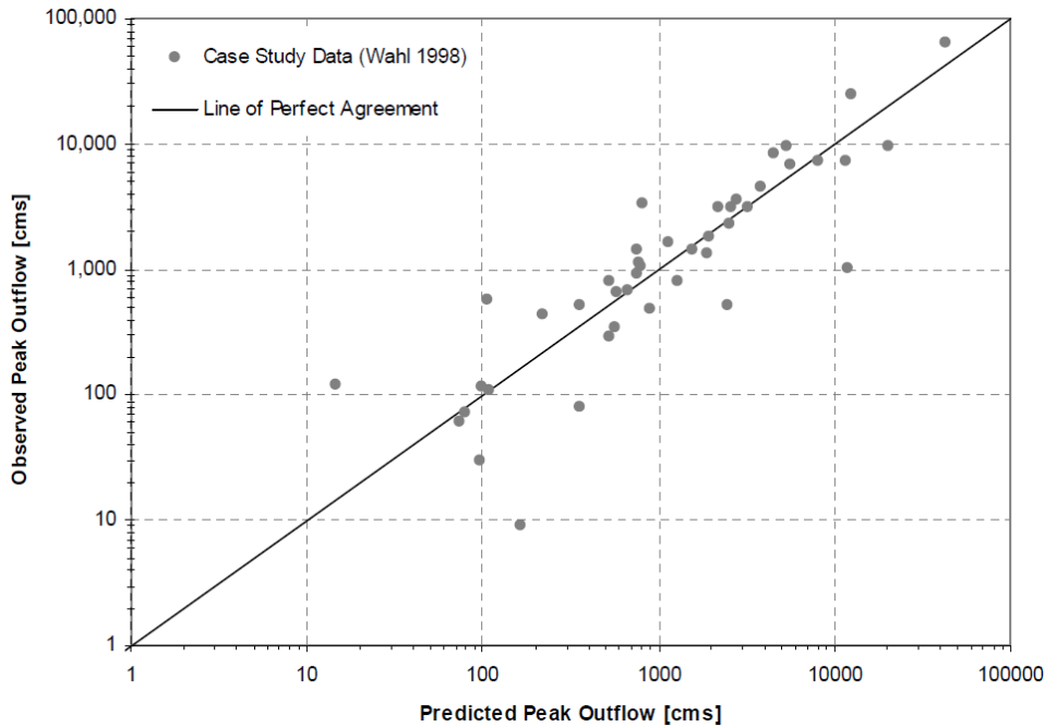
Figure 10 - Observed and Predicted Peak Outflow using Froehlich (1995a) Relationship (Pierce 2010)
