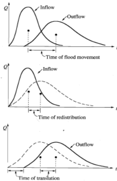
Figure 1 – Hydrograph Attenuation and Redistribution
