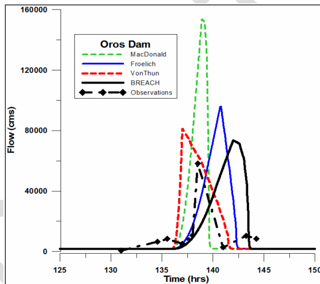
Figure 11 - Breach Hydrographs for Oros Dam (Gee, 2008)
