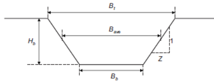
Figure 12 - Geometric Parameters of an Idealized Dam Breach (Xu and Zhang, 2009)
