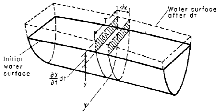
Figure 2 – Definition Sketch for St. Venant Equation
