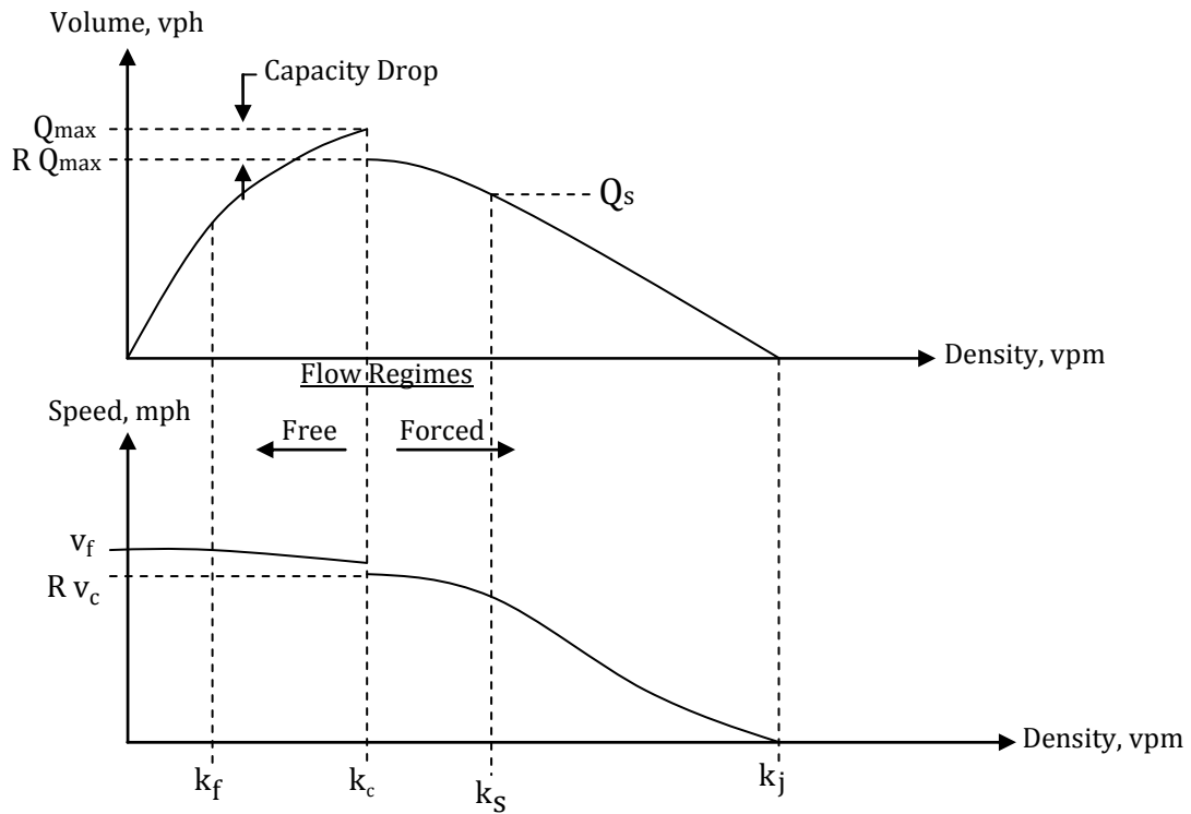
Figure C-2. Fundamental Diagrams
