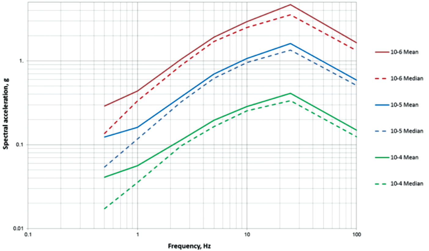
PSEG Site Mean and Median Rock UHRS for 10^{-4} , 10^{-5} , and 10^{-6} AFE
