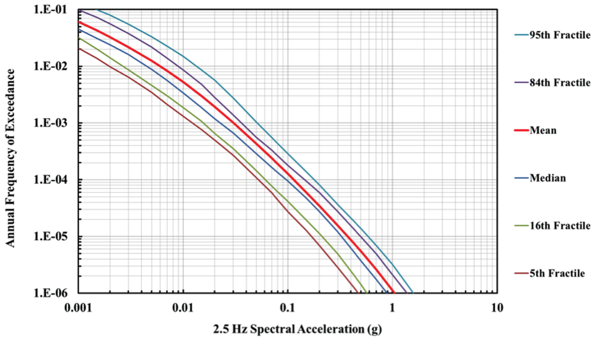
2.5 Hz Rock Total Mean and Median Hazard and Select Fractiles at PSEG Site
