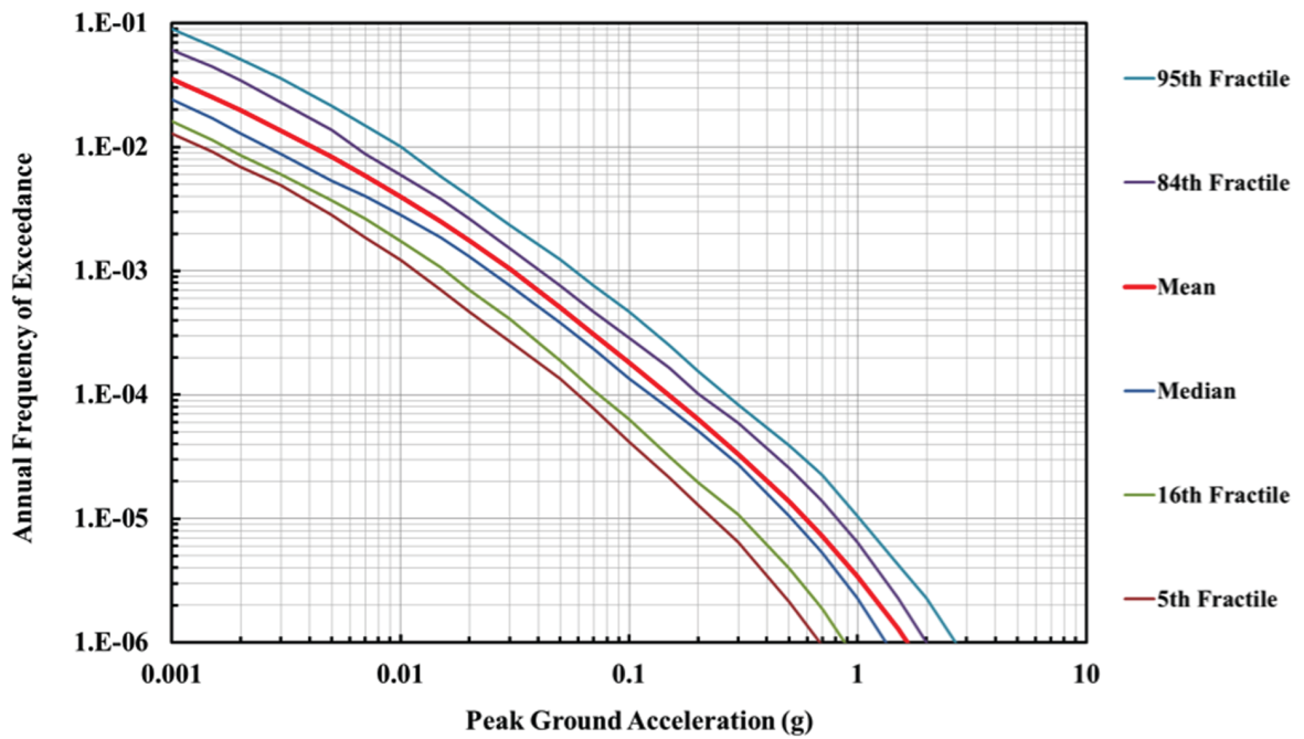
PGA Rock Total Mean and Median Hazard and Select Fractiles at PSEG Site
