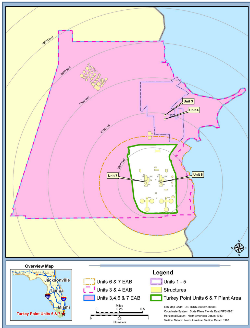
FIGURE 4.1-2 Exclusion Area Boundary
