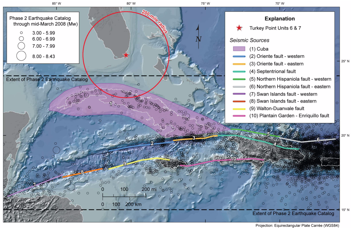
Cuba and Northern Caribbean Seismic Source Model Sources
