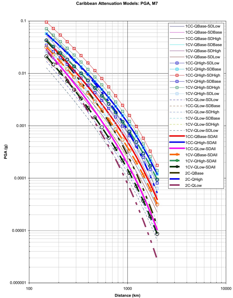
Figure 2.5.2-255 Comparison of PGA Attenuation Curves for the Cuba and Caribbean Region for a Magnitude Mw 7 Earthquake
