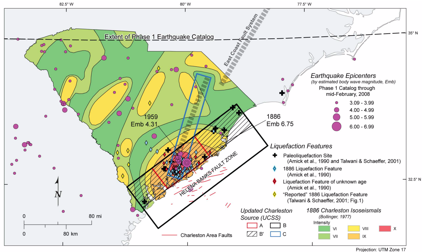
Updated Charleston Seismic Source (UCSS) Model Sources
