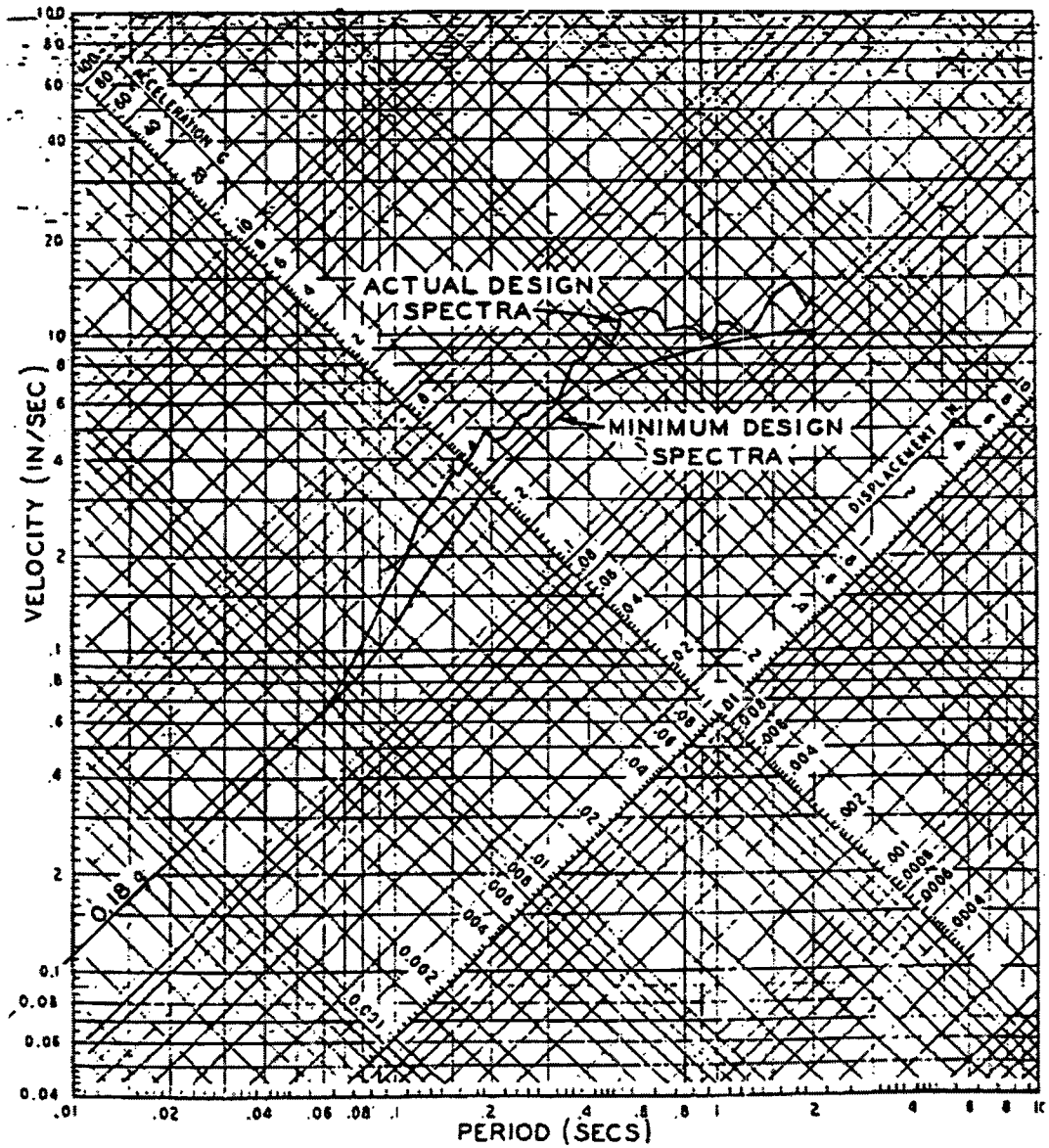
Figure 1 – Comparison of Response Spectra for Safe Shutdown Earthquake, 5% damping
