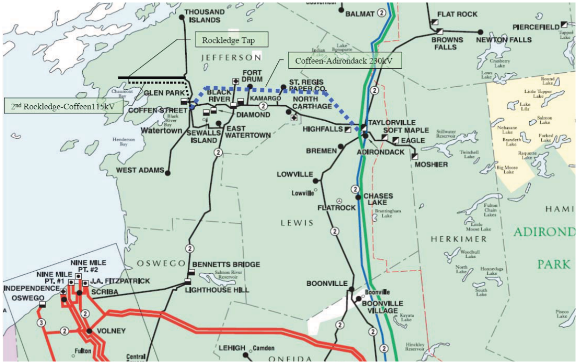
Figure 5.74: Transmission Map with 230kV Upgrade (dotted line)
