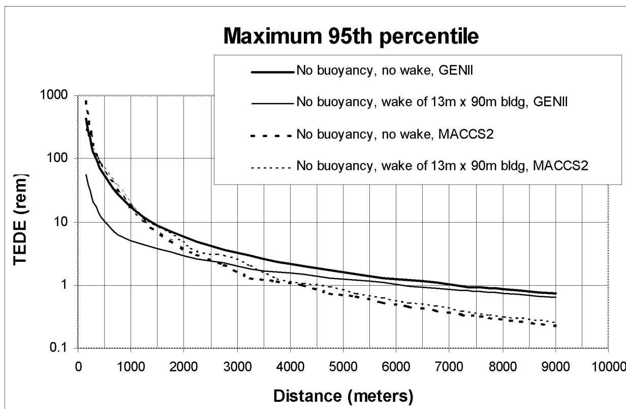
Figure 7-5. Comparison of MACCS2 with GENII for results at 95 th percentile TEDE. Note: GENII produces maximum sector 95 th percentile results whereas MACCS2 results are 95 th direction-independent. GENII results are calculated for two cases only: (1) base case (no lofting, no wake) and (2) building wake without lofting. Sensible heat impact differences from a fire condition were not examined because GENII cannot treat this phenomenon.
