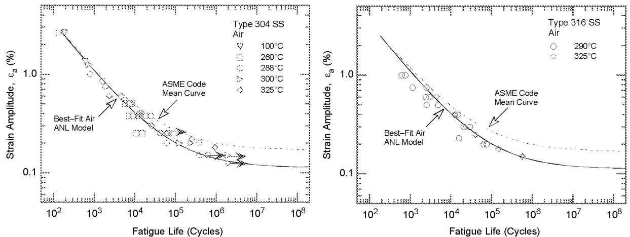
Figure 32. Influence of temperature on fatigue life of Types 304 and 316 stainless steel in air (Ref. 38, JNUFAD database).
