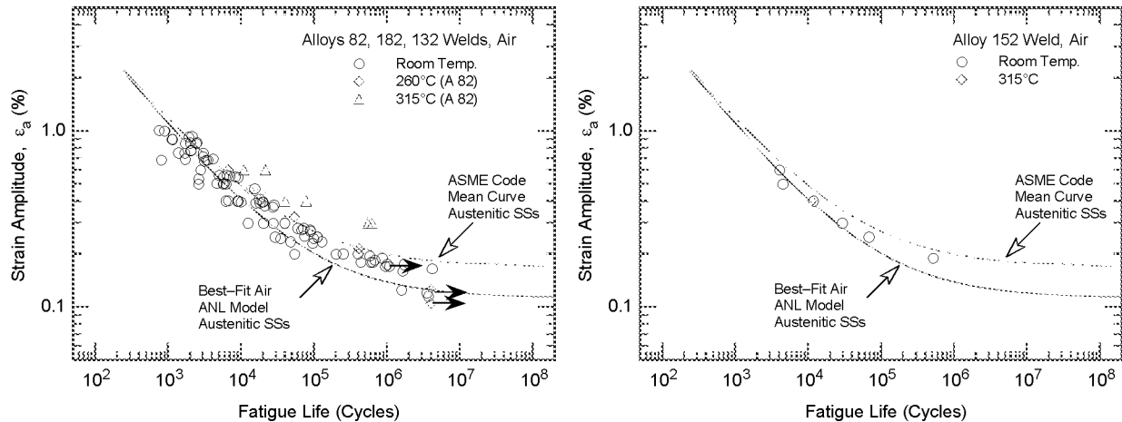
Figure 57. Fatigue \epsilon - N behavior for Alloys 82, 182, 132, and 152 welds in air at various temperatures (Refs. JNUFAD data, 72–78).
