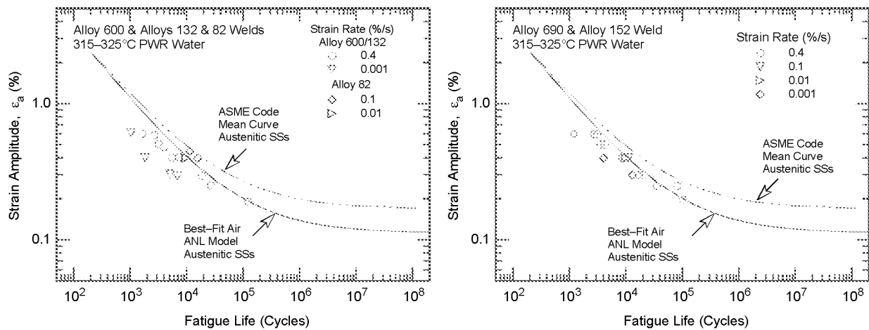
Figure 59. Fatigue \epsilon -N behavior for Alloys 600 and 690 and their weld alloys in simulated PWR water at 315 or 325^\circ\text{C} (Refs. 33, 78).
