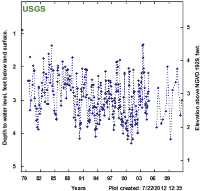
Monitoring Well Water Level Elevation Above NVGD 1929 (Seawater Reference Level)
