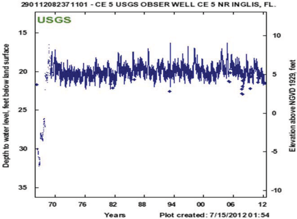
Monitoring Well Water Level Elevation Above NVGD 1929 (Seawater Reference Level)
