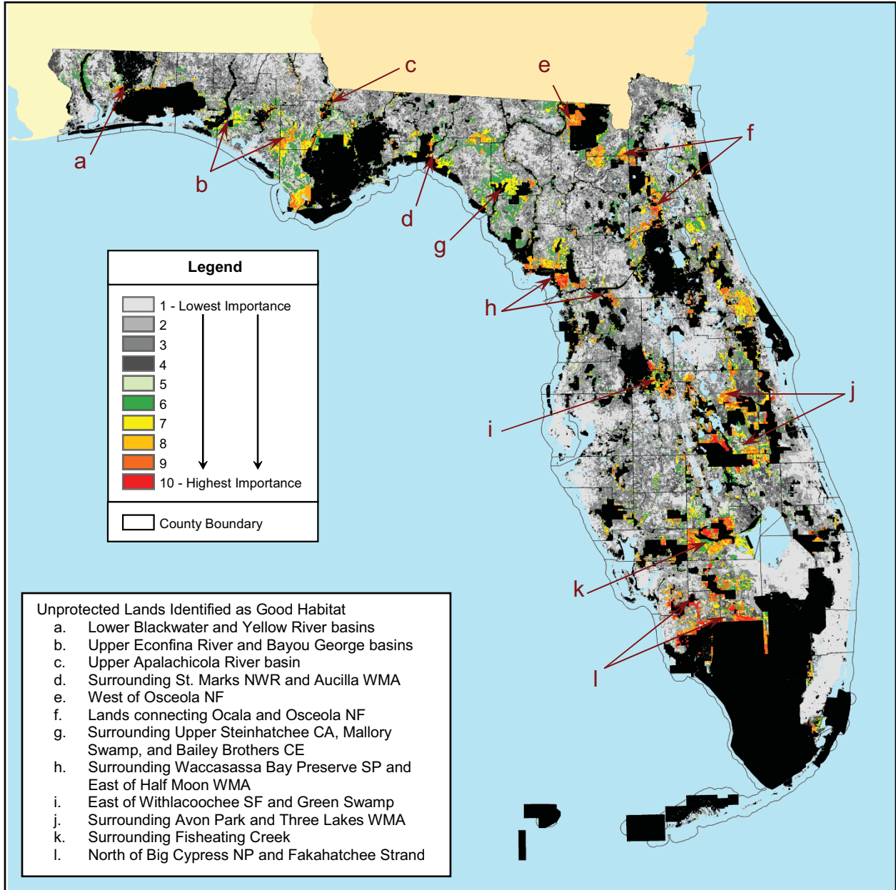
Figure 2. Final model calculation of the IWHRS 2009 with managed lands in black.
