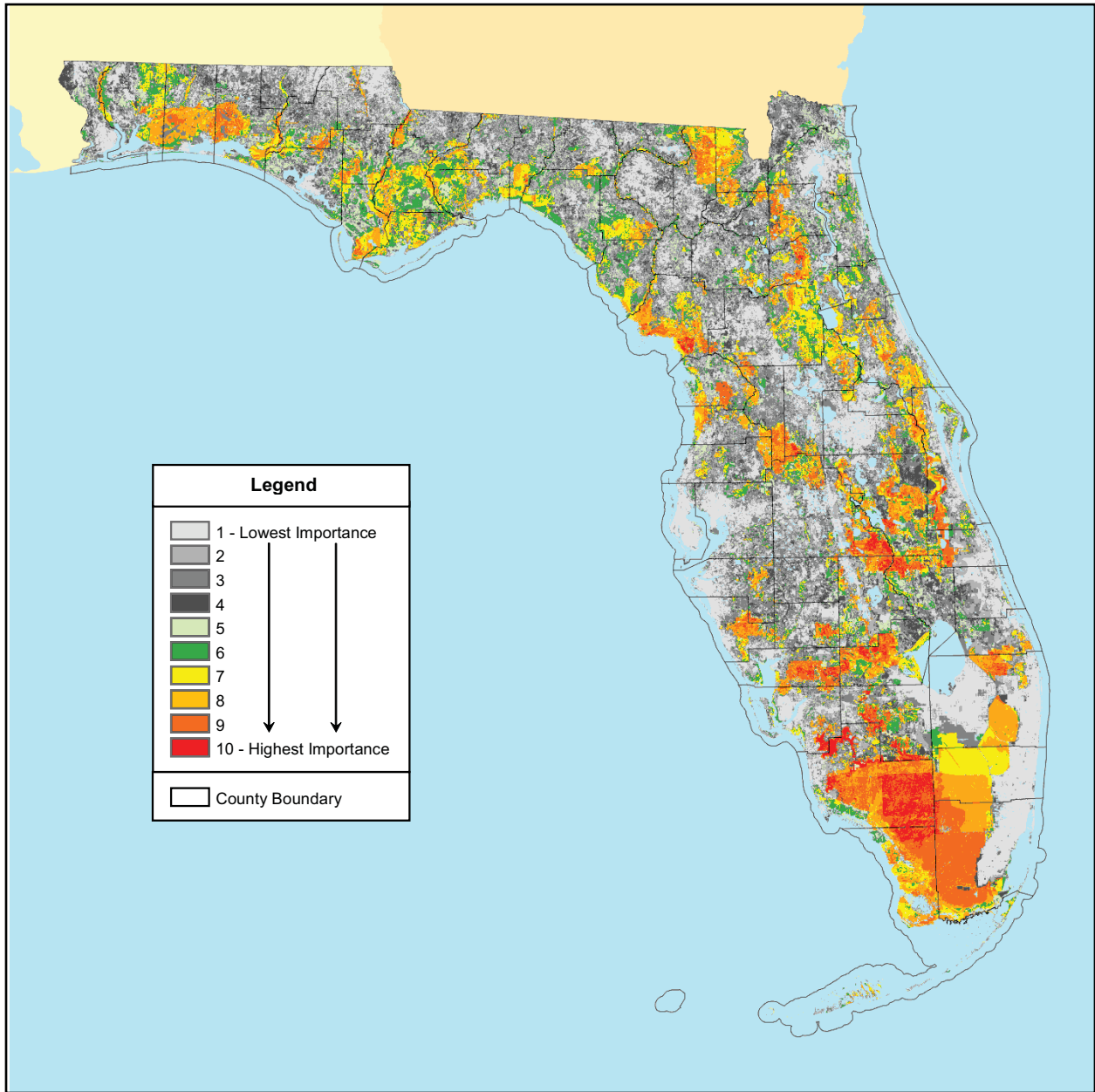
Figure 1. The final model calculation of the IWHRs 2009.
