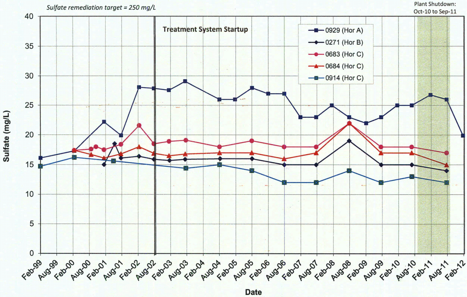
Figure E-5. Horizons A-C Sentinel Wells, Sulfate Concentrations
