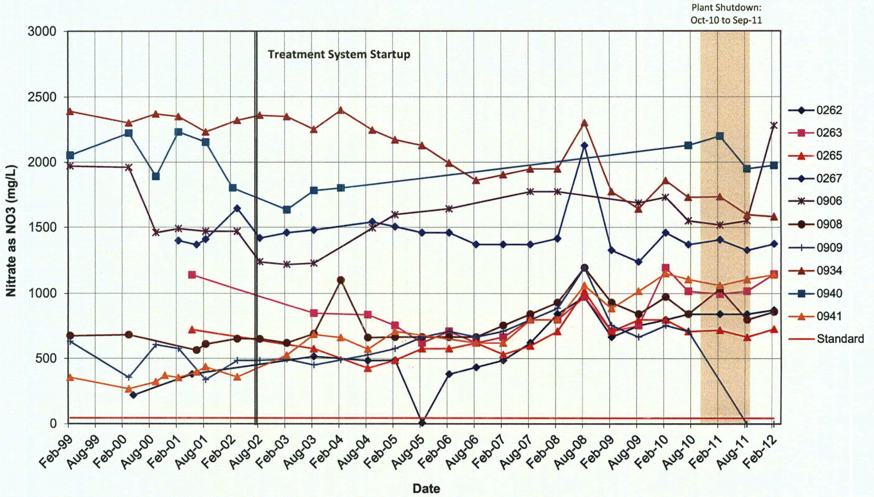
Figure E-1. Horizons A and B Monitoring Wells, Nitrate as NO 3 Concentrations
