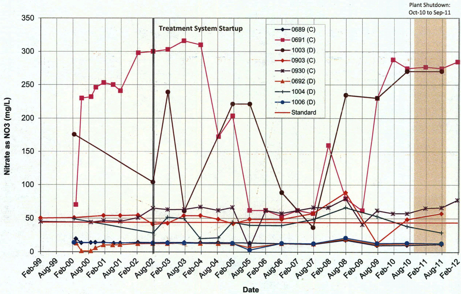
Figure E-10. Horizons C and D Lower Terrace Monitoring Wells, Nitrate as NO 3 Concentration
