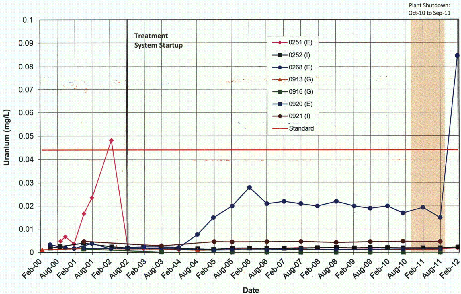
Figure E-15. Deep Monitoring Wells, Uranium Concentration.
