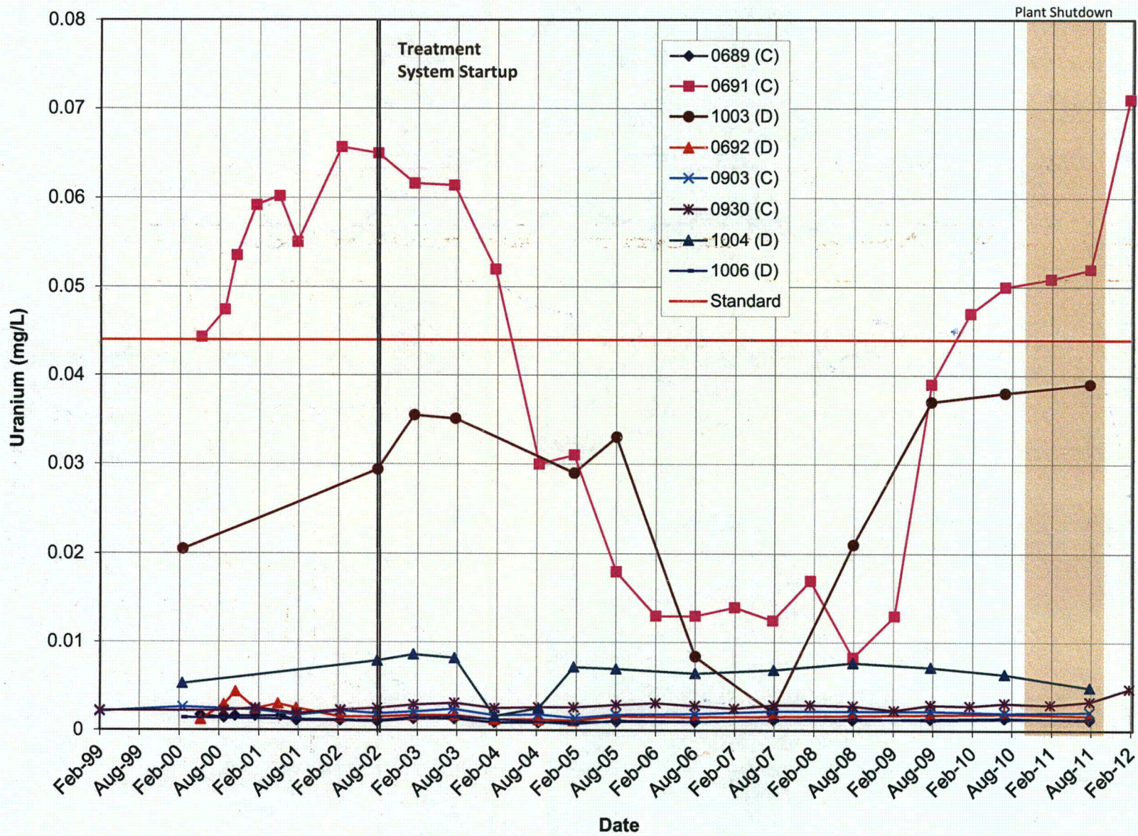
Figure E-12. Horizons C and D Lower Terrace Monitoring Wells, Uranium Concentration
