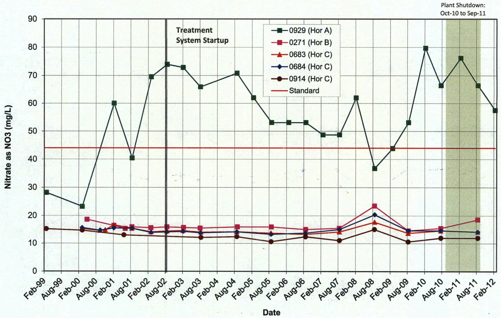
Figure E-4. Horizons A-C Sentinel Wells, Nitrate as NO 3 Concentrations
