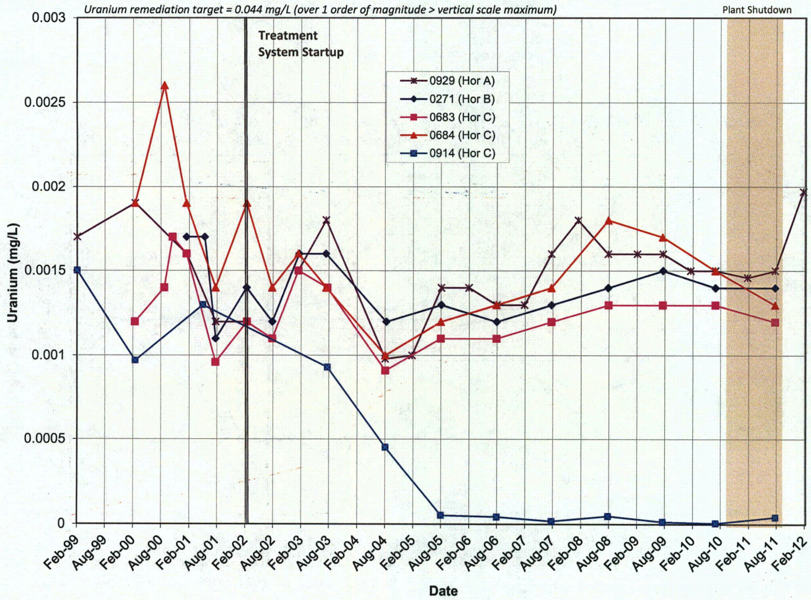
Figure E-6. Horizons A-C Sentinel Wells, Uranium Concentrations
