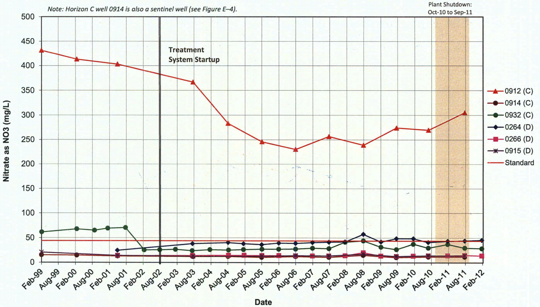
Figure E-7. Horizons C and D Monitoring Wells, Nitrate as NO 3 Concentration
