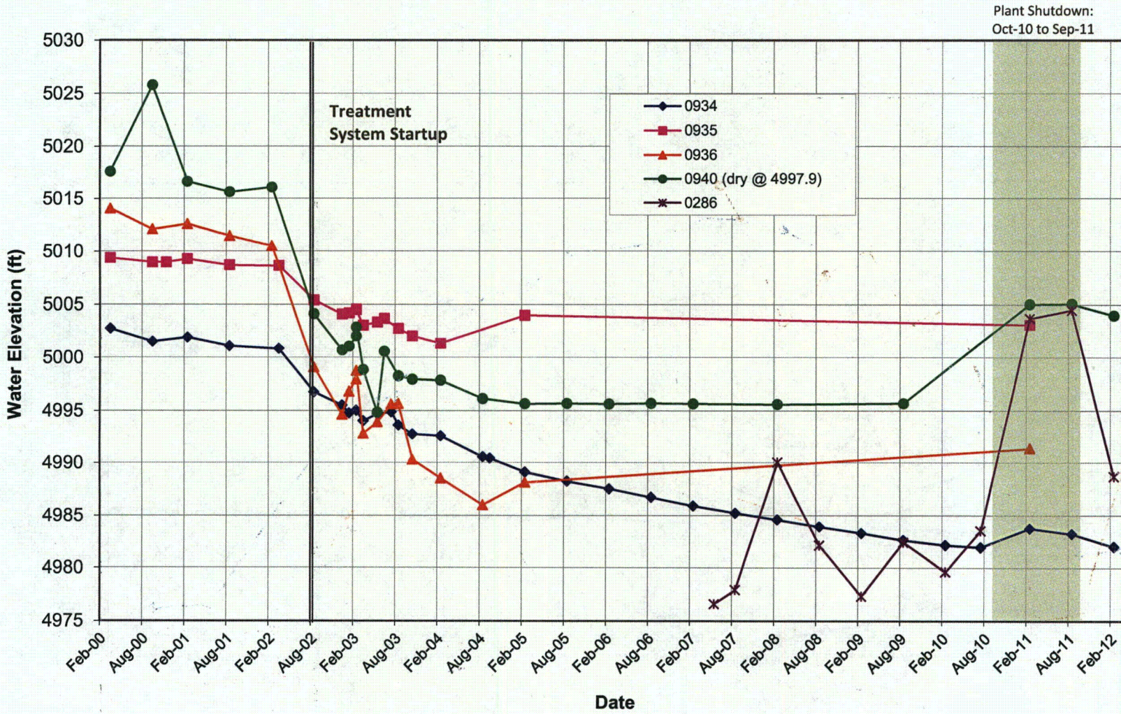
Figure D-2. Horizon A and B Monitoring Wells 286, 934-936, 940
