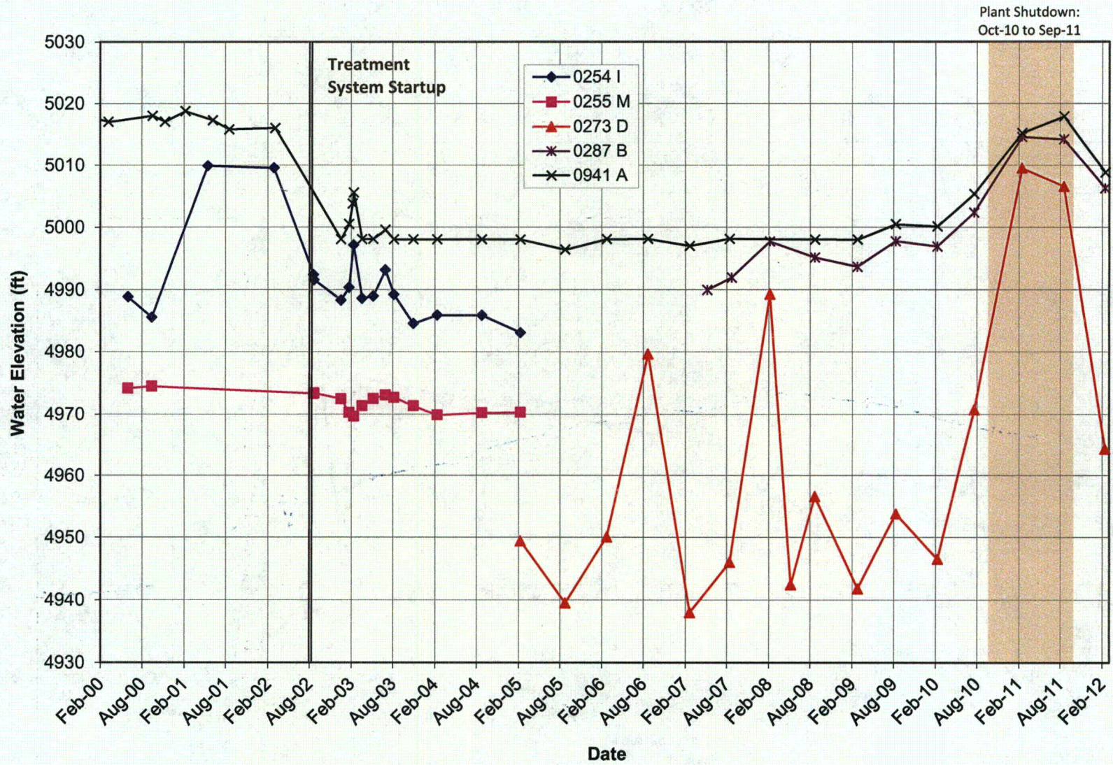
Figure D-10. Middle Terrace Well Cluster 254, 255, 273, 287, and 941
