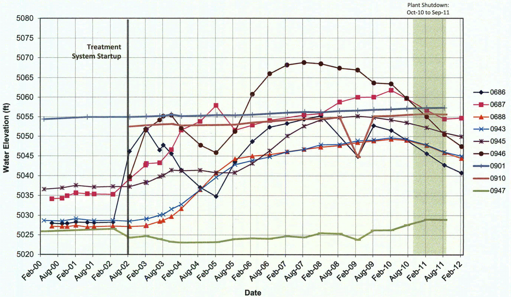
Figure D-1. Monitoring Wells at Infiltration Trench (686-688, 943, 945, 946) and Background Wells 901, 910, and 947
