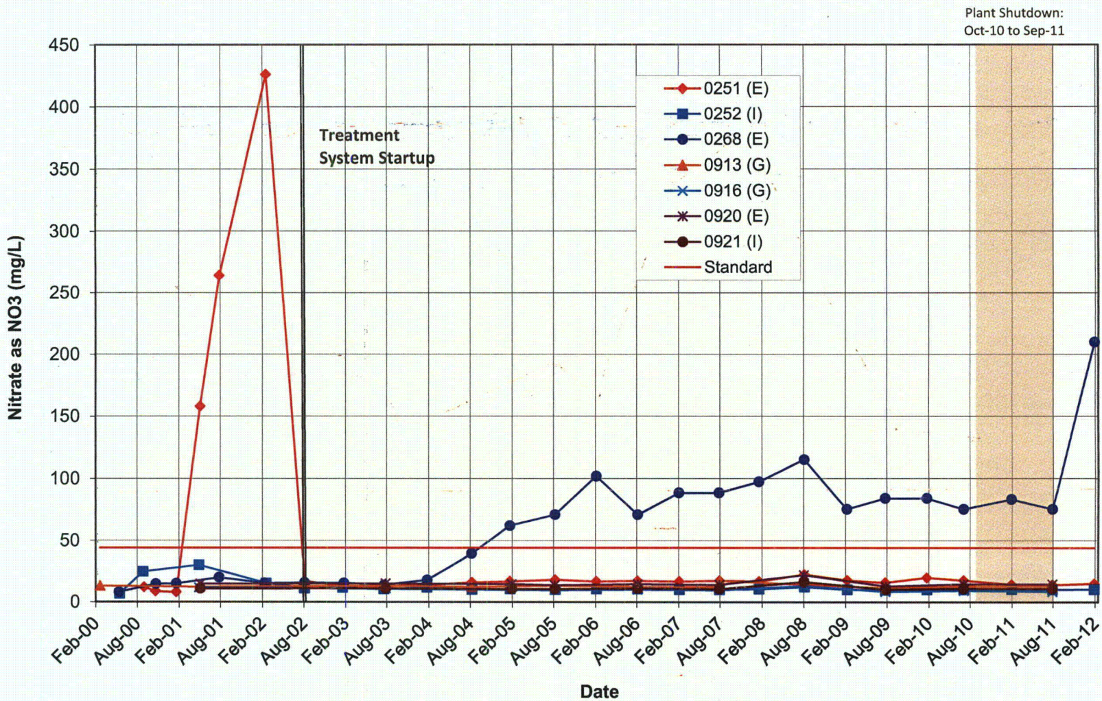
Figure E-13. Deep Monitoring Wells, Nitrate as NO 3 Concentration
