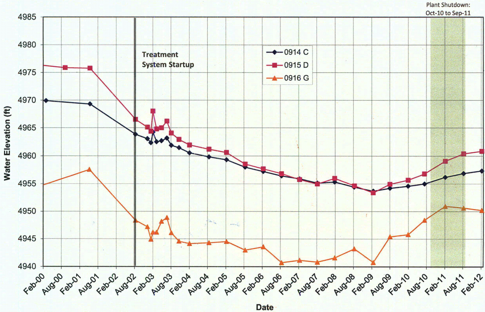
Figure D-11. Middle Terrace Well Cluster 914, 915, and 916
