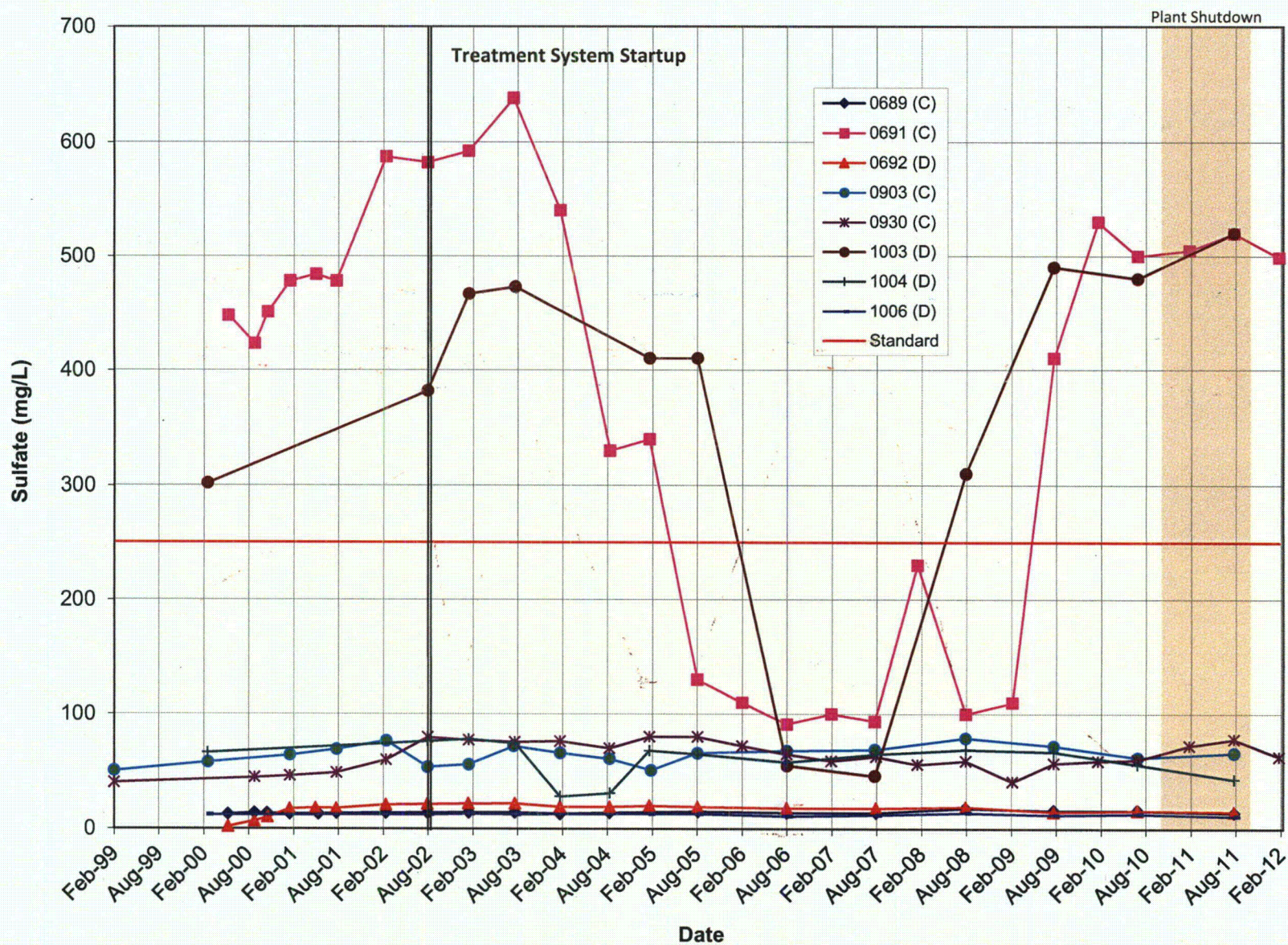
Figure E-11. Horizons C and D Lower Terrace Monitoring Wells, Sulfate Concentration
