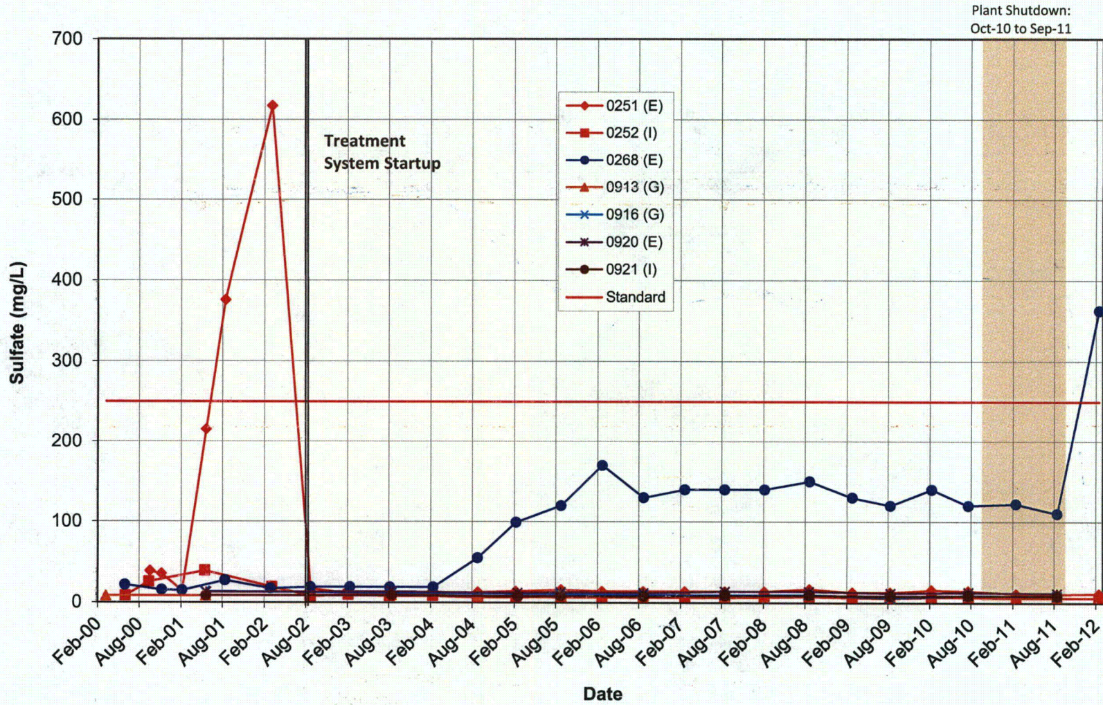
Figure E-14. Deep Monitoring Wells, Sulfate Concentration
