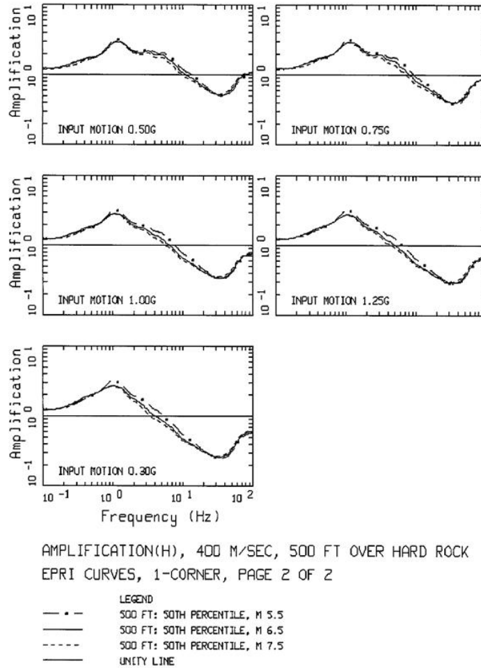
Figure B-11b. Comparison of amplification functions (5%-damped PSa) computed for magnitudes of M 5.5, 6.5, and 7.5, using the single-corner source model and the 400 m/sec VS30 stiff-soil template profile (Figure B-2) with the EPRI (1993) [12] G/GMAX and hysteretic damping curves (Figure B-7). The input reference rock loading levels varied from 0.01 to 1.50 g (Table B-4).
