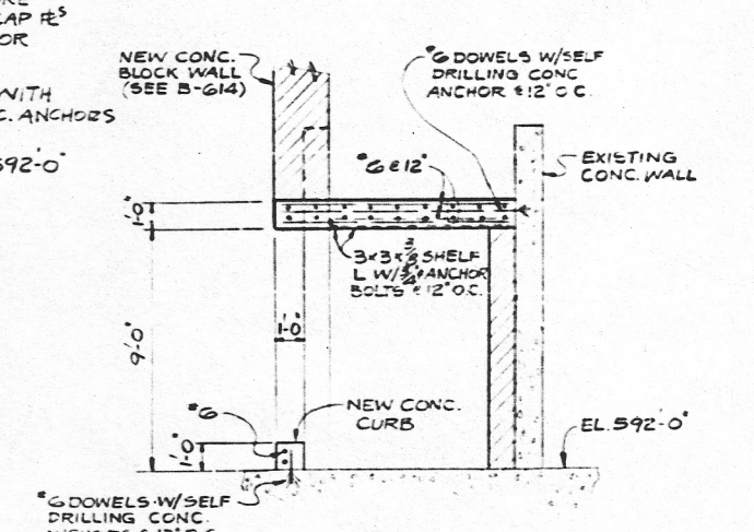
SECTION 107-107 (B-723) SCALE 1/4\"/>
