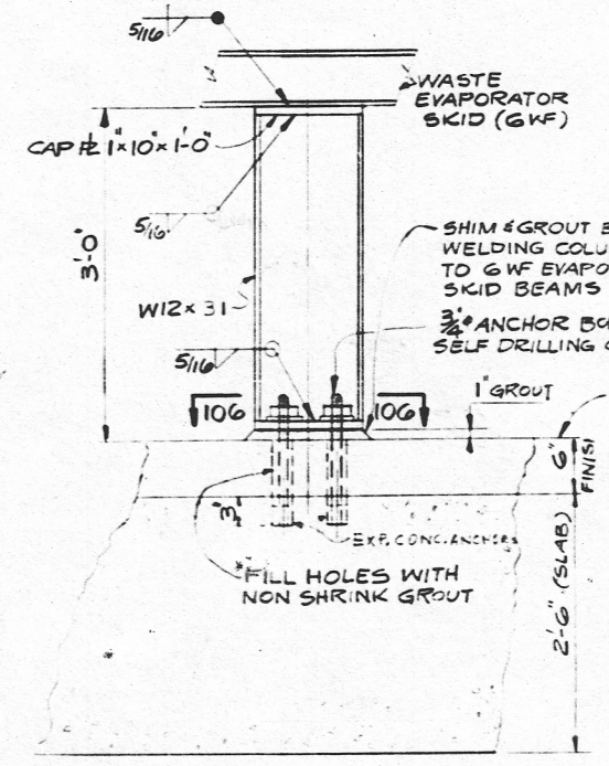
SECTION 105-105 (B-723) SCALE 1/4\"/>
