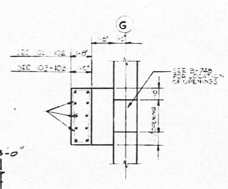
SECTION 102-102 (B-733, B-734) SECTION 103-103 (B-733)
