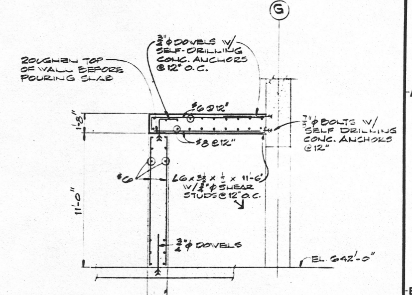
SECTION 104-104 (B-733, B-745)
