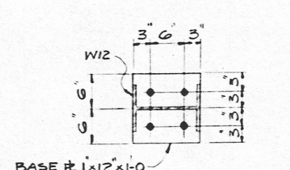
SECTION 106-106 SCALE 1/4\"/>
