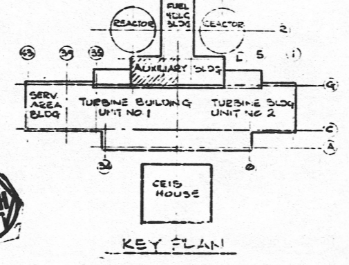
AUXILIARY BUILDING WALL PLAN EL. 642'-0" SOUTHEAST AREA
