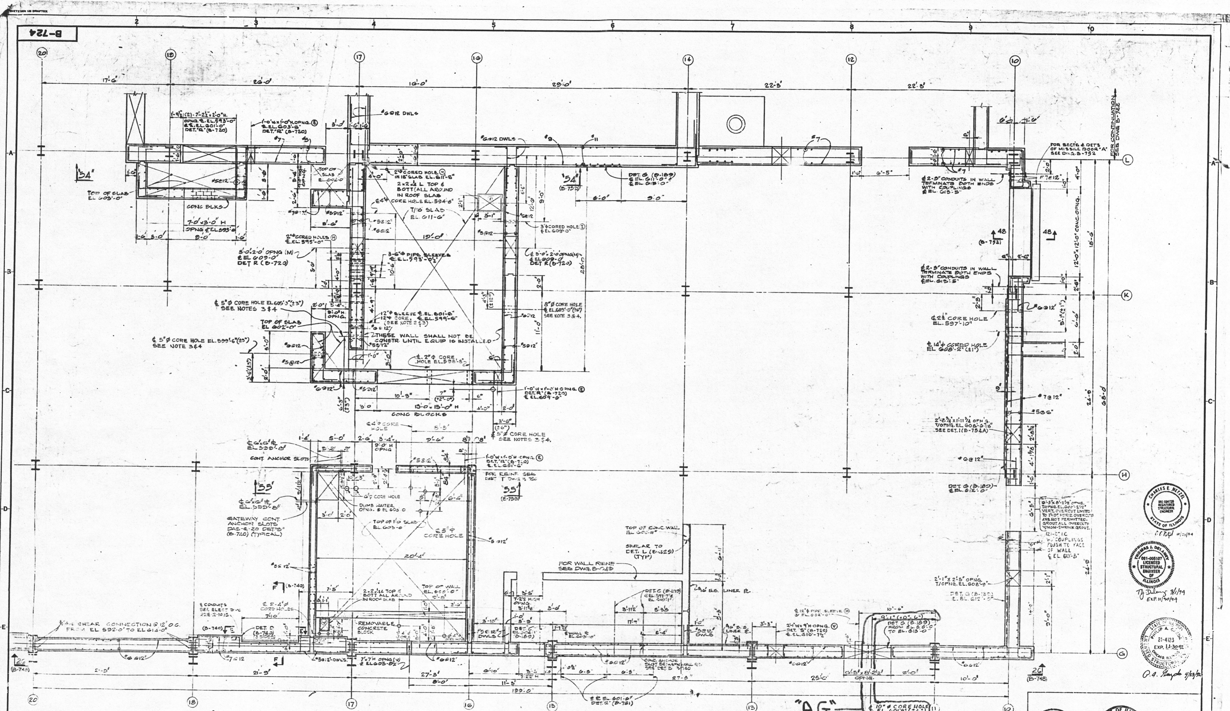
AUXILIARY BUILDING WALL PLAN EL 592'-0" NORTH EAST AREA
