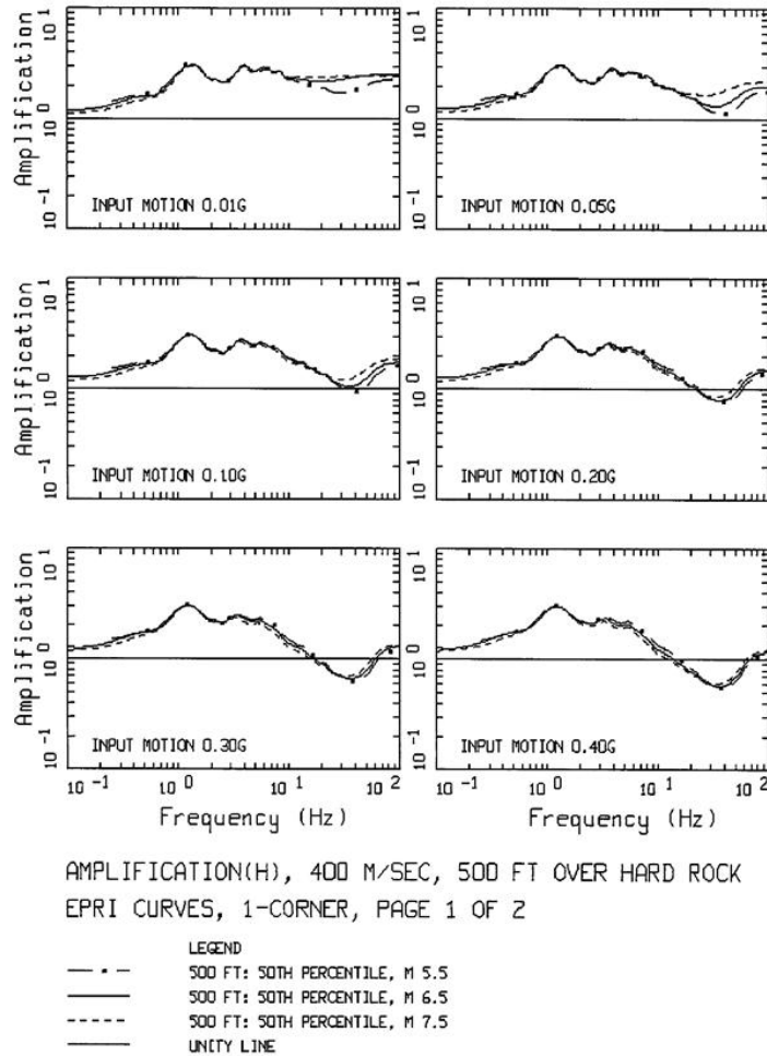
Figure B-11a. Comparison of amplification functions (5%-damped PSa) computed for magnitudes of M 5.5, 6.5, and 7.5, using the single-corner source model and the 400 m/sec VS30 stiff-soil template profile (Figure B-2) with the EPRI (1993) [12] G/GMAX and hysteretic damping curves (Figure B-7). The input reference rock loading levels varied from 0.01 to 1.50 g (Table B-4).
