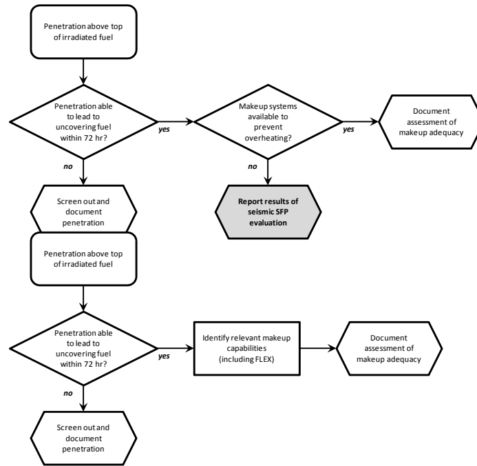
Figure 7-2 Basic Process for Evaluation of Potential Failures for Penetrations above Top of Irradiated Fuel
