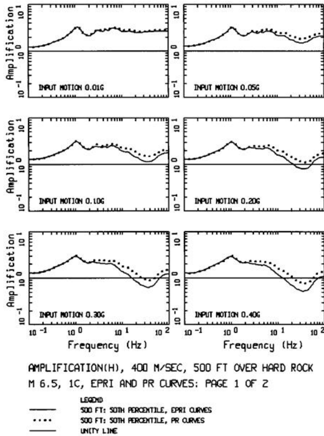
Figure B-8a. Comparison of median amplification functions (5%-damped PSa) derived using the EPRI (1993) [12] (see Figure B-7) and Peninsular Range [28]) G/GMAX and hysteretic damping curves. The results are for the 400 m/sec VS30 template profile and a single-corner source model for reference rock loading levels of 0.01 to 1.50g.
