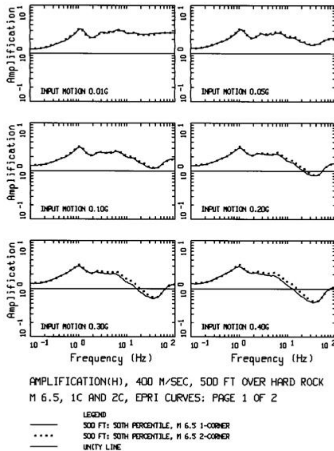
Figure B-12a. Comparison of amplification functions (5% damped PSa) computed using the Single- and Double-Corner source models (Tables B-4 and B-6) for the 400 m/sec VS30 stiff-soil template profile (Figure B-2) with the EPRI (1993) [12] G/GMAX and hysteretic damping curves (Figure B-7). The input reference rock loading levels varied from 0.01 to 1.50 g (Tables B-4 and B-6).
