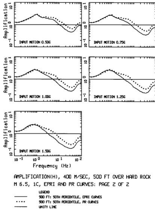
Figure B-8b. Comparison of median amplification functions (5%-damped PSa) derived using the EPRI (1993) [12] (see Figure B-7) and Peninsular Range [28] G/GMAX and hysteretic damping curves. The results are for the 400 m/sec VS30 template profile and a single-corner source model for reference rock loading levels of 0.01 to 1.50g.
