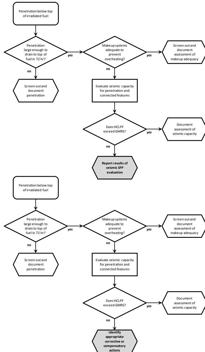
Figure 7-1 Basic Process for Evaluation of Potential Failures for Penetrations below Top of Irradiated Fuel
