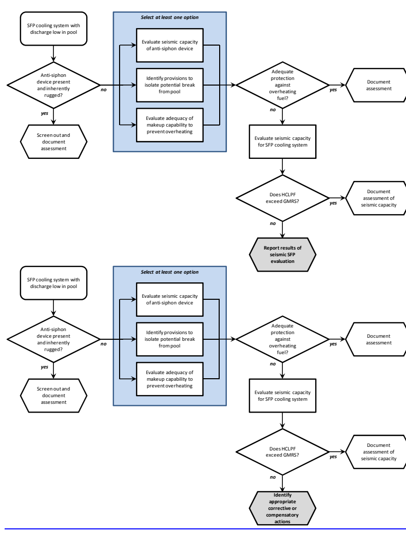
Figure 7-3 Basic Process for Evaluation of Potential Siphoning of SFP Inventory
