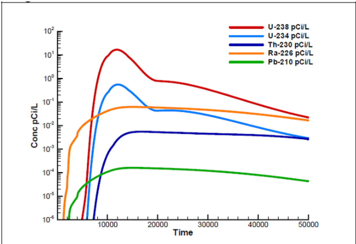
Figure A4A-91. ILV well concentration for U-238
