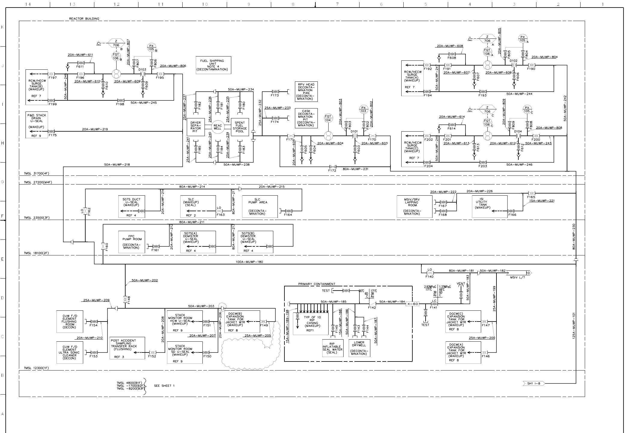
Figure 9.2-5 – Makeup Water System (Purified) P&ID (Sheet 2 of 3)
