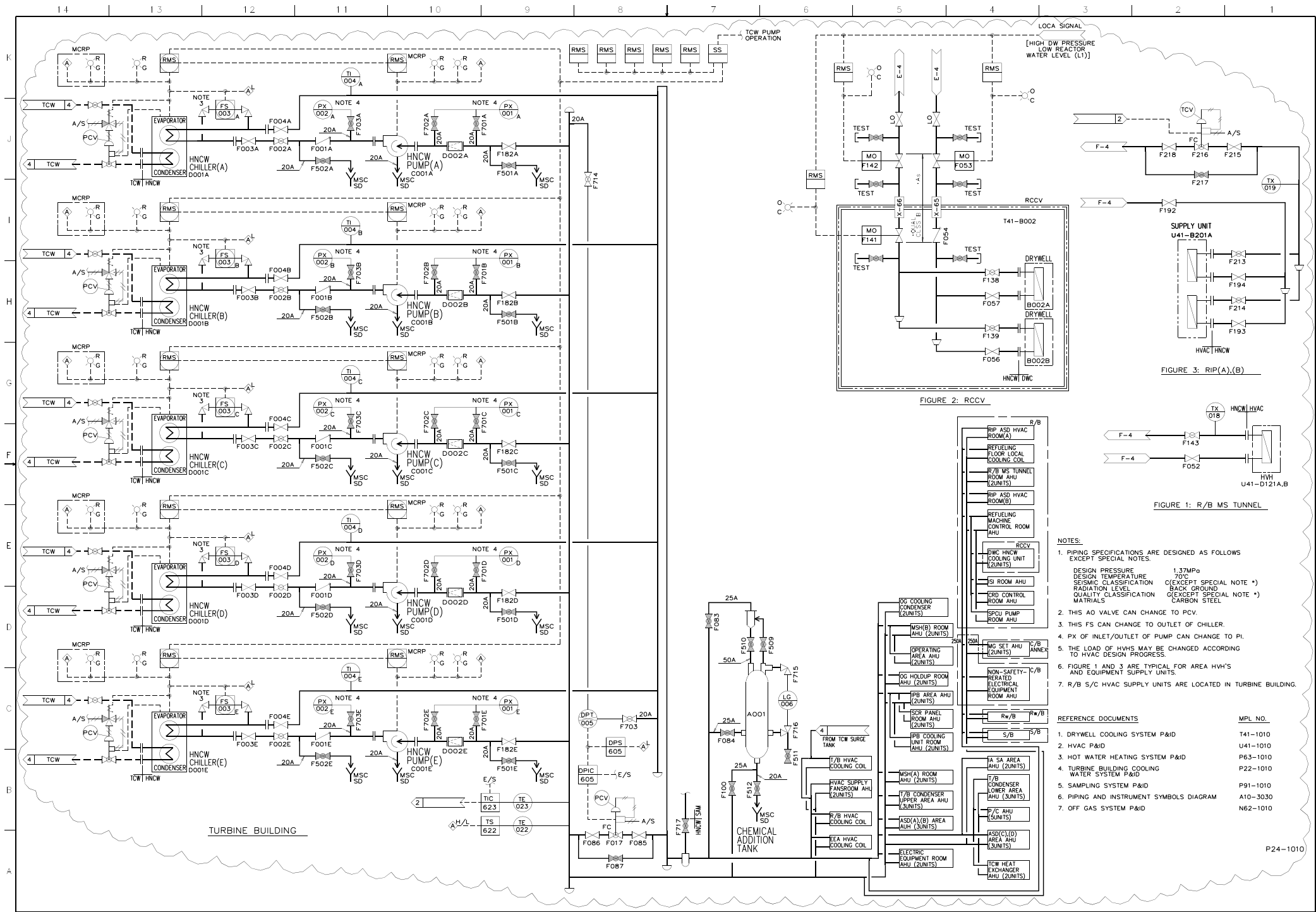
Figure 9.2-2 – Hvac Normal Cooling Water System P&ID
