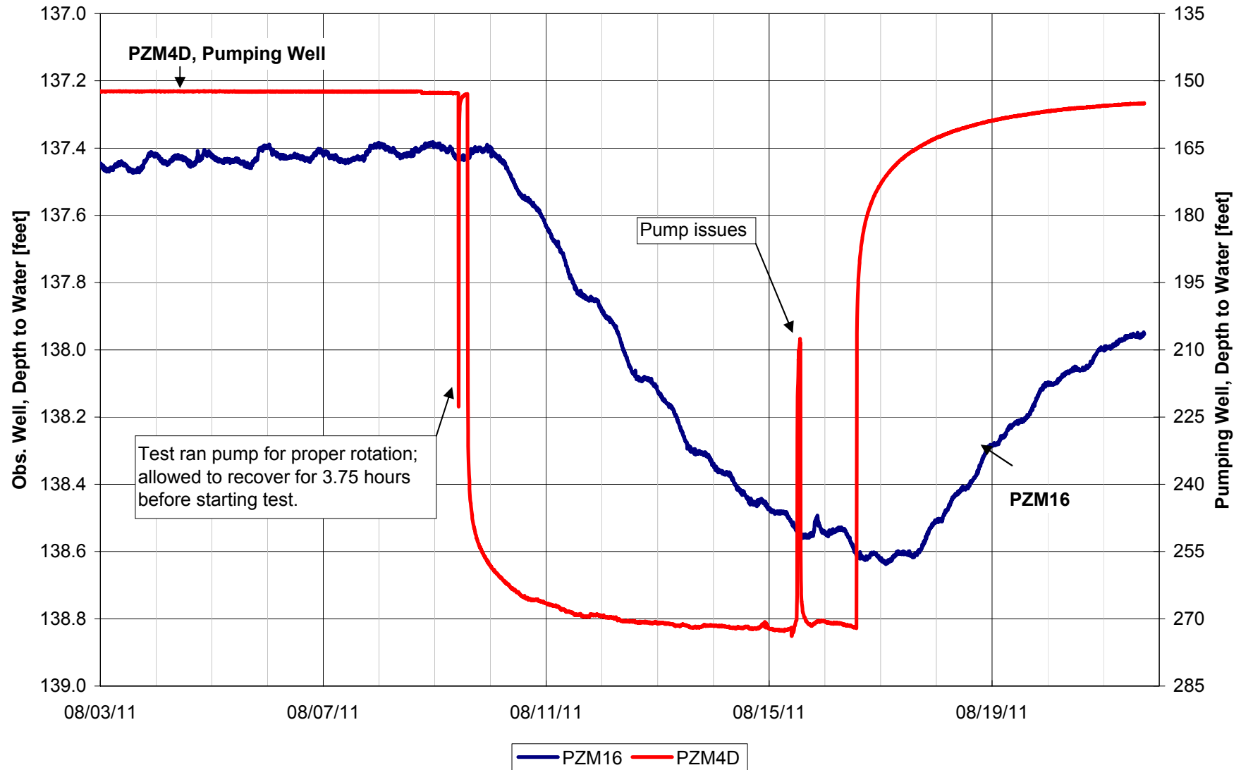
Figure 2.7B-35. Production Zone Observation Well vs. Pumping Well Water Level, Well PZM16, PZM4D Pump Test Reno Creek Project
