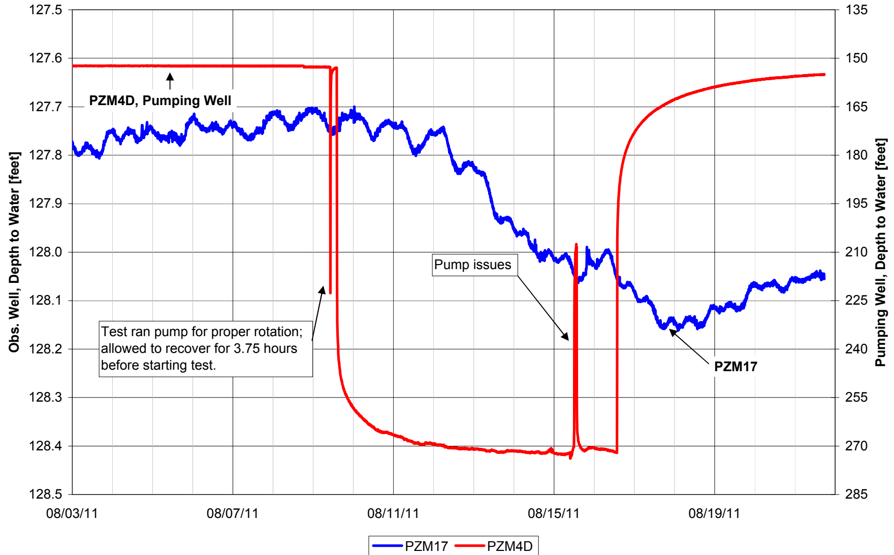
Figure 2.7B-37. Production Zone Observation Well vs. Pumping Well Water Level Well PZM17, PZM4D Pump Test Reno Creek Project
