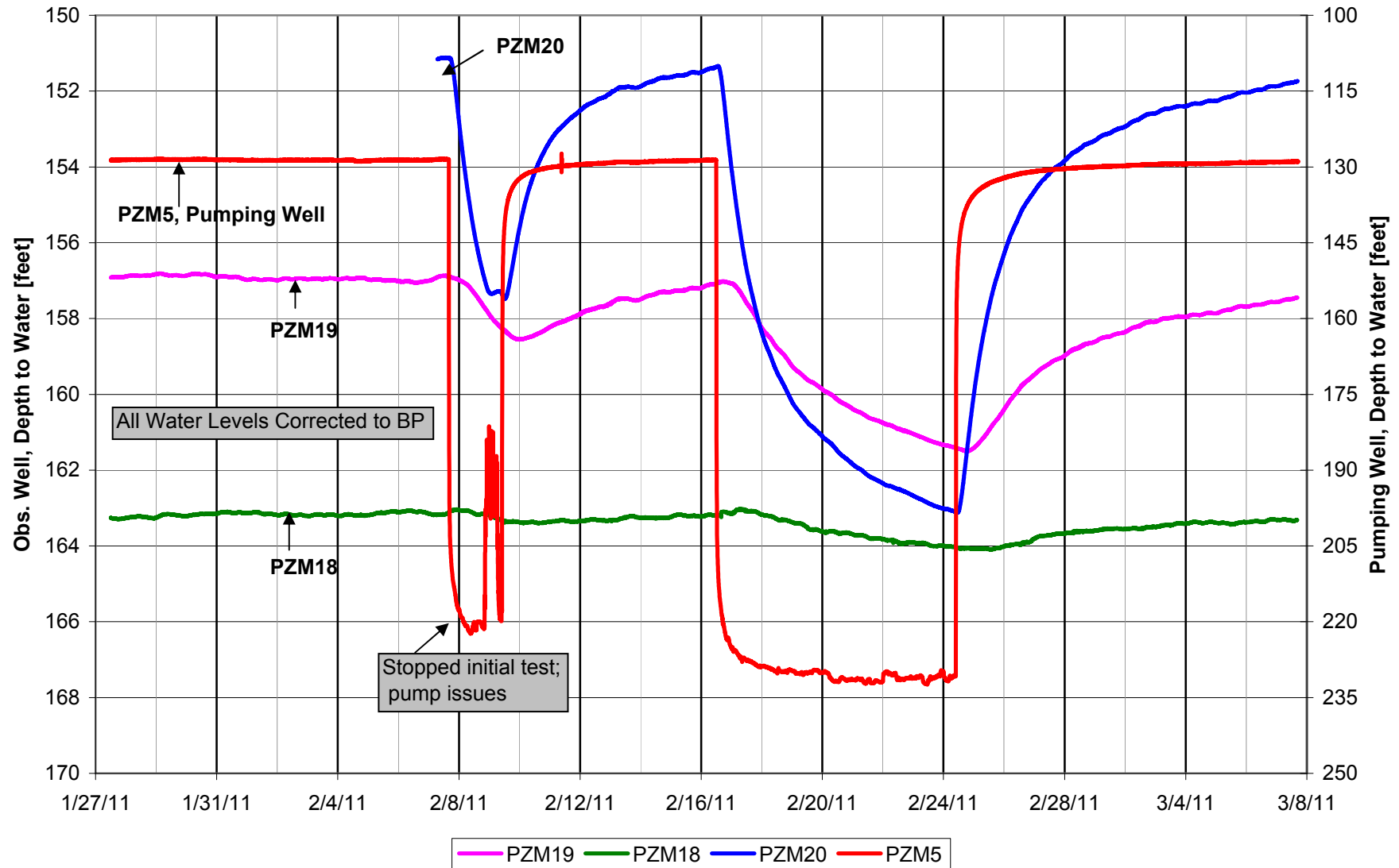
Figure 2.7B-45. Production Zone Observation Wells vs. Pumping Well Water Level Data, Wells PZM18, PZM19, PZM20, PZM5 Pump Test Reno Creek Project
