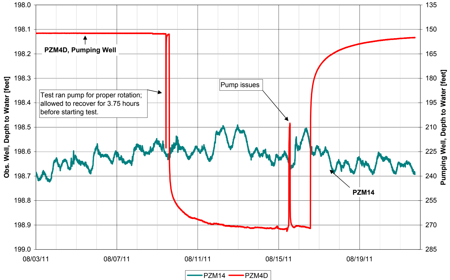
Figure 2.7B-38. Production Zone Observation Well vs. Pumping Well Water Level Well PZM14, PZM4D Pump Test Reno Creek Project
