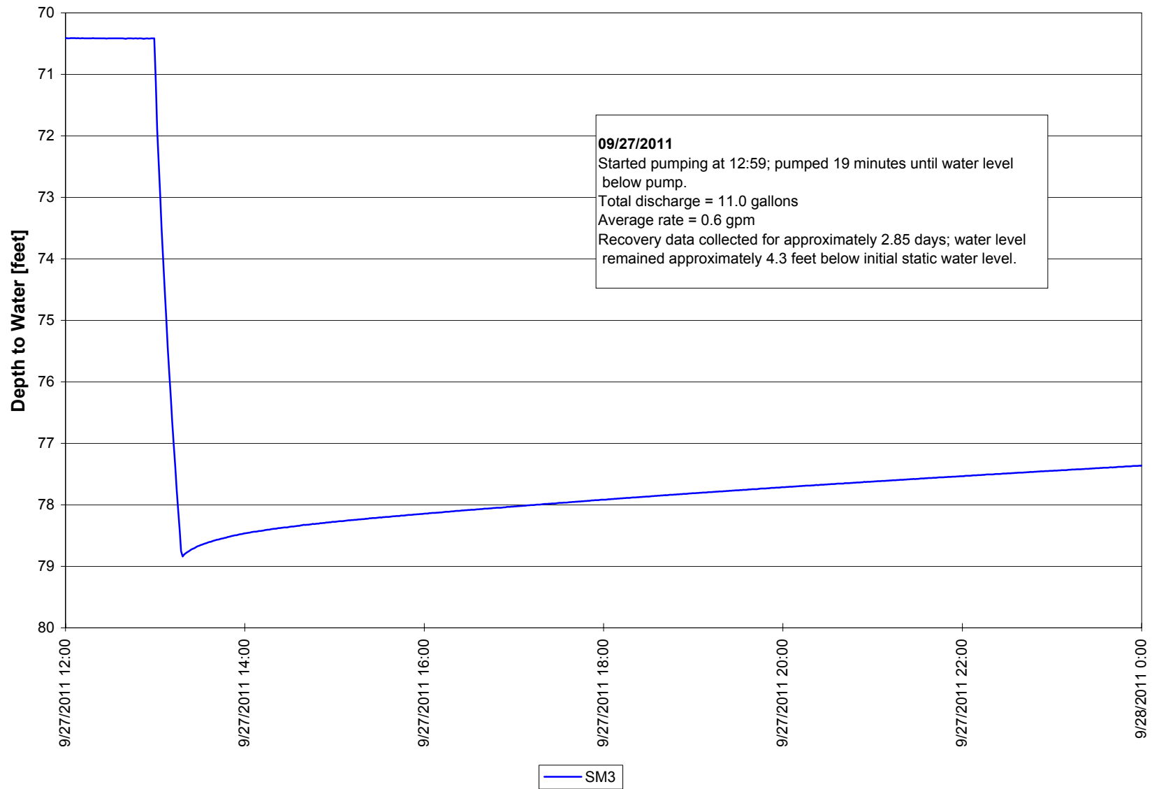
Figure 2.7B-31. SM3 Single-well Test Water Level Data Reno Creek Project
