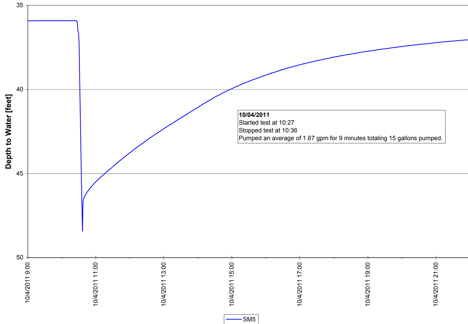
Figure 2.7.B-51. SM5 Single-well Test Water Level Data Reno Creek Project
