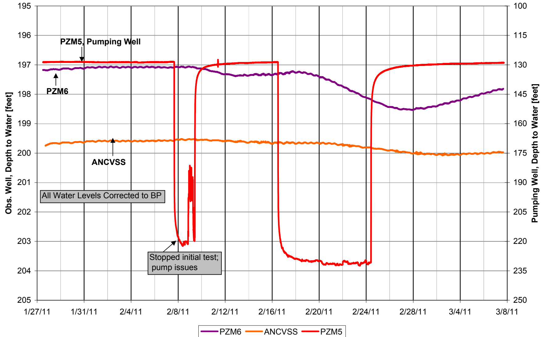
Figure 2.7B-46. Production Zone Observation Wells vs. Pumping Well Water Level Data, Wells PZM6 and BLM ANCVSS, PZM5 Pump Test Reno Creek Project
