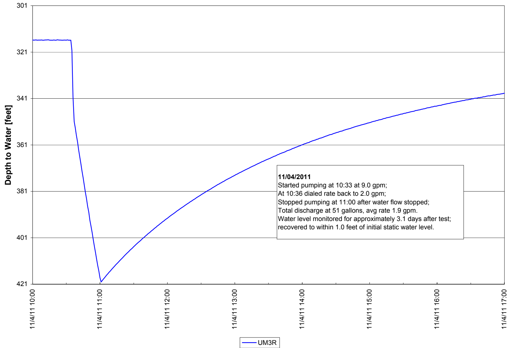
Figure 2.7B-33. UM3R Single-well Test Water Level Data Reno Creek Project
