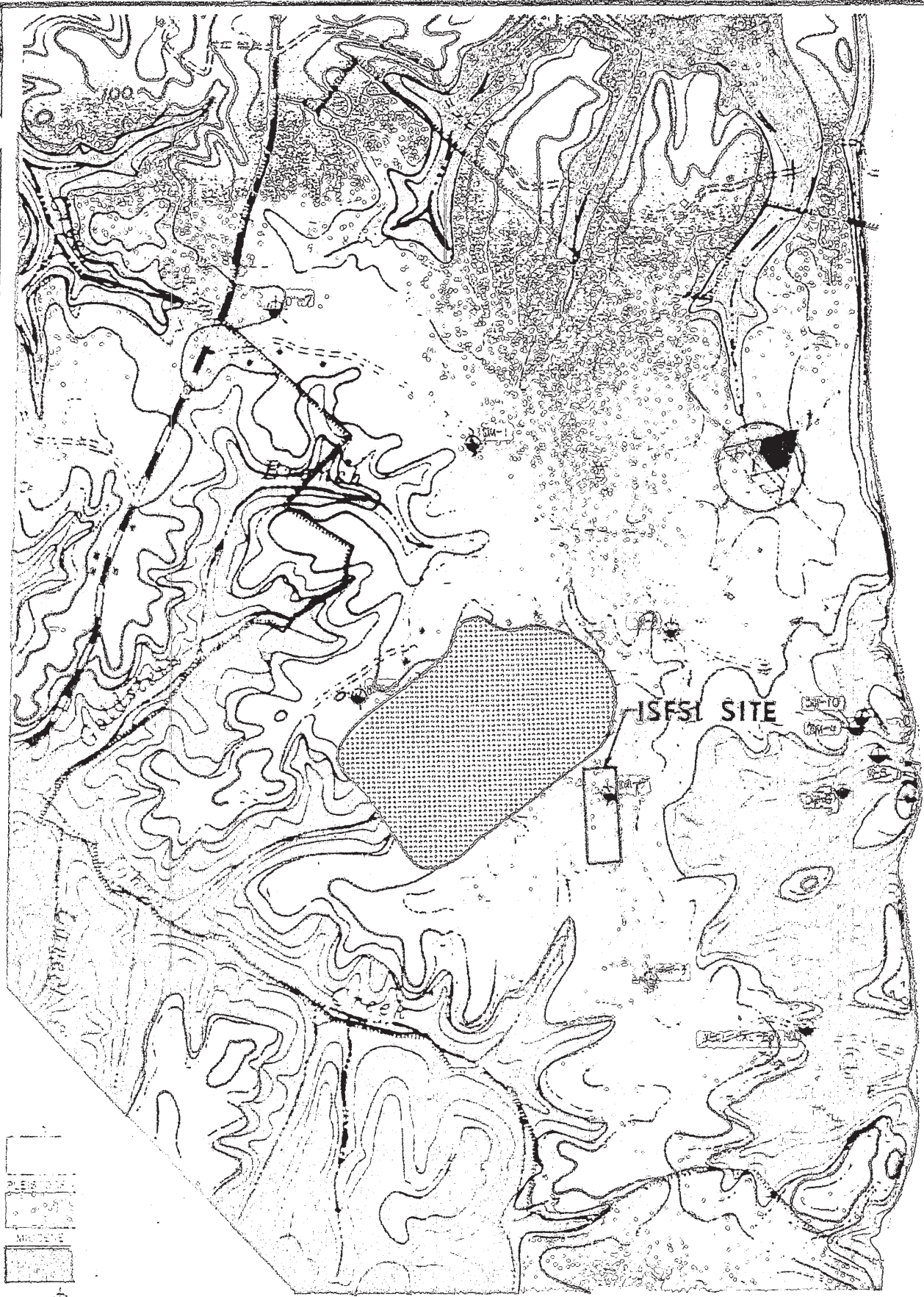
SITE GEOLOGIC MAP
