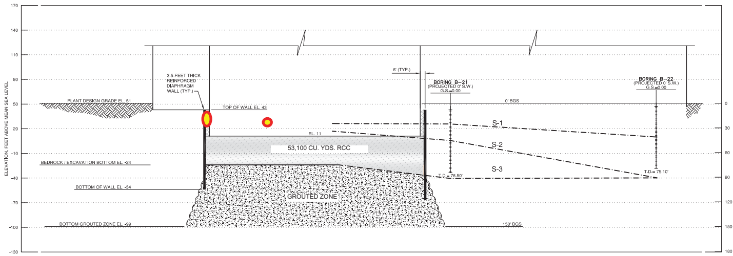
SECTION A
