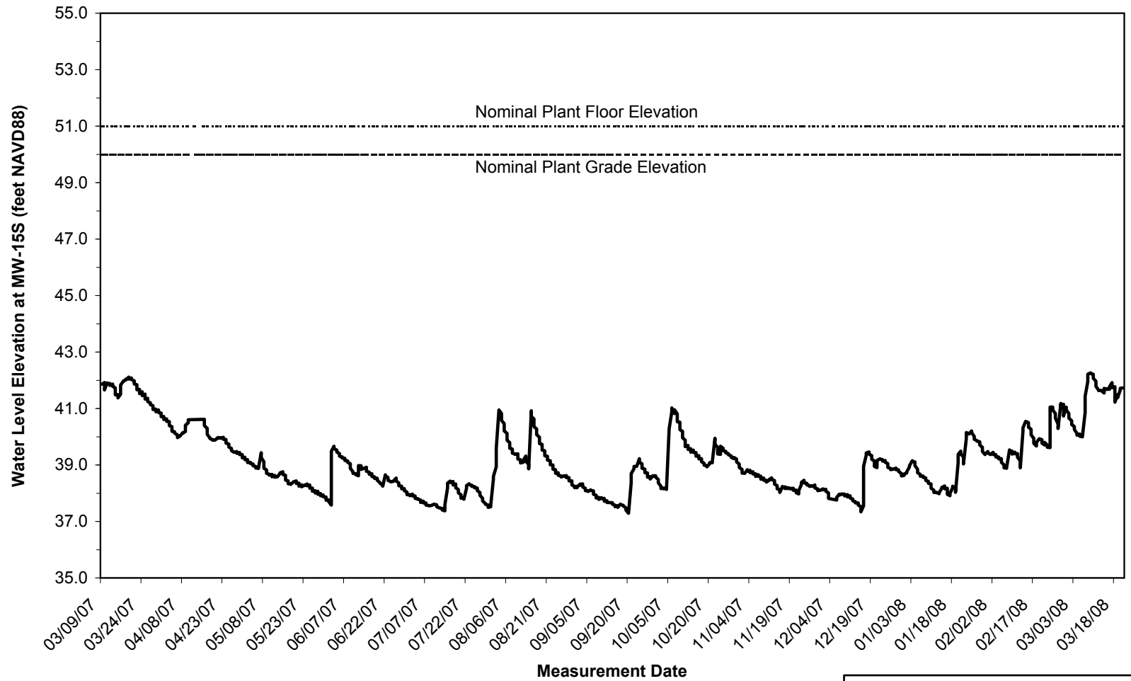
Progress Energy Florida Levy Nuclear Plant Units 1 and 2 Part 2, Final Safety Analysis Report Surficial Aquifer Groundwater Elevation at LNP 1 FIGURE 2.4.12-223 Rev 0
