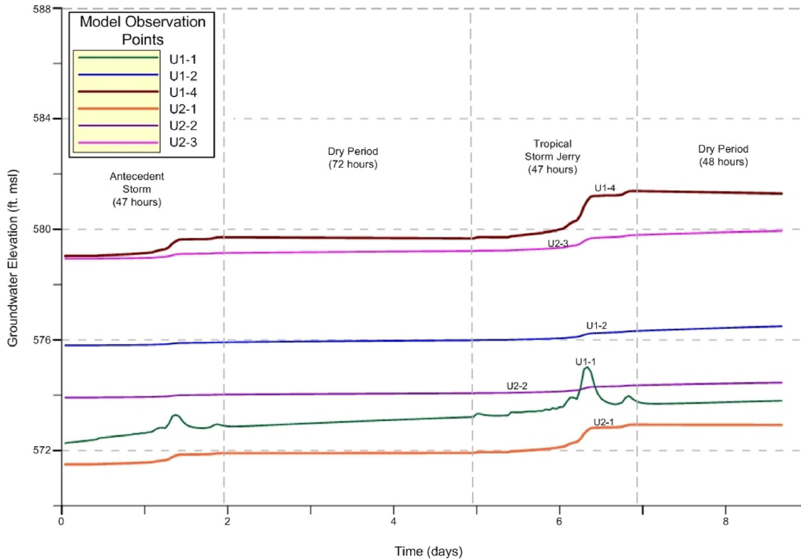
WILLIAM STATES LEE III NUCLEAR STATION UNITS 1 & 2 Maximum Post-Construction Groundwater Analysis, Results Hydrograph FIGURE 2.4.12-211 Rev 6
