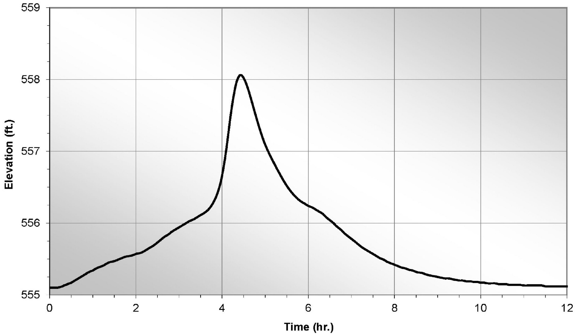
WILLIAM STATES LEE III NUCLEAR STATION UNITS 1 & 2 Flood Elevation Hydrograph Make-Up Pond A 6-Hour Local Intense Precipitation FIGURE 2.4.3-233 Rev 6
