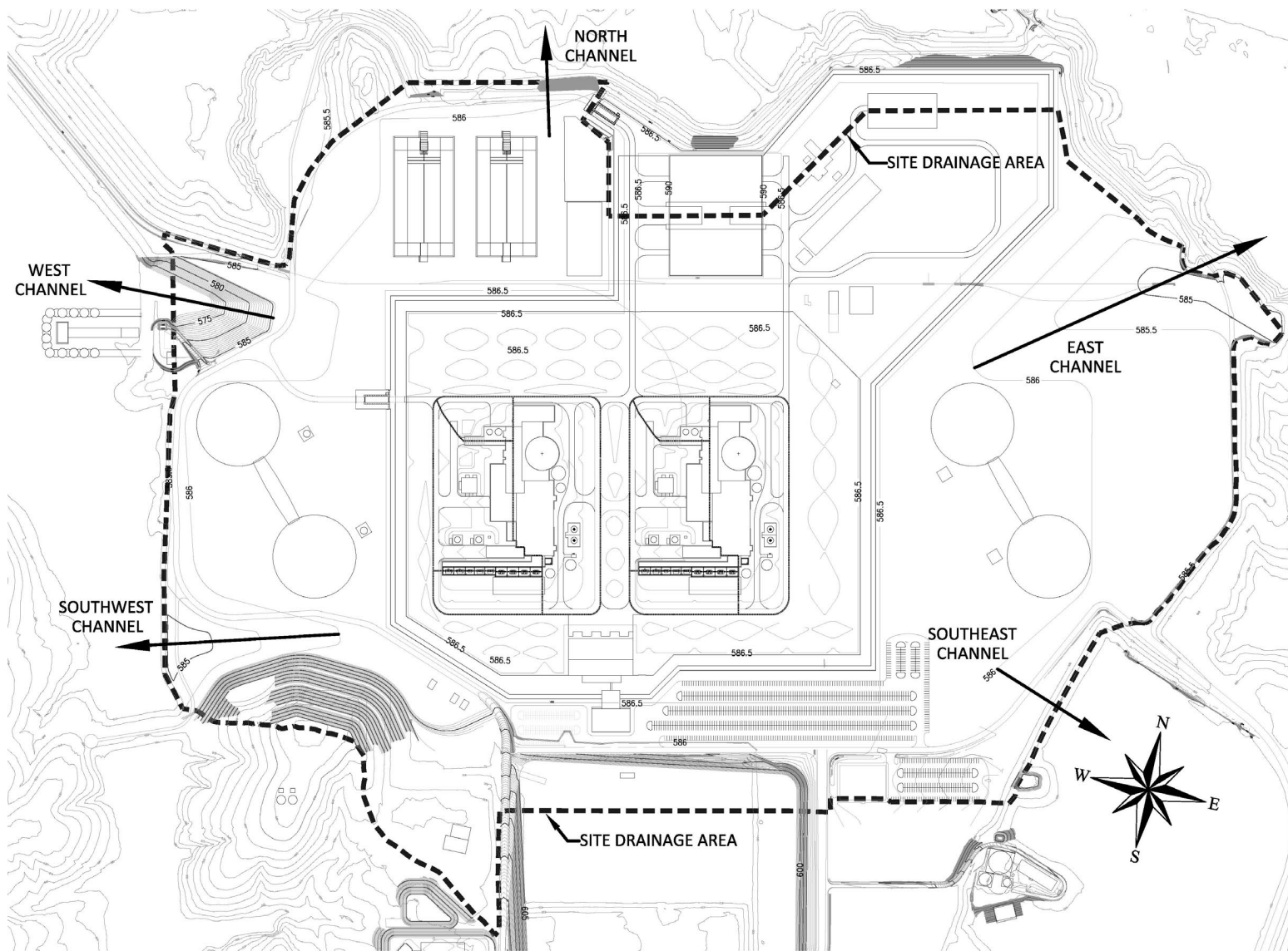
WILLIAM STATES LEE III NUCLEAR STATION UNITS 1 & 2 Grading and Drainage Plan FIGURE 2.4.2-202 Rev 6
