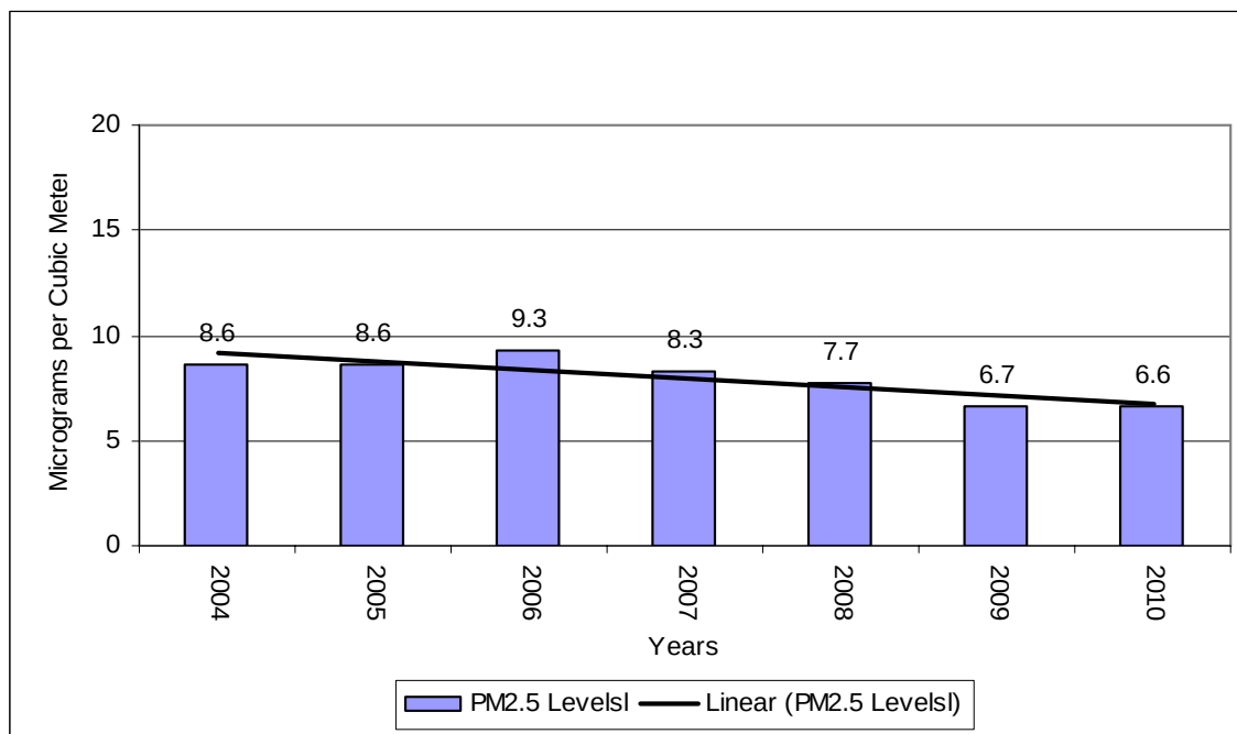
Figure 7-8 – RC Credit Union PM 2.5 Annual Averages
