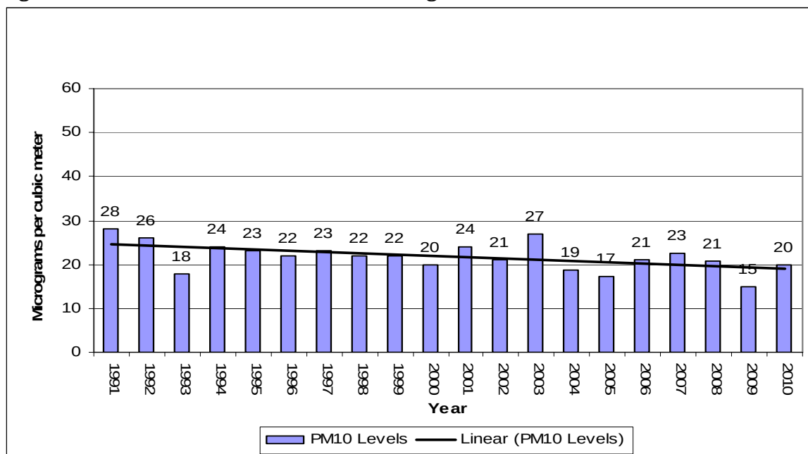
Figure 7-25 – SF KELO PM 10 Annual Averages
