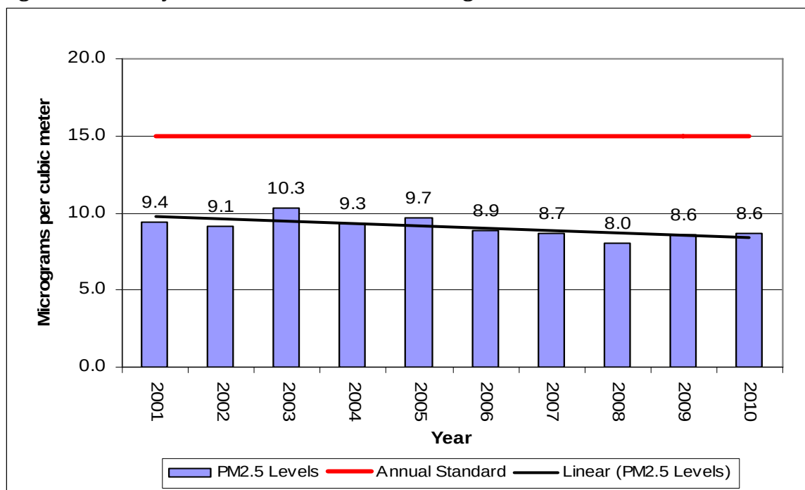
Figure 7-38 – City Hall Site PM 2.5 Annual Averages
