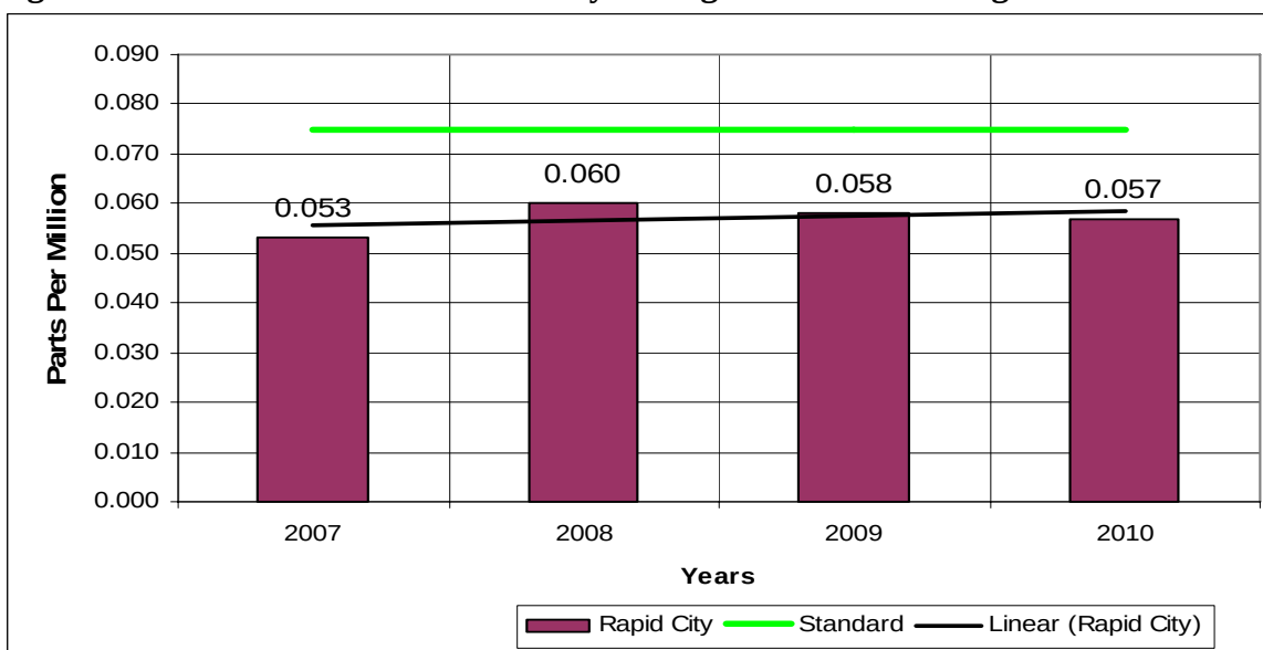
Figure 7-11 – Black Hawk Ozone Yearly 4 th Highest 8-hour Averages
