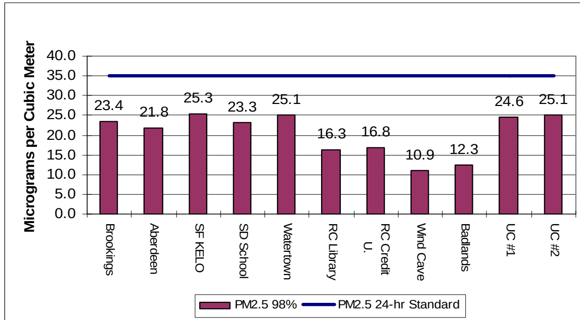
Figure 6-2 – 2010 PM 2.5 Statewide 24-Hour design values 1
