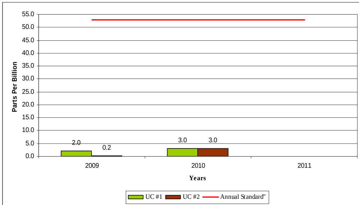
Figure 7-49 – Union County Nitrogen Dioxide Concentrations
