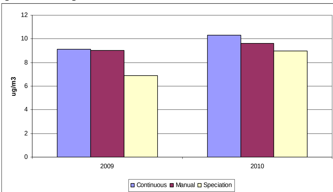
Figure 8-2 – Average PM 2.5 Concentration
