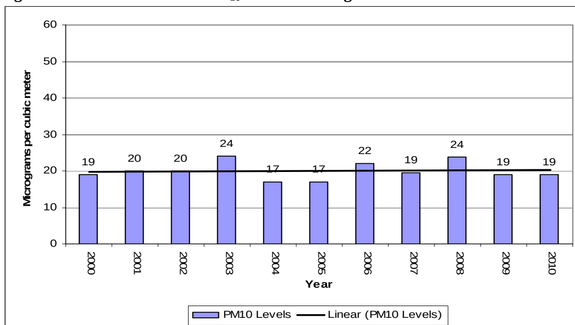
Figure 7-34 – Fire Station #1 PM 10 Annual Averages
