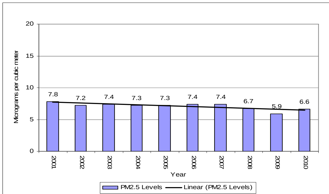
Figure 7-3 – RC Library PM 2.5 Annual Averages
