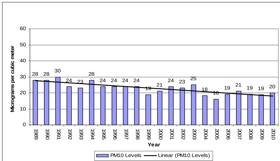
Figure 7-2 – RC Library PM 10 Annual Averages
