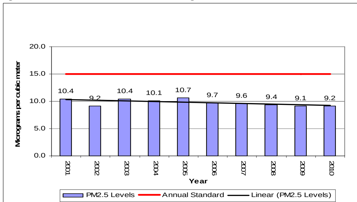
Figure 7-26 – SF KELO PM 2.5 Annual Averages
