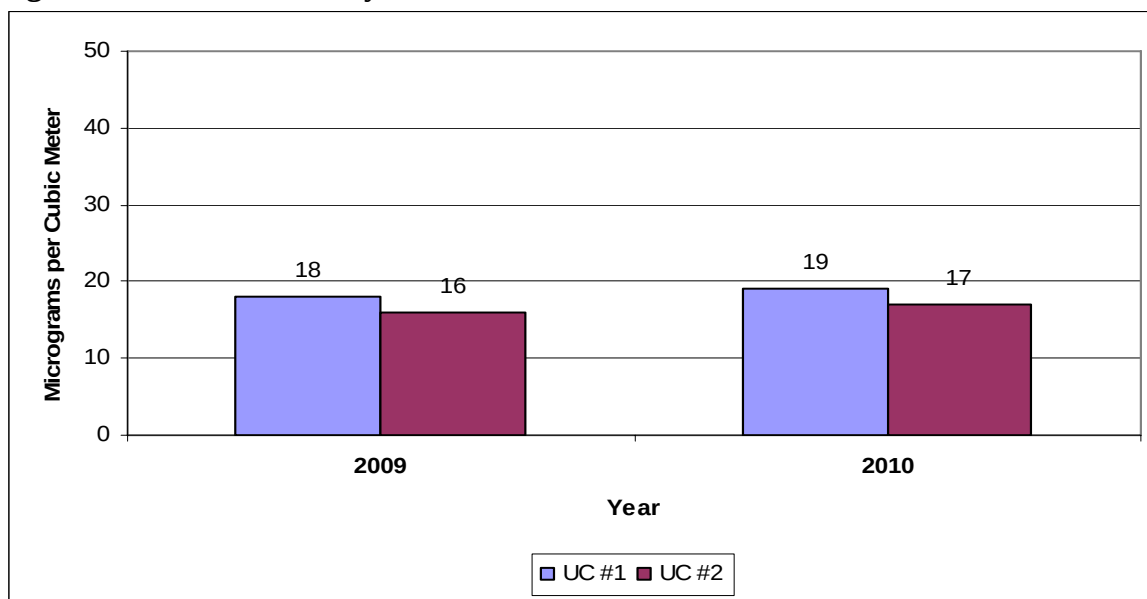
Figure 7-46 – Union County Annual PM 10 Concentrations
