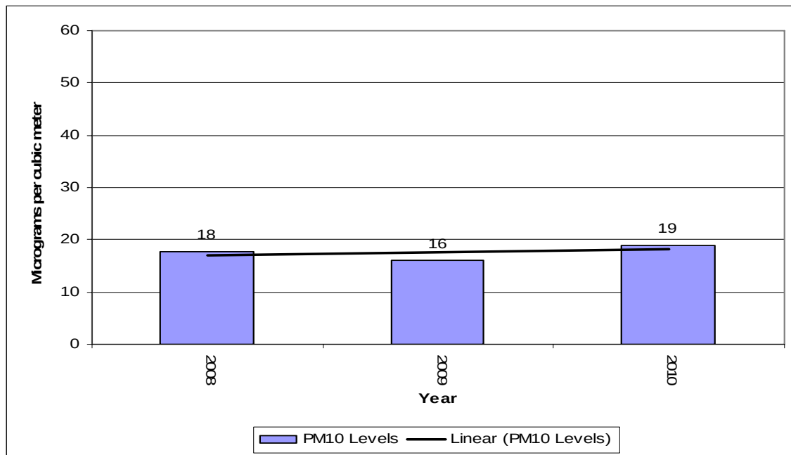
Figure 7-28 – SD School PM 10 Annual Averages
