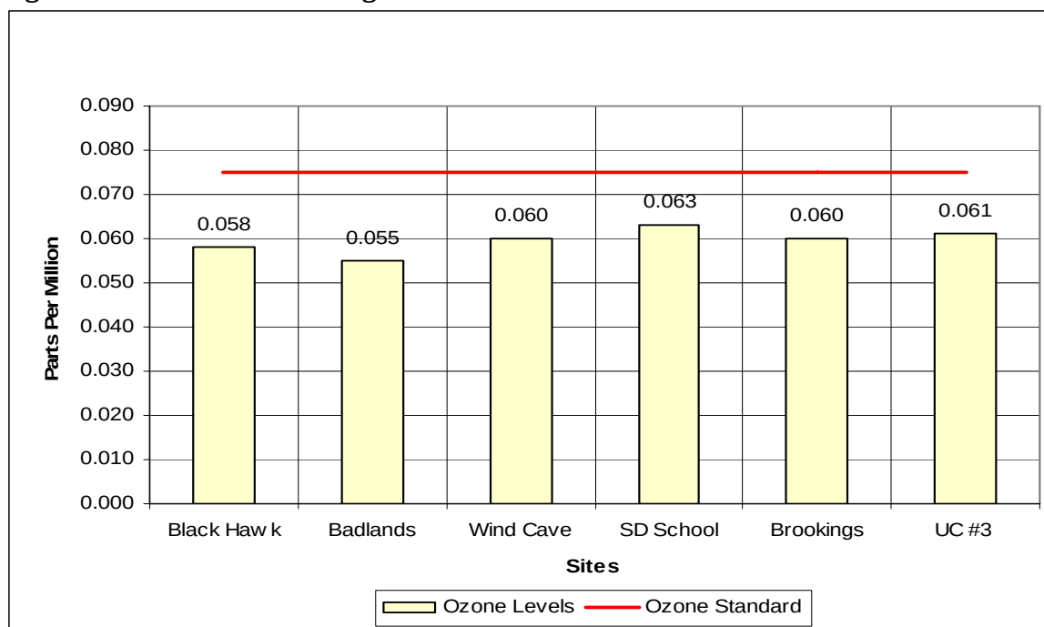
Figure 6-4 – 2010 Ozone Design Values Statewide 1
