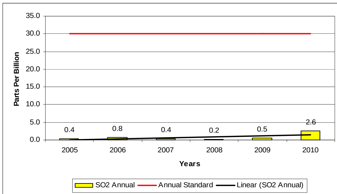
Figure 7-21 – Wind Cave Sulfur Dioxide Annual Averages
