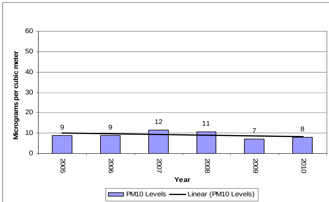
Figure 7-13 – Badlands PM 10 Annual Averages
