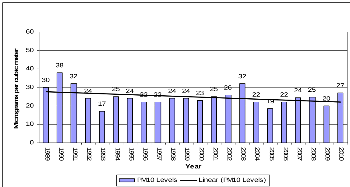
Figure 7-37 – City Hall Site PM 10 Annual Averages
