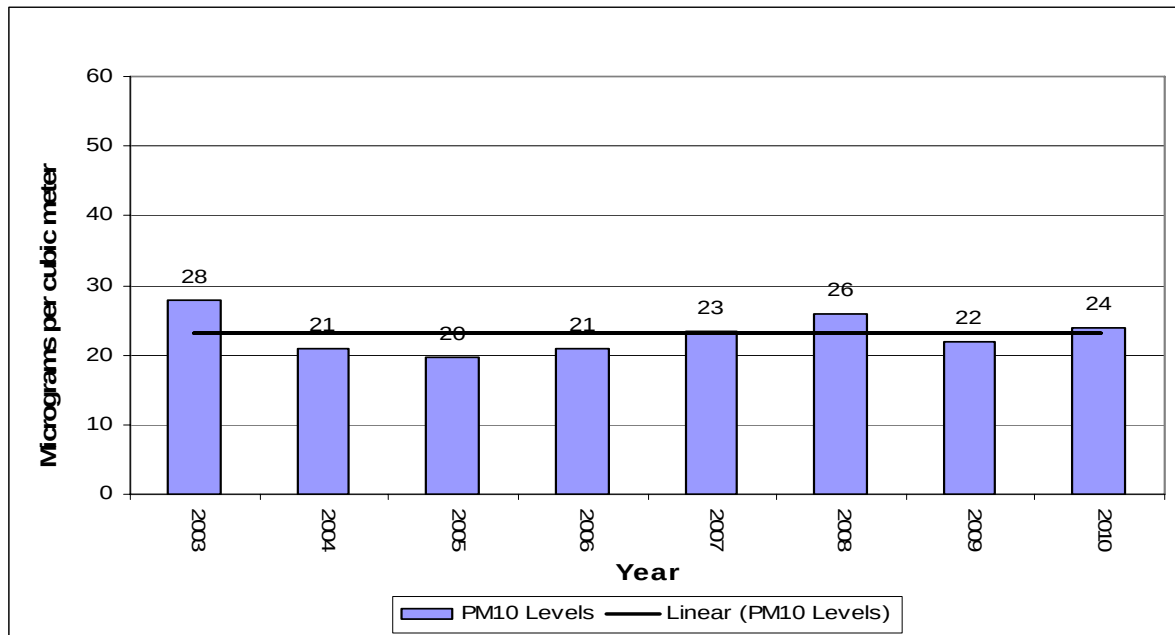
Figure 7-42 – Watertown PM 10 Annual Averages
