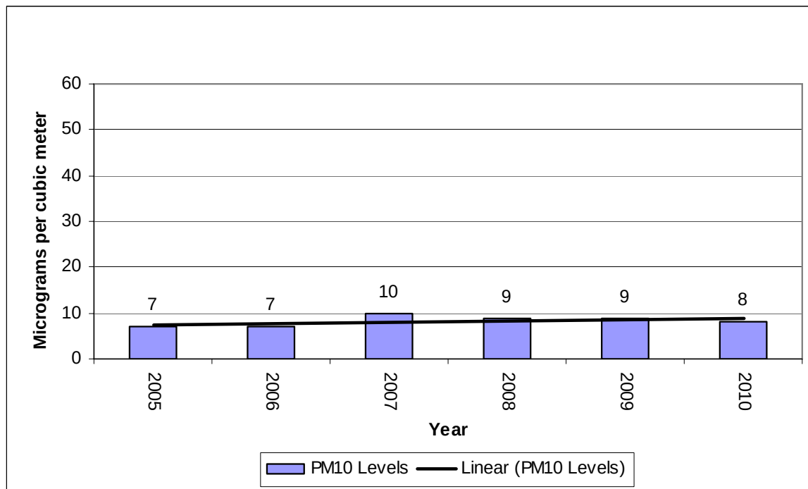
Figure 7-19 – Wind Cave PM 10 Annual Averages
