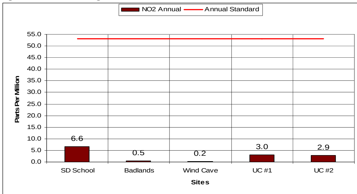
Figure 6-8 – 2010 Nitrogen Dioxide Annual Concentration
