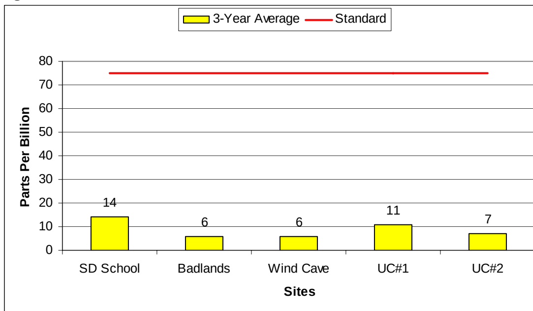
Figure 6-5 – 2010 Sulfur Dioxide 1-Hour Concentrations 1
