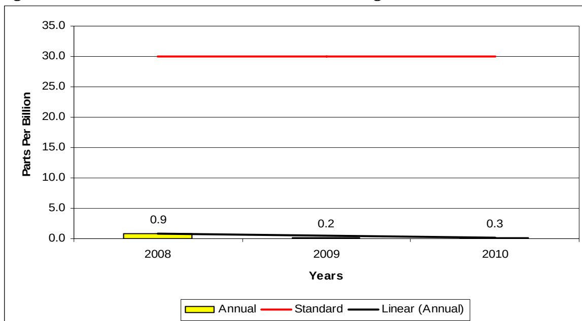
Figure 7-31 – SD School Sulfur Dioxide Annual Averages
