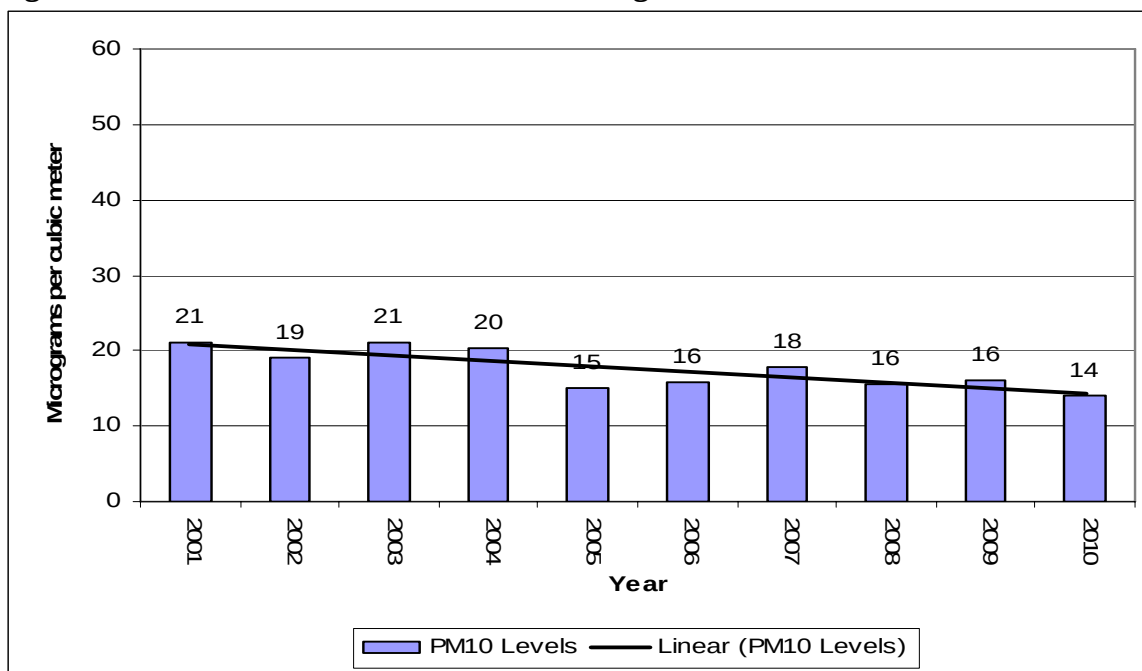
Figure 7-10 – Black Hawk PM 10 Annual Averages
