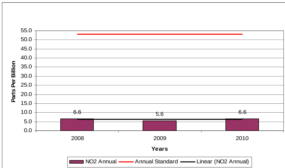
Figure 7-32 – SD School Nitrogen Dioxide Annual Averages
