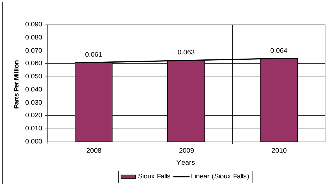
Figure 7-30 – SD School Ozone Yearly 4 th Highest 8-Hour Averages
