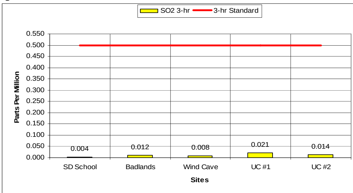
Figure 6-6 – 2010 Sulfur Dioxide 3-hour Concentrations 1
