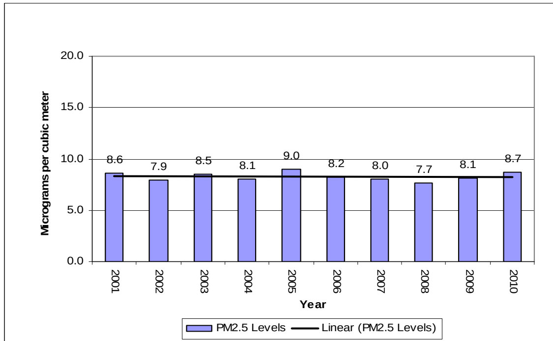
Figure 7-35 – Fire Station #1 PM 2.5 Annual Averages
