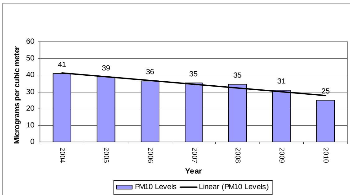
Figure 7-7 – RC Credit Union PM 10 Annual Averages
