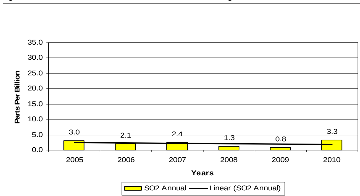
Figure 7-15 – Badlands Sulfur Dioxide Annual Averages
