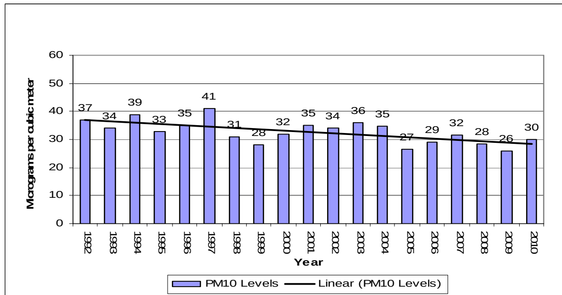
Figure 7-5 – RC National Guard PM 10 Annual Averages
