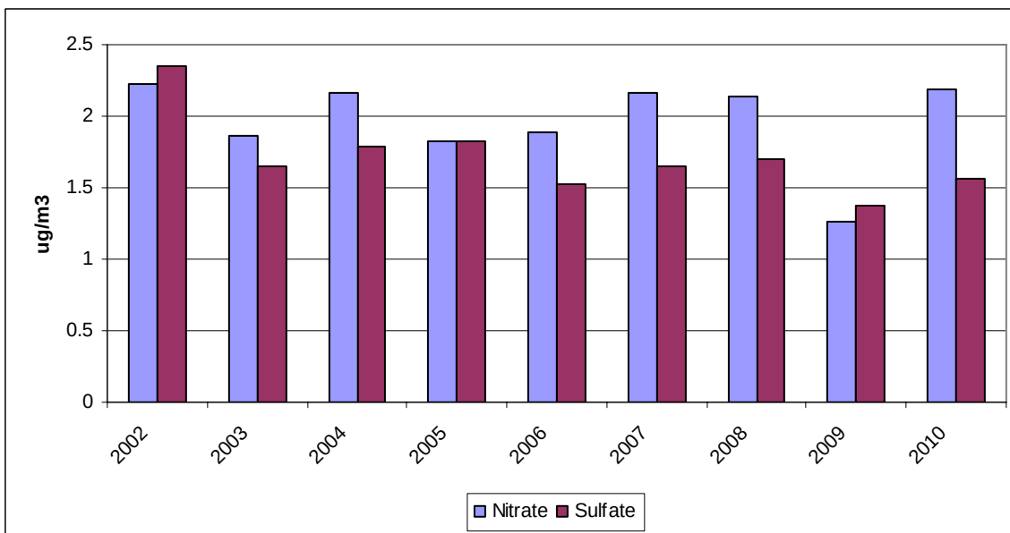
Figure 8-4 – Average Nitrate and Sulfate Concentrations
