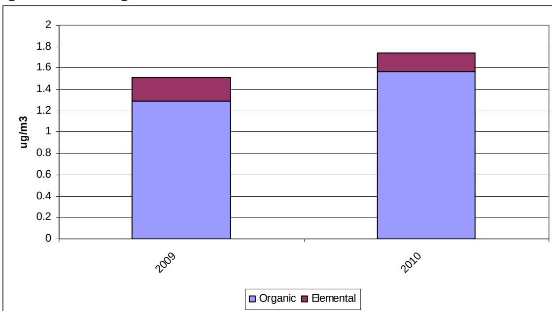
Figure 8-3 – Average Carbon Concentrations
