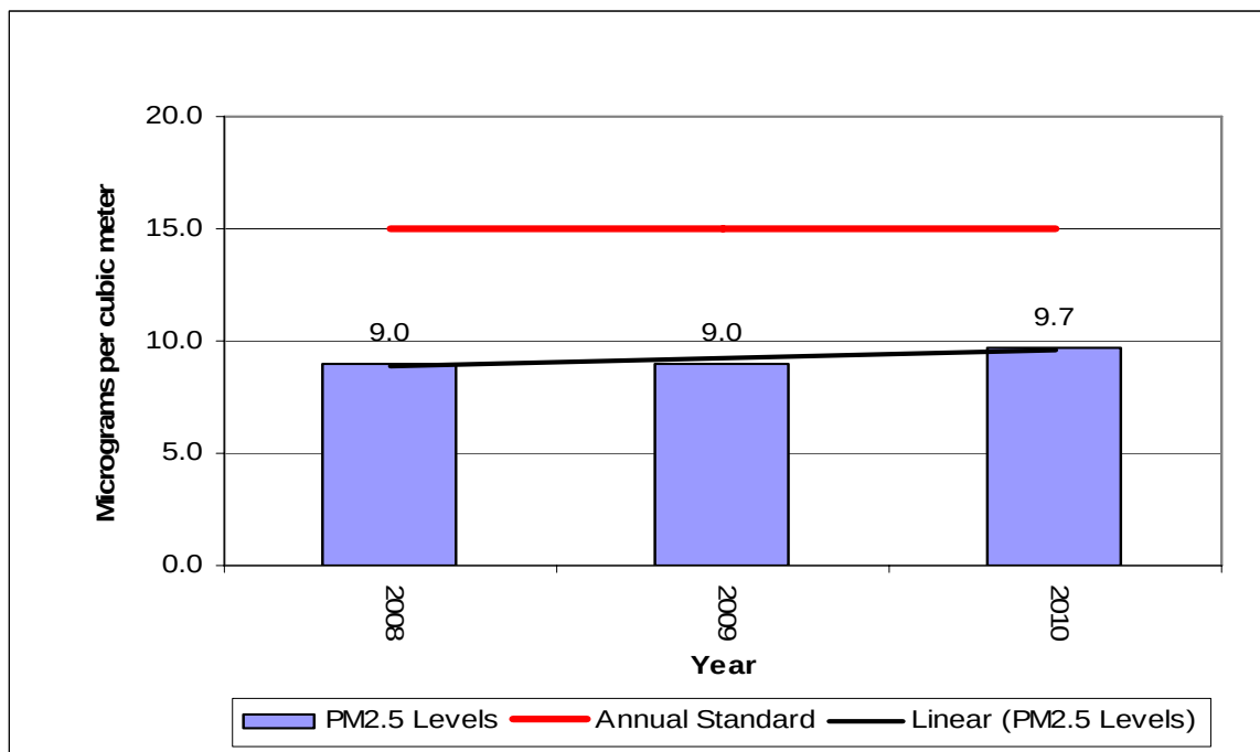
Figure 7-29 – SD School PM 2.5 Annual Averages
