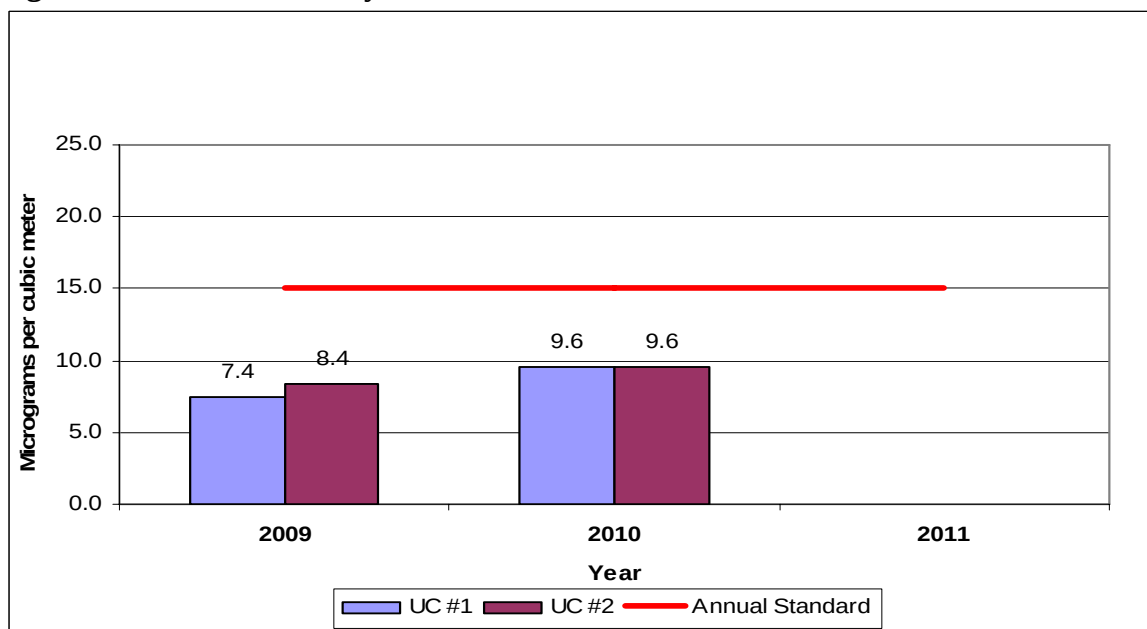
Figure 7-47 – Union County Annual PM 2.5 Concentrations
