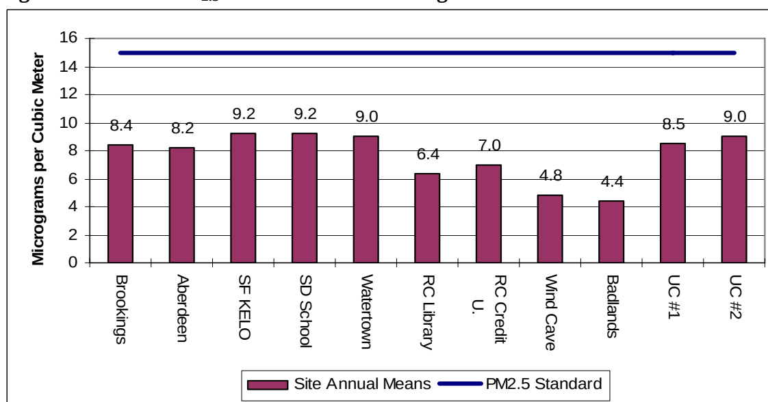
Figure 6-3 – 2010 PM 2.5 Statewide Annual Design Values 1
