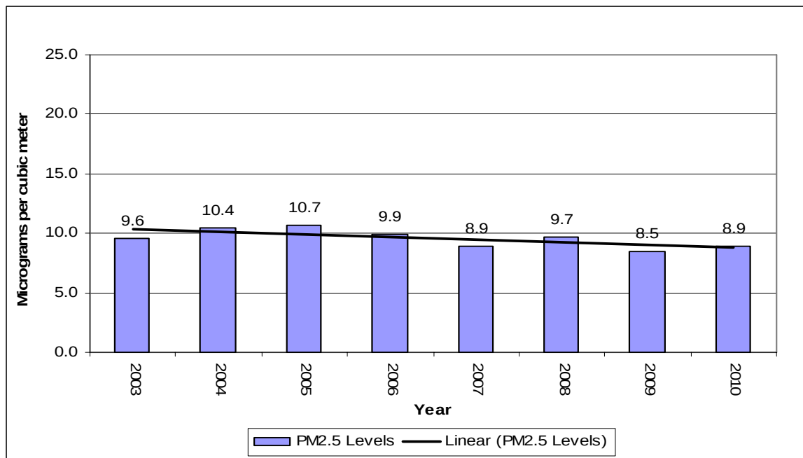
Figure 7-43 – Watertown PM 2.5 Annual Averages
