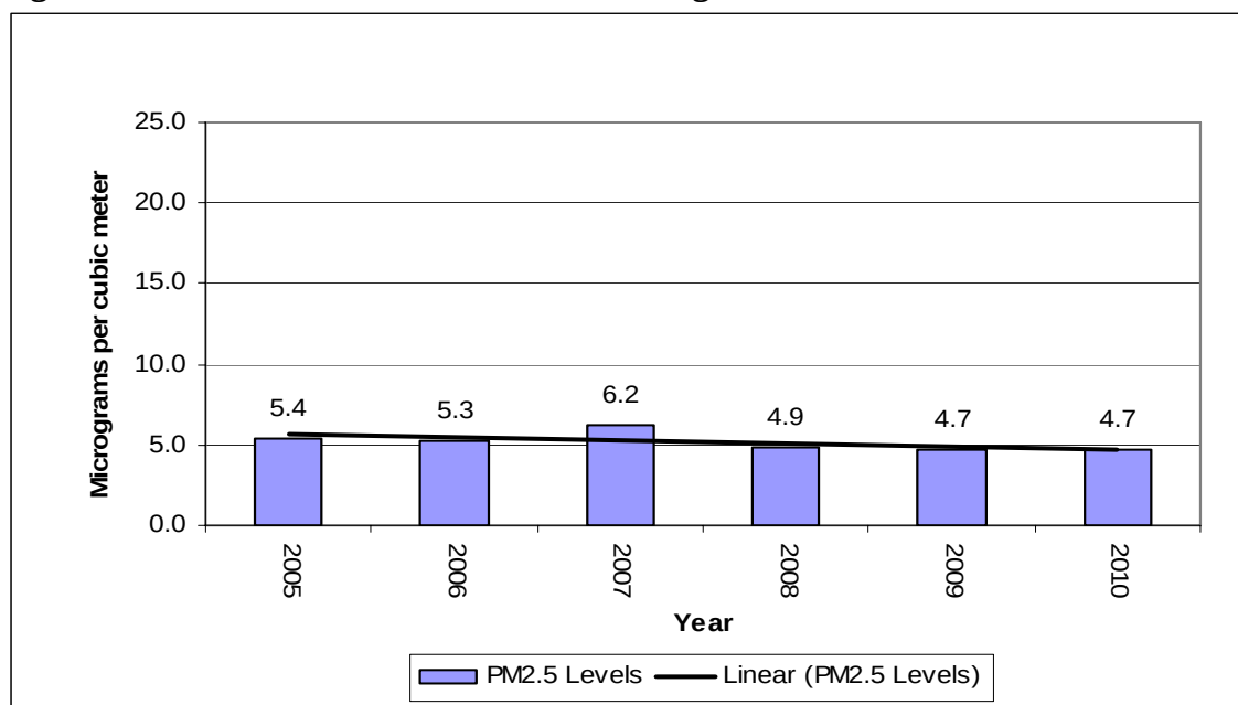
Figure 7-20 – Wind Cave PM 2.5 Annual Averages
