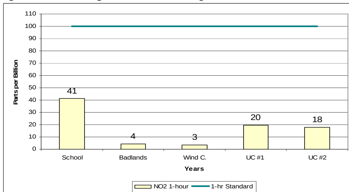
Figure 6-7 – 2010 Nitrogen Dioxide 1-hour Design Values 1
