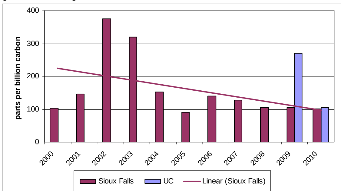
Figure 8-1 – Average Total NMOC 1
