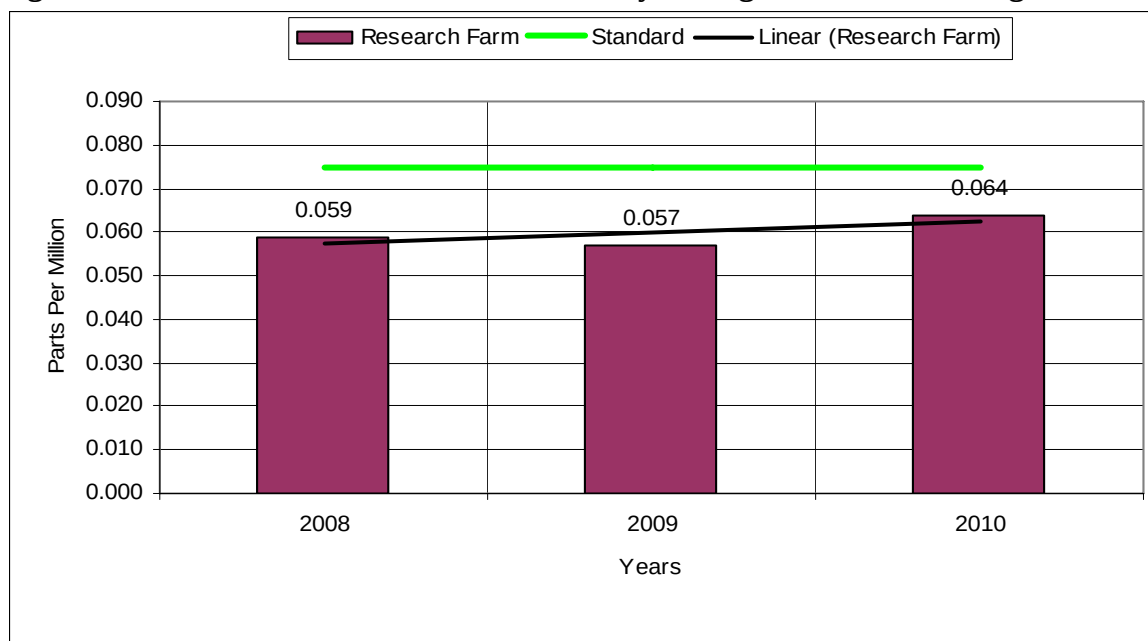
Figure 7-40 – Research Farm Site Ozone Yearly 4 th Highest 8-Hour Averages
