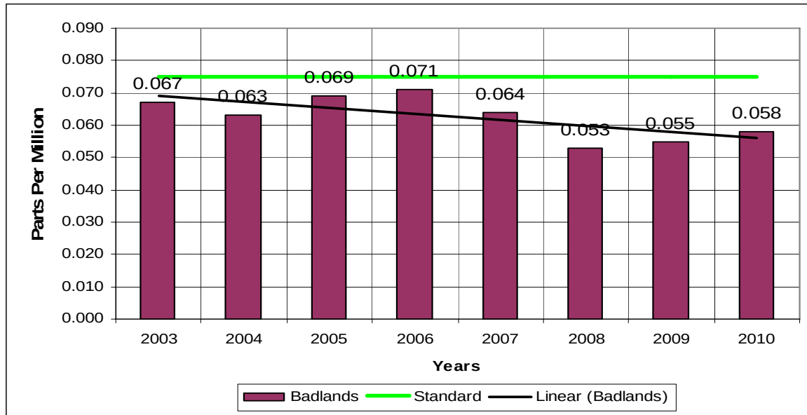
Figure 7-16 – Badlands Ozone Yearly 4 th Highest 8-hour Averages
