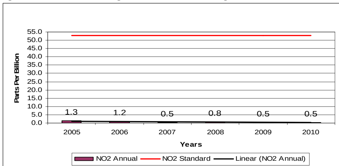
Figure 7-17 – Badlands Nitrogen Dioxide Annual Averages
