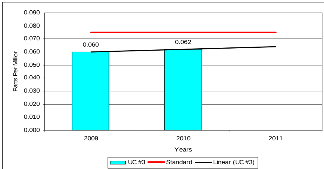
Figure 7-51 – Union County Ozone Concentrations
