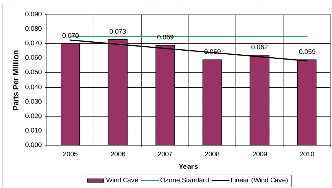
Figure 7-23 – Wind Cave Ozone Yearly 4 th Highest 8-hour Averages
