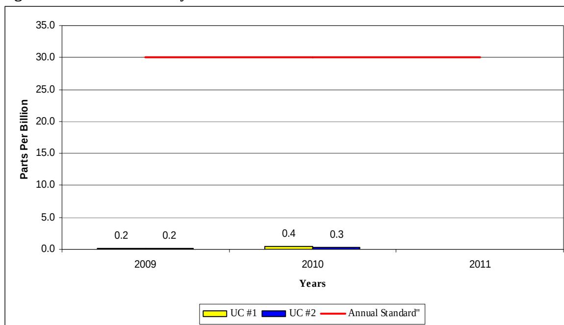
Figure 7-48 – Union County Sulfur Dioxide Concentrations
