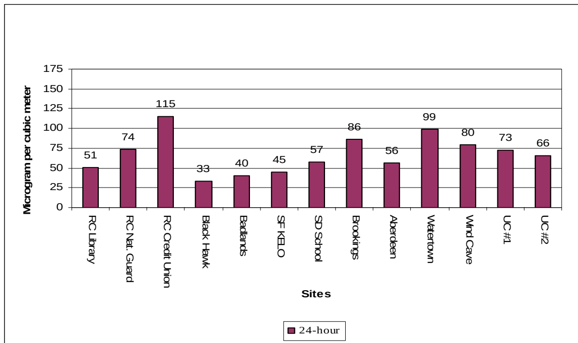
Figure 6-1 – 2010 PM 10 Design Values Statewide 1
