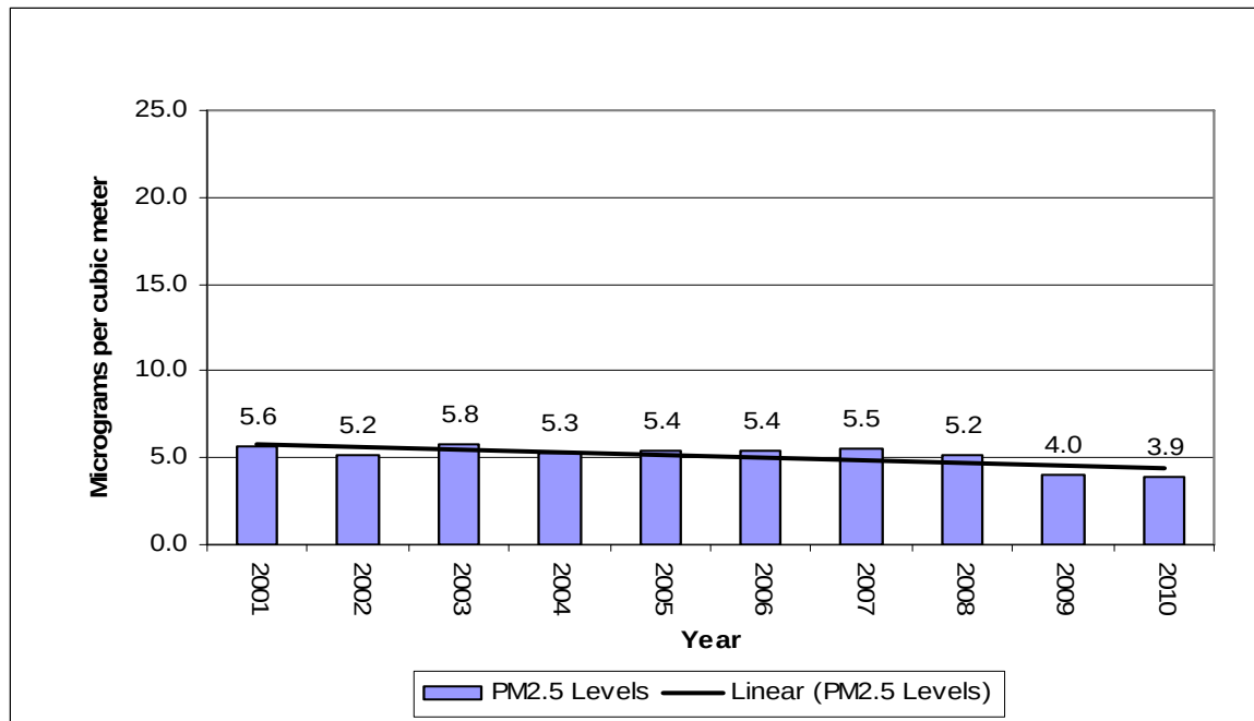
Figure 7-14 – Badlands PM 2.5 Annual Averages
