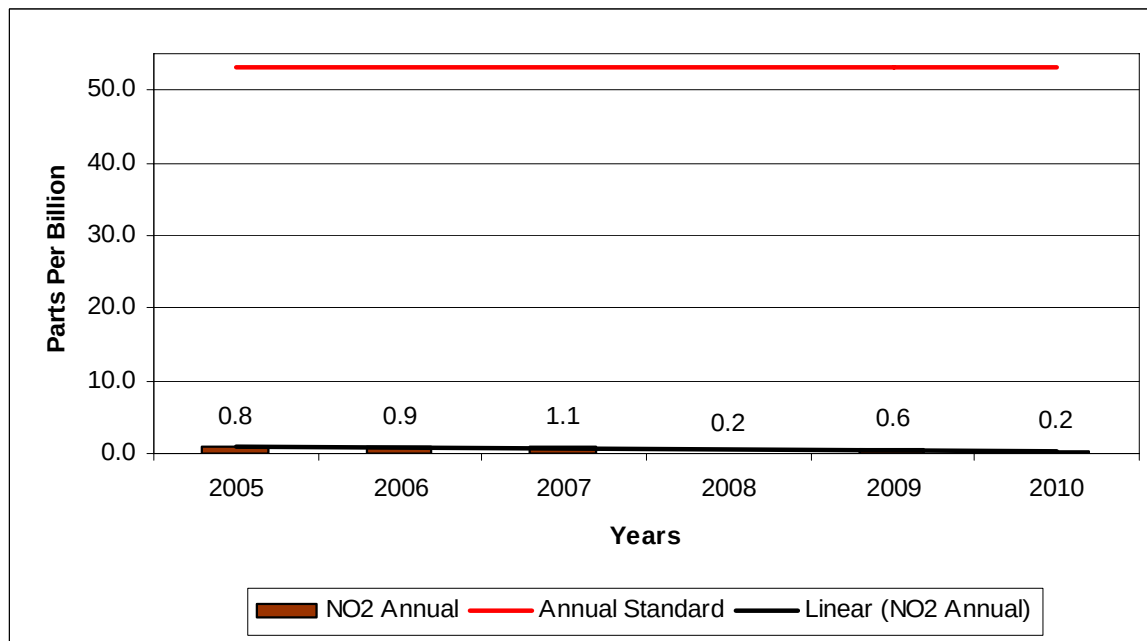
Figure 7-22 – Wind Cave NO 2 Annual Averages
