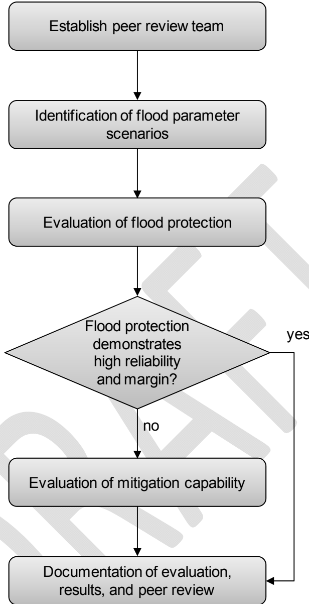
Figure 2: Evaluation flowchart
